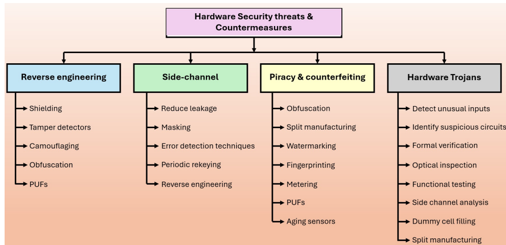
Figure 14. Hardware security threats and countermeasures [204,205].
