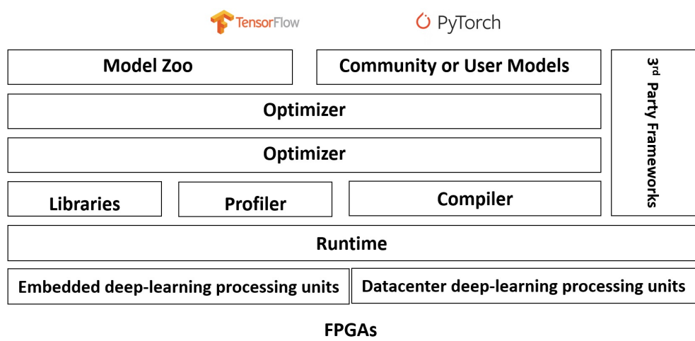
Figure 20. Xilinx Vitis™ AI Integrated Development Environment.
