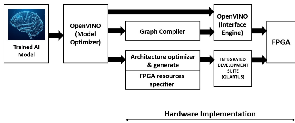
Figure 19. Edge-ready AI toolkits for Intel FPGAs [261].
