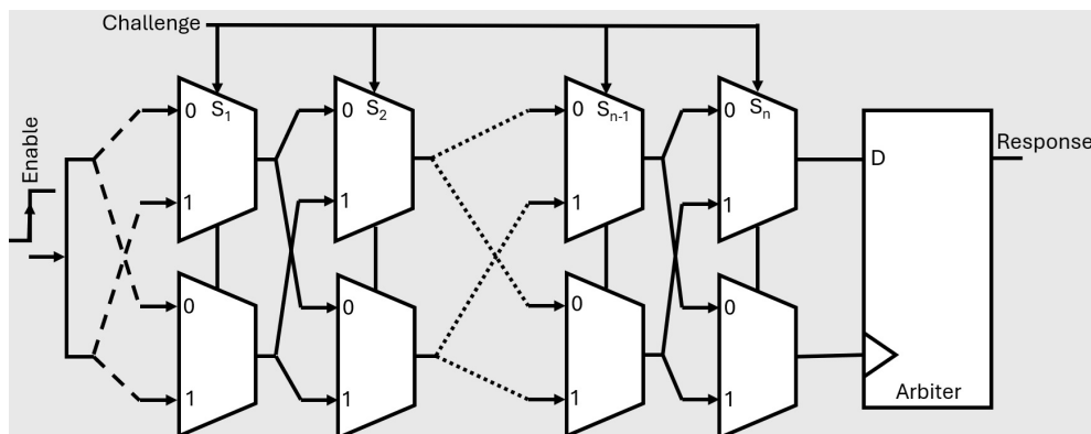
Figure 17. Structure diagram of n-stage APUF.
