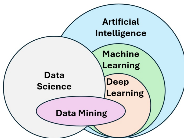
Figure 10. AI taxonomy.
