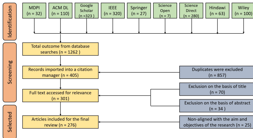
Figure 3. PRISMA chart.
