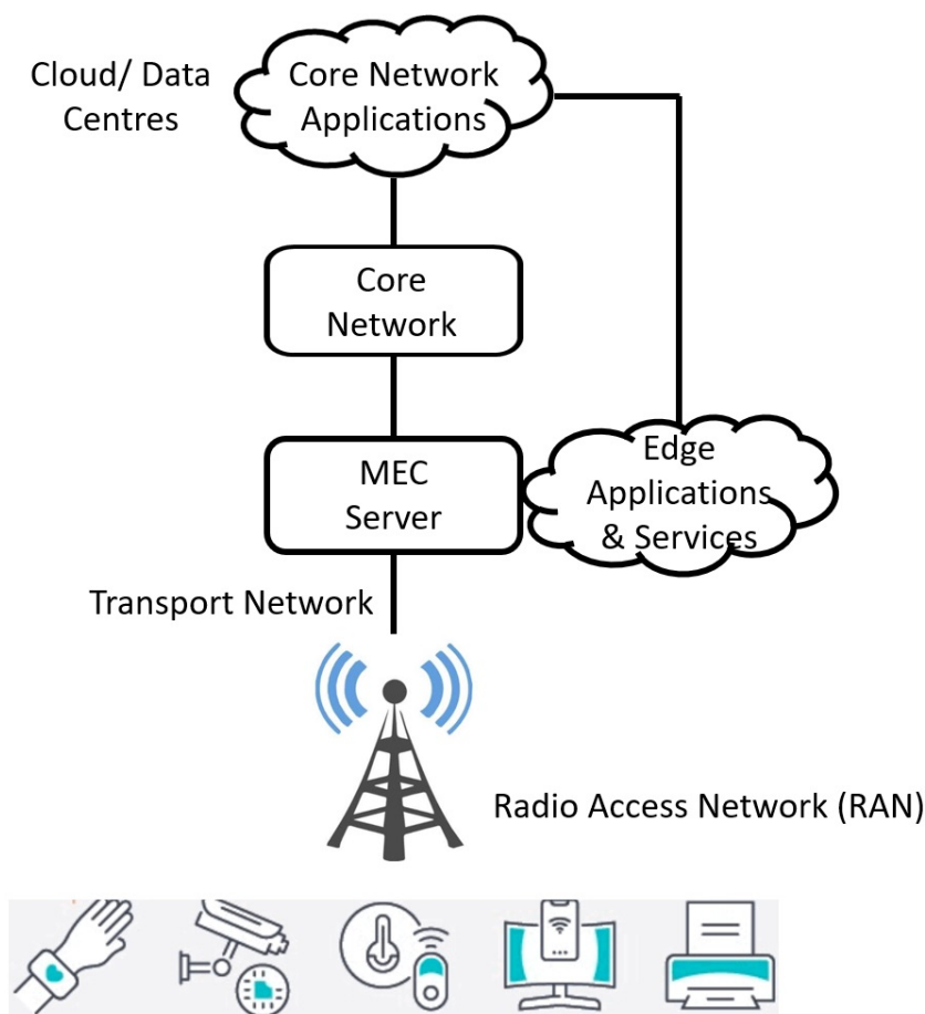
Figure 13. MEC architecture.
