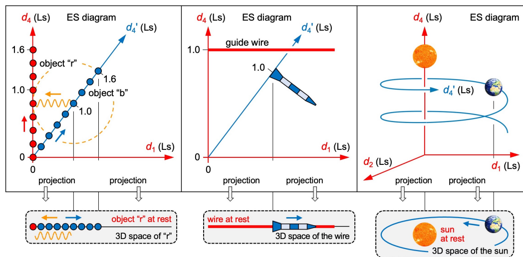
Fig. 5 Solving three problems in ER. Left: In ES, an energy taking a detour (blue and orange arrow) cannot collide with an energy moving straight (red arrow). In the 3D space of "r", it can. Center: In ES, the guide wire escapes from the rocket. In the 3D space of the wire, it does not. Right: In ES, the sun escapes from Earth's orbit. In the 3D space of the sun, it does not.
