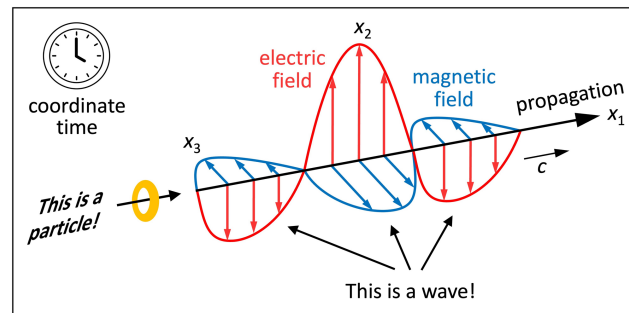
Fig. 8 Illustration of a wavematter. From an observer's perspective, it manifests itself as a particle or as a wave packet. As a wave packet (shown here), it propagates and oscillates as a function of his coordinate time. From its perspective (view through yellow pinhole), it is a particle at rest.
