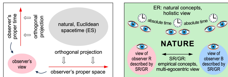
Fig. 1 Euclidean spacetime and observer's view. Left: How an observer's view is created from ES. Right: SR/GR and ER describe nature in different concepts.
