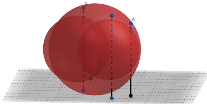
Figure 1. Visual representation, using three-dimensional spheres, of the fission of a hadron into two hadrons, with the creation of a pair of opposite colored charges. All the spheres are tangent to ordinary space. For clarity, the relativistic contraction of the radii of the spheres is not shown. The additional coordinate, perpendicular to spacetime, is only an aid in visualizing the intrinsic curvature of the positional constraint on strong charges and has no physical relevance in itself.
