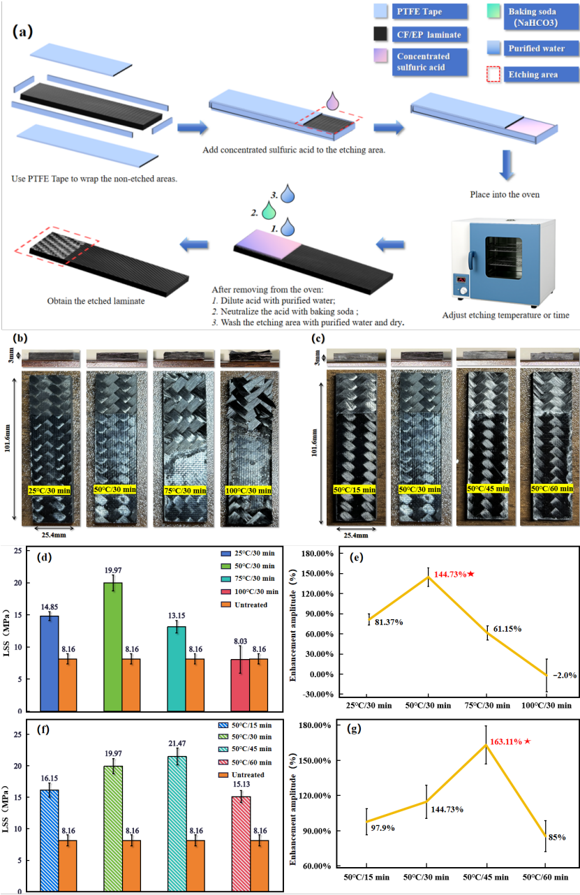
Figure 4. Acid-etching treatment of CF/EP laminates. (a)Acid-etching method. (b)Surface morphology of laminates for Temperature-variable groups. (c)Surface morphology of laminates for Time-variable groups. (d)LSS for Temperature-variable groups. (e)Percentage of increase in LSS for Temperature-variable groups. (f)LSS for Time-variable groups. (g)Percentage of increase in LSS for Time-variable groups.
