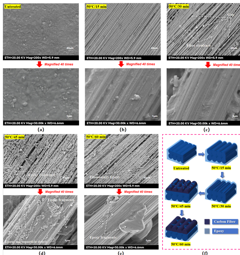
Figure 6. FE-SEM observation of Acid-etching effect (Time-variable experimental groups). (a) Untreated sample. (b) 50°C/15 min-treated sample. (c) 50°C/30 min-treated sample. (d) 50°C/45 min-treated sample. (e) 50°C/60 min-treated sample. and (f) Mechanism diagram of Acid-etching action.
