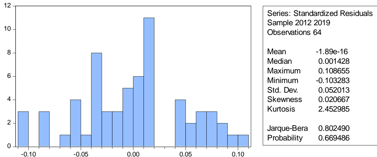
Figure 1: Normality test for residuals of LEV model
