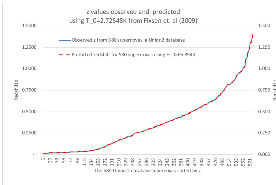
Figure 3. This figure shows observed redshift values from 580 type Ia supernovae, sorted by redshift (blue line). Based upon the measured CMB temperature by Fixsen et al (2009) of 2.72548K, the red line represents our predictions based on H_0 = 66.8943 \text{ km/s/Mpc} calculated from equation (10).
