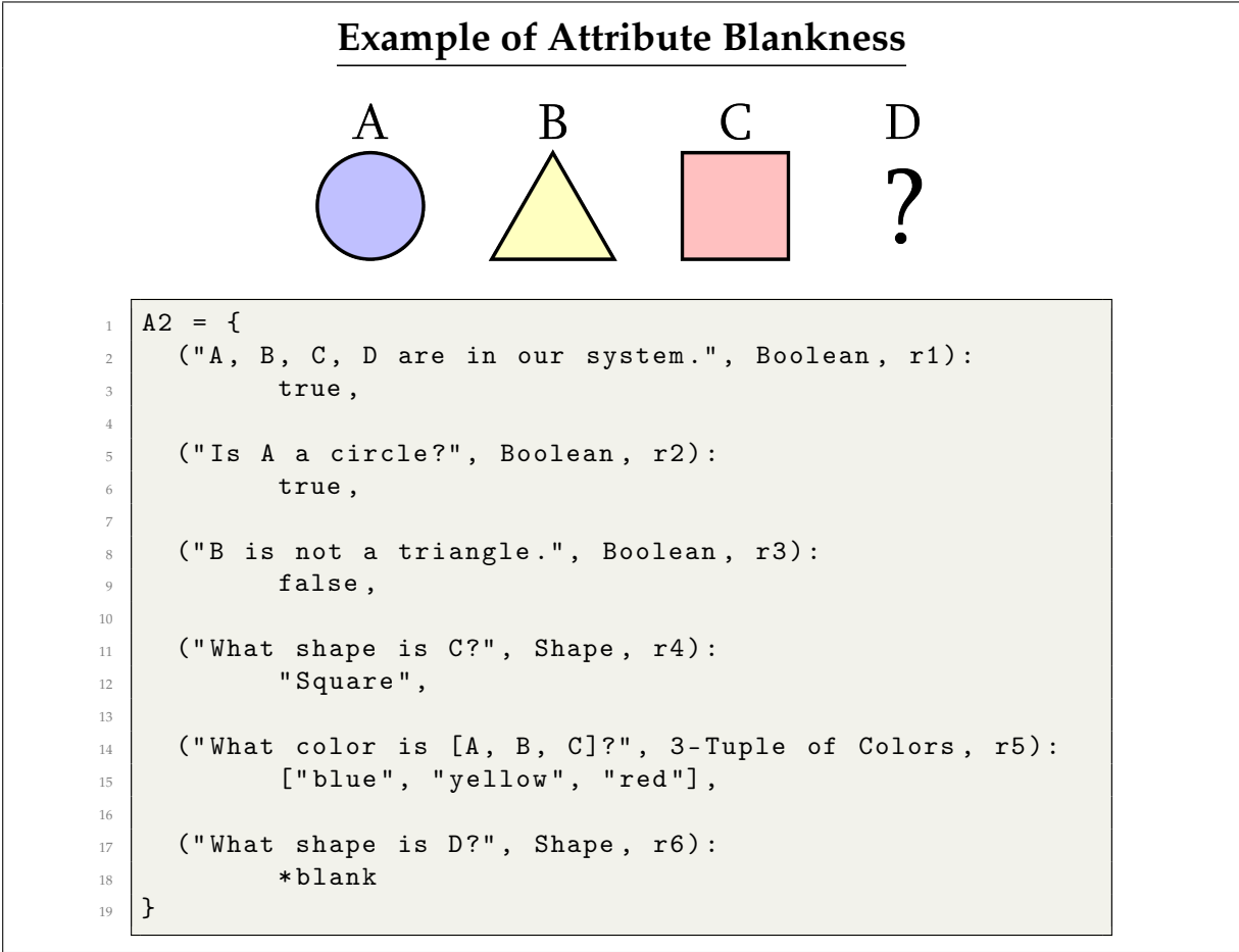
Figure 7. For this 2-Aethus, we have acknowledged the presence of an additional shape in the system as compared to what we analyzed earlier. However, we do not know which shape such an additional shape is, and as such are obliged to set the attribute encoding its shape to blank. [1]
