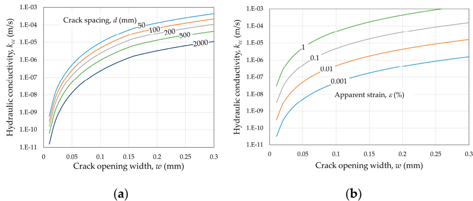
Figure 4. Values of the hydraulic conductivity of cracked concrete, k_{cc} (m/s), calculated using Equation (20) for w \leq 0.158 mm and Equation (21) for w \geq 0.158 mm as a function of the crack opening width, w : (a) for different crack spacings; (b) for different apparent strains.
