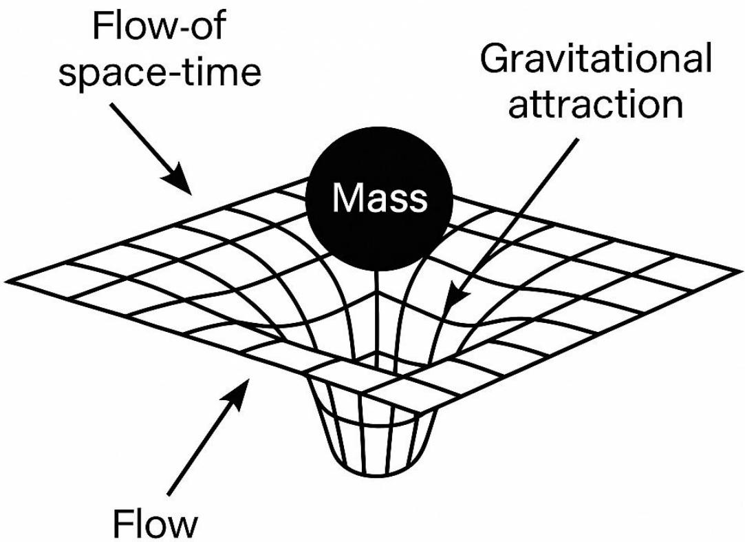
Figure 1. SPACETIME AS FLUID MEDIUM.
