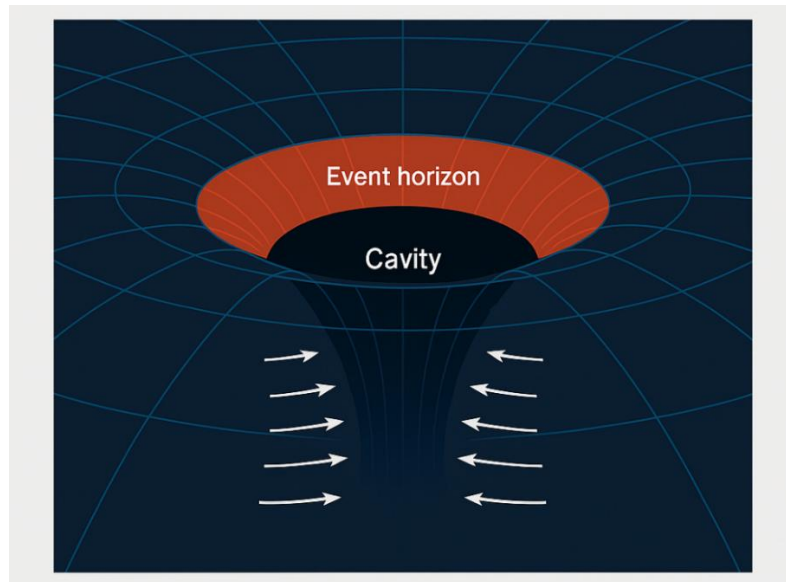
Figure 10. – CAVITATION RUPTURE AND EVENT HORIZON
