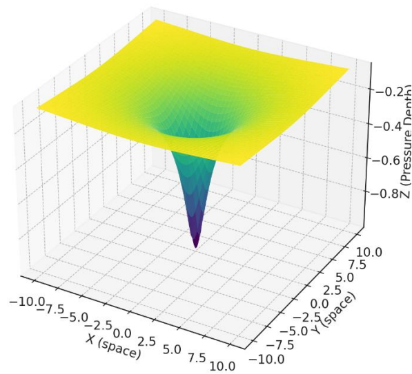
Figure 9. A – A 3D MODEL OF A SPACE-TIME GRAVITY WELL VISUALIZED AS A PRESSURE PIT IN AN INCOMPRESSIBLE FLUID.
