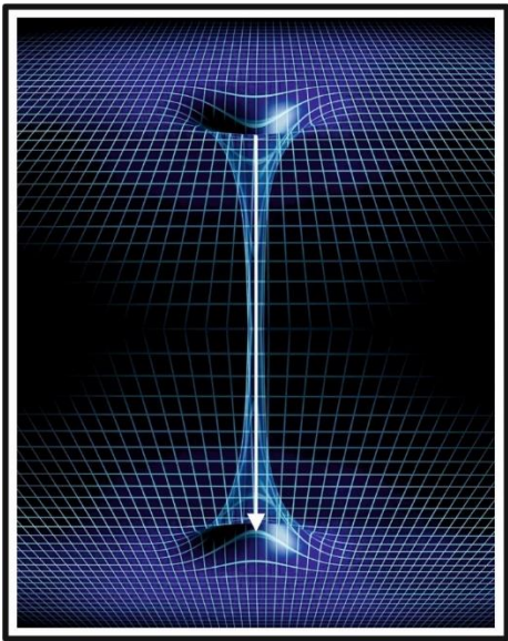
Figure 12. – Wormhole as pressure tunnel Caption: The wormhole forms as a stable fluid conduit between two cavities in the space-time fluid. The tunnel is held open by balanced internal and external pressures, not exotic matter.
