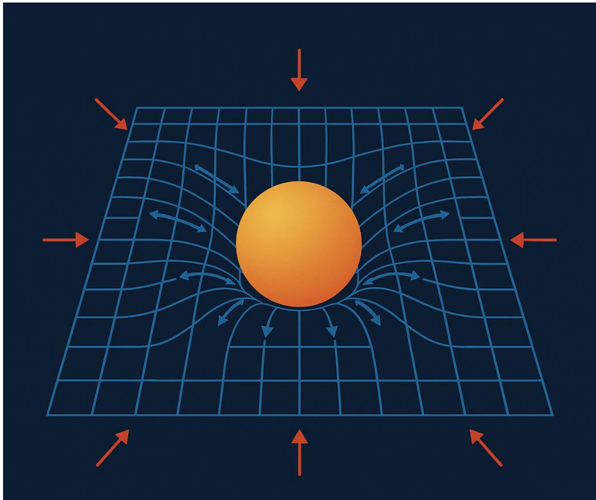
Figure 16. GRAVITY/MASS AND TENSION DISTRIBUTION.
