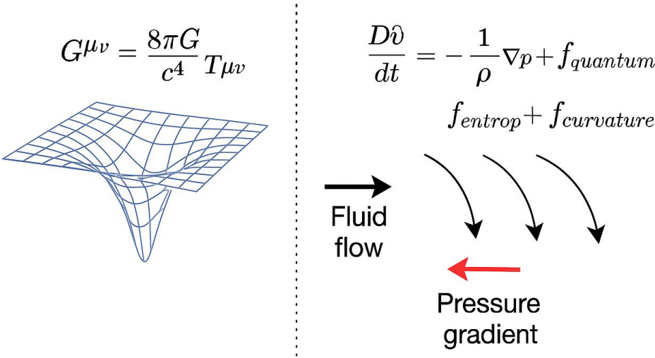
Figure 3. ANALOG BETWEEN EINSTEIN’S FIELD DYNAMICS AND FLUID DYNAMICS.
