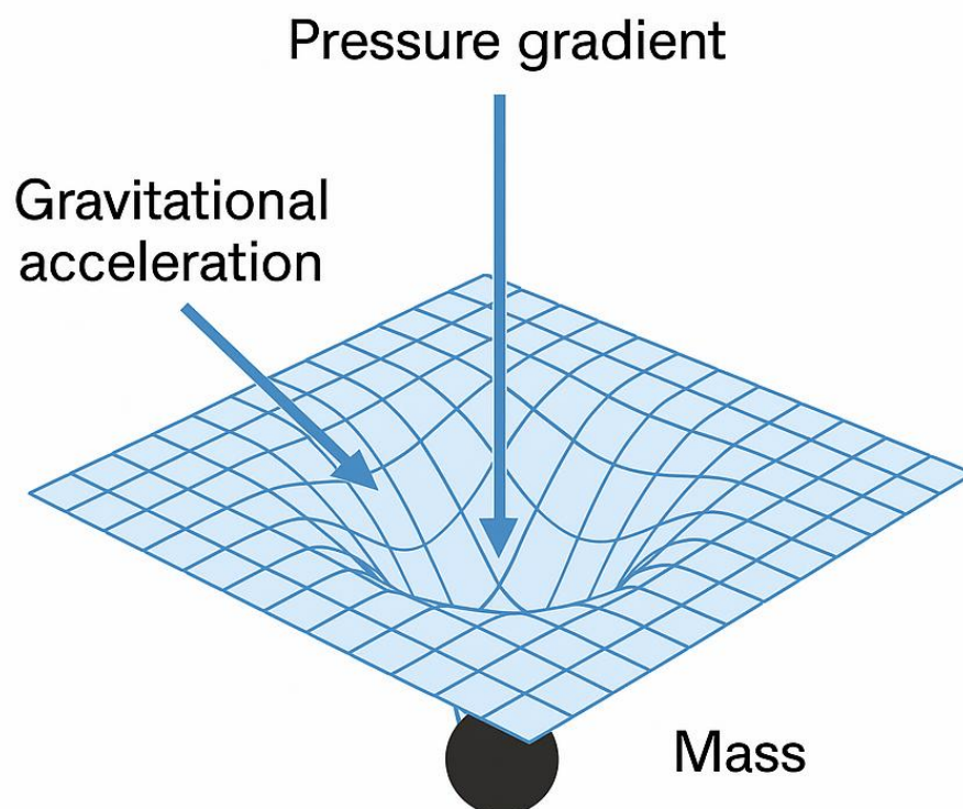
Figure 5. GRAVITY AS PRESSURE IMBALANCE IN SPACETIME FLUID.
