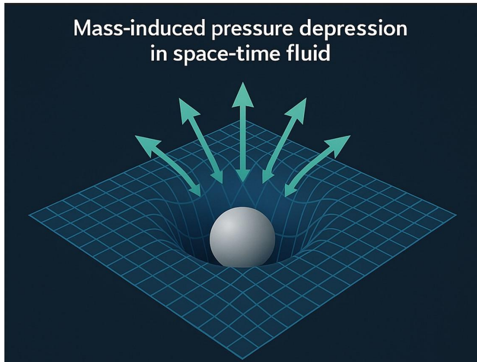
Figure 7. MASS-INDUCED PRESSURE DEPRESSION IN SPACE-TIME FLUID.
