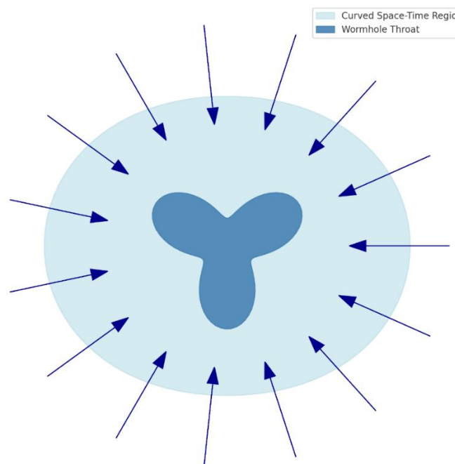
Figure 11. – WORMHOLE THROAT AND PRESSURE CURVATURE.
