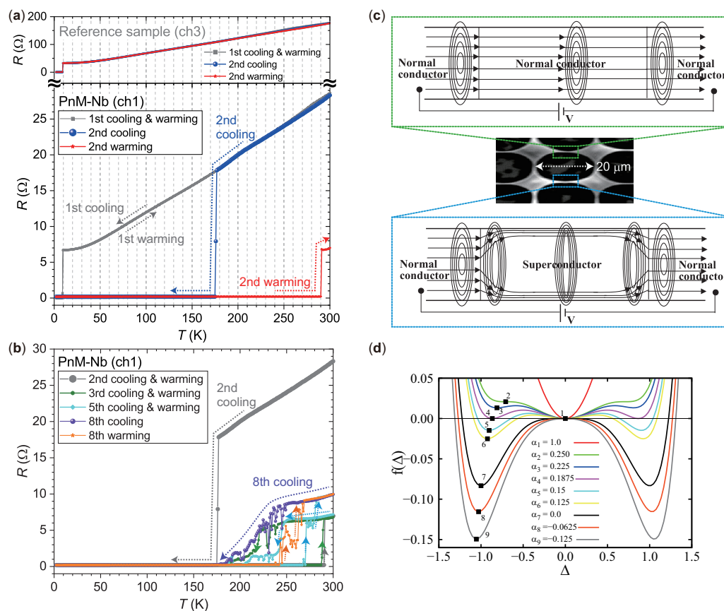
Figure 4. R - T results and possible involvement of magnetic flux for the first order phase transition. (a) Electrical resistance versus temperature of a reference Nb sample (upper panel) and that of a PnM-Nb sample (bottom panel) using the two-probe method, in the absence of an externally applied magnetic field. They were measured at the same time in the PPMS under the same condition. Only R - T results for the first and second cycles are shown. (b) R - T results of the PnM-Nb sample for all the rest of eight cycles. (c) Possible involvement of magnetic flux in the superconducting transition for an Nb holey sheet, based on the theory of hole superconductivity . Center panel, a portion of an SEM image of the Nb holey sheet; a void with the diameter of approximately 20 μm is surrounded by four narrow bridges. Upper and lower panel, a schematic normal bridge and a superconducting one with current streamlines and magnetic field lines (circles), respectively, from Ref. [14]. Even in the absence of an externally applied magnetic field, a self field generated by an excitation current for measuring resistance is expelled from a bridge becoming superconducting. As the dynamics of magnetic flux is involved in the superconducting transition, it can be a first order phase transition. This effect is significant for a system wherein magnetic orientation of the expelled flux is not to be averaged out. For details, read text. (d) Reason why warming is always beneficial to the zero-resistance state presented in this study, based on the Ginzburg-Landau theory: the key feature of a first-order phase transition. Free energy density as a function of the order parameter, for various temperatures, is dictated by differing choices of \alpha , as indicated in the legend, from Ref. [18]. The highest temperature is for \alpha_1 = 1 and progresses downwards towards \alpha_9 = -0.125 . Note that hysteresis may arise because, on lowering the temperature from \alpha_4 to \alpha_5 the system may choose to remain in the \Delta = 0 state. Only when the temperature is lowered to \alpha_7 (when \Delta = 0 is no longer a local minimum), does the system have to transition to a state with non-zero \Delta (we show the negative solutions only as square points for clarity), at which point the resistance would drop to zero. Upon increasing the temperature, a similar phenomenon may occur, whereby the non-zero \Delta state remains, until finally \alpha_2 is reached, and then a transition has to occur to the \Delta = 0 state with finite resistance.
