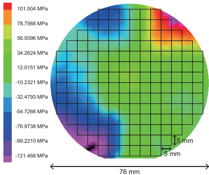
Figure 9. In-plane stress of an Nb layer sputtered on an SiO 2 /Si wafer with the diameter of 76 mm. The size of a sample chip (5×5 mm 2 ) is also indicated. The in-plane stress was measured using FSM 128NT (Frontier Semiconductor).
