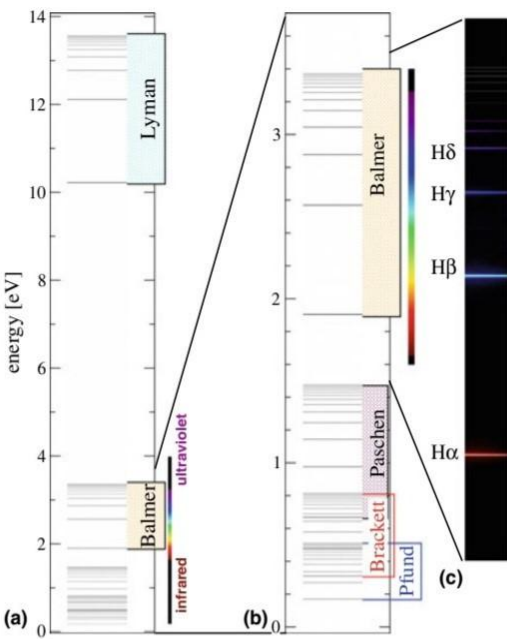
Figure 2. The observed emission line spectrum of atomic hydrogen in chapter 2 atoms.[5] (Manini, 2020).
