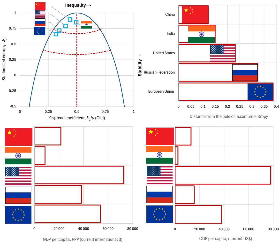
Figure 10. Characteristic graphs for the examined five major geopolitical players in 2022 (clockwise from upper left): standardized entropy vs. K-spread coefficient (Gini index), plotted alongside the maximum entropy vs. K-spread curve; distance from the pole of maximum entropy; GDP per capita [22]; GDP-PPP per capita, [23].
