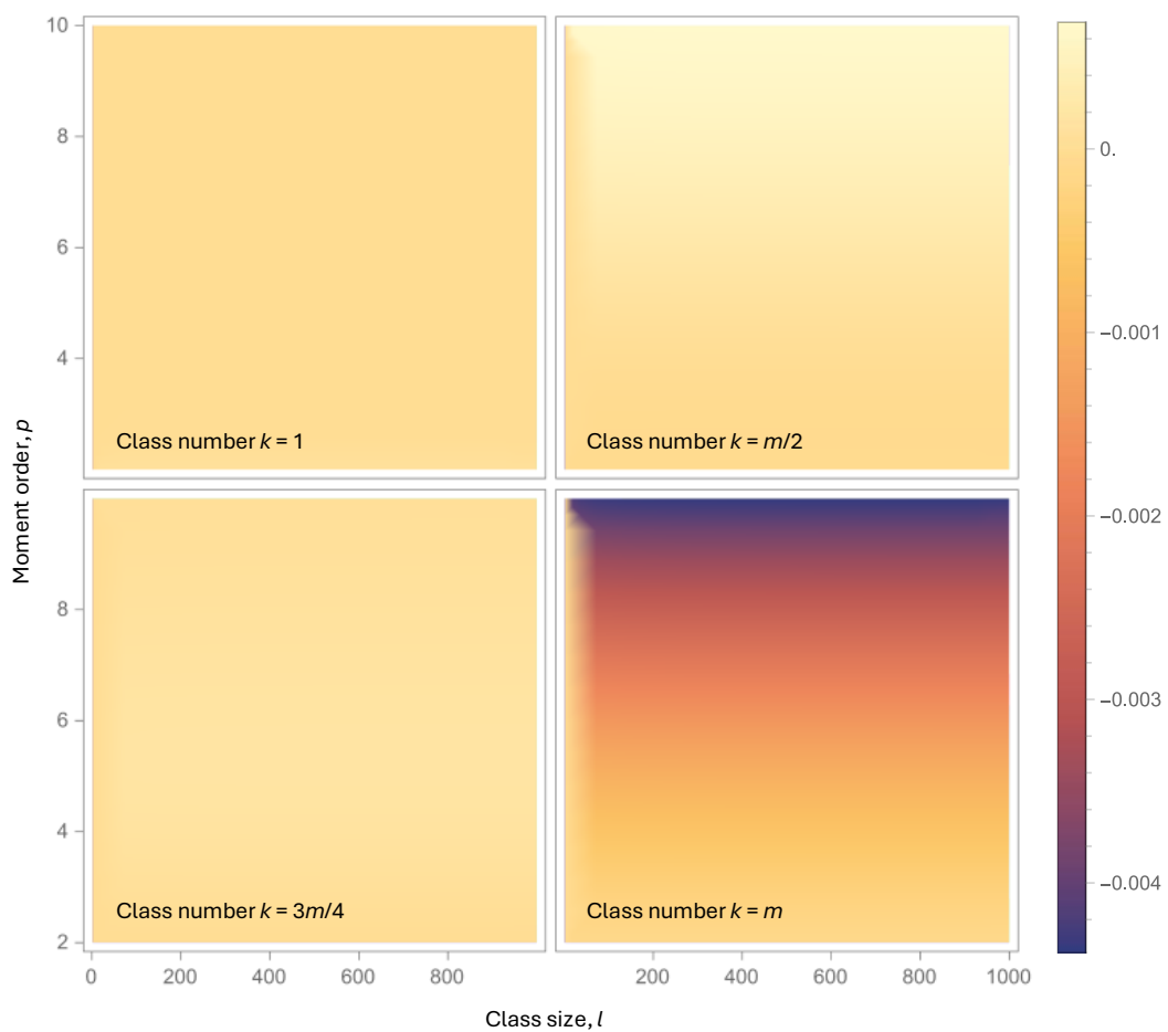
Figure A1. Density plots of the error D_{l,k,m,p} for a number of classes m = 100 and varying moment order p and class size, l , and for the indicates class numbers, k .
