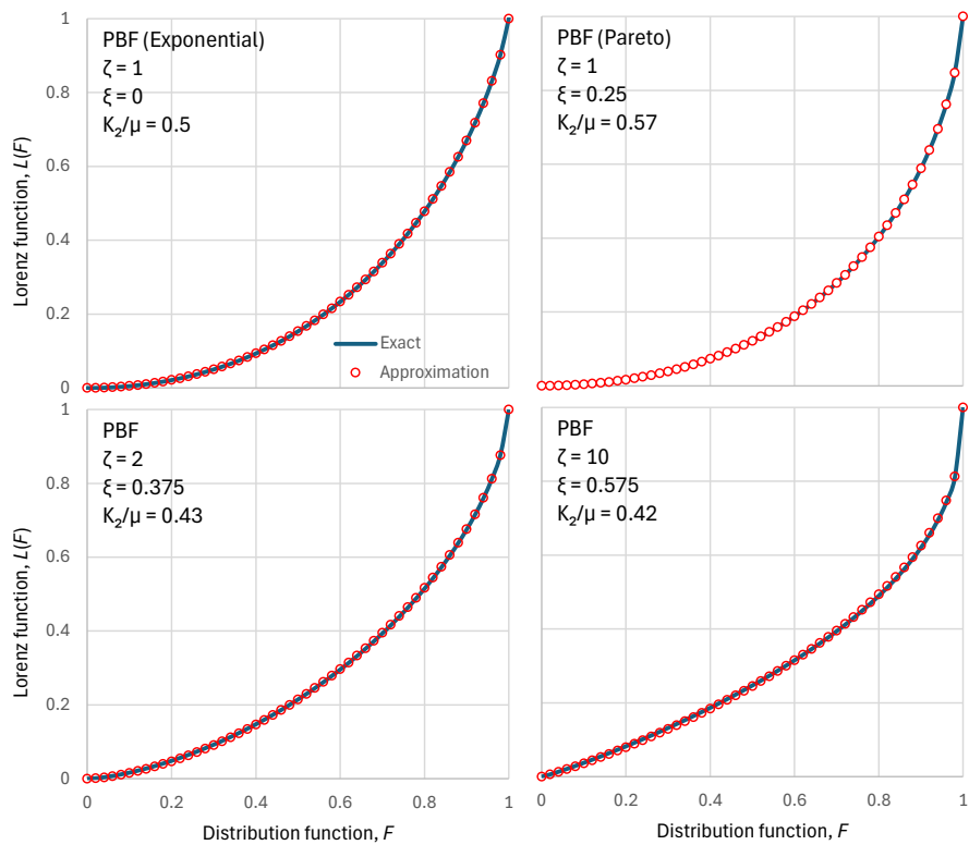
Figure 1. Visual comparison of the exact Lorenz curves for the PBF distribution function with four different parameters sets (shown in each of the four panels) with the approximation of Equation (30). Except for the Pareto case, the \xi parameter was determined so as to maximize entropy for a chosen \zeta parameter.
