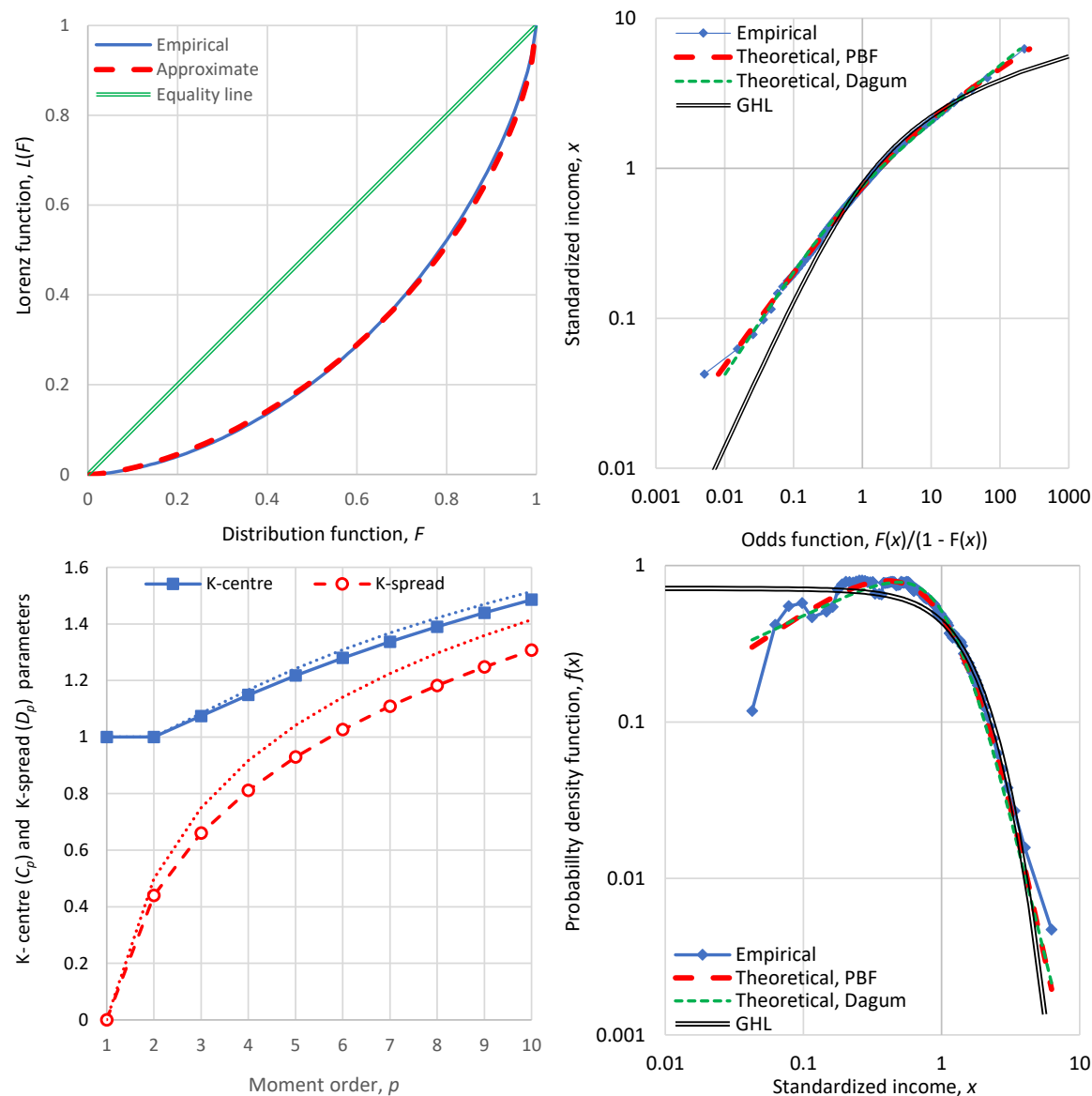
Figure 9. Detailed graphs of economic indicators of China in 2022 ( clockwise from upper left ): Lorenz curve; odds function; probability density function; and graph of K-centre and K-spread vs. K-moment order, where for reference the theoretical curves of the ME exponential distribution are also plotted in dotted lines.
