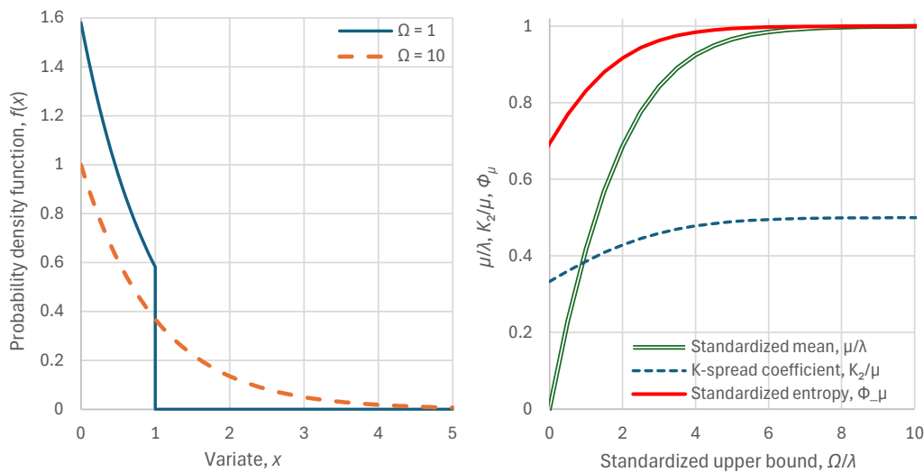
Figure 5. Visualization of the behaviour of the bounded exponential distribution, resulting from maximization of entropy for fixed mean \mu and upper bound \Omega : (left) two instances of the probability density function for the indicated values of the upper bound and for scale parameter \lambda = 1 ; (right) variation of standardized mean, K-spread coefficient (Gini index) and standardized entropy, for varying upper bound \Omega/\lambda .
