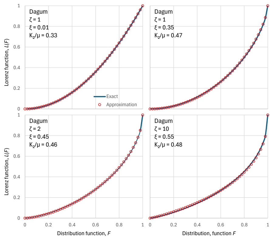
Figure 2. Visual comparison of the exact Lorenz curves for the Dagum distribution function with four different parameters sets (shown in each of the four panels) with the approximation of Equation (30). Except for the upper-left case, the \xi parameter was determined so as to maximize entropy for a chosen \zeta parameter.
