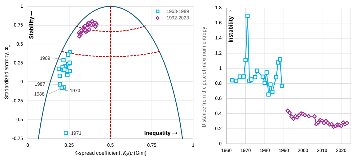
Figure 17 Characteristic graphs for the evolution of major economic indices in Bulgaria: (left) : standardized entropy vs. K-spread coefficient (Gini index), plotted alongside the maximum entropy vs. K-spread curve; (right) distance from the pole of maximum entropy. The cyan rectangles represent the era of Soviet influence and the purple diamonds the era of free market.
