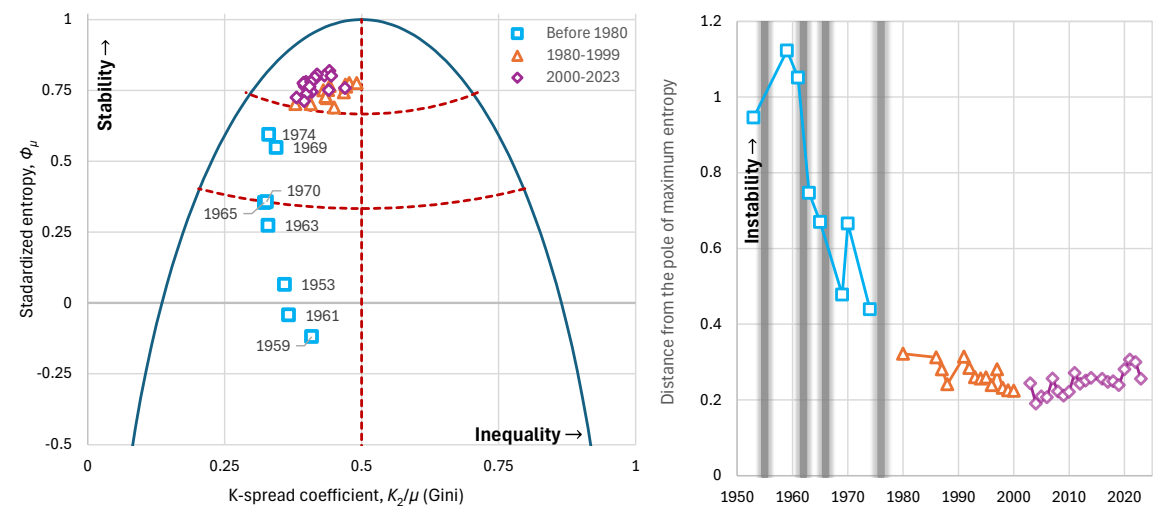
Figure 12. Characteristic graphs for the evolution of major economic indices in Argentina: (left): standardized entropy vs. K-spread coefficient (Gini index), plotted alongside the maximum entropy vs. K-spread curve; (right) distance from the pole of maximum entropy with the grey lines indicating the times of coups d'état.
