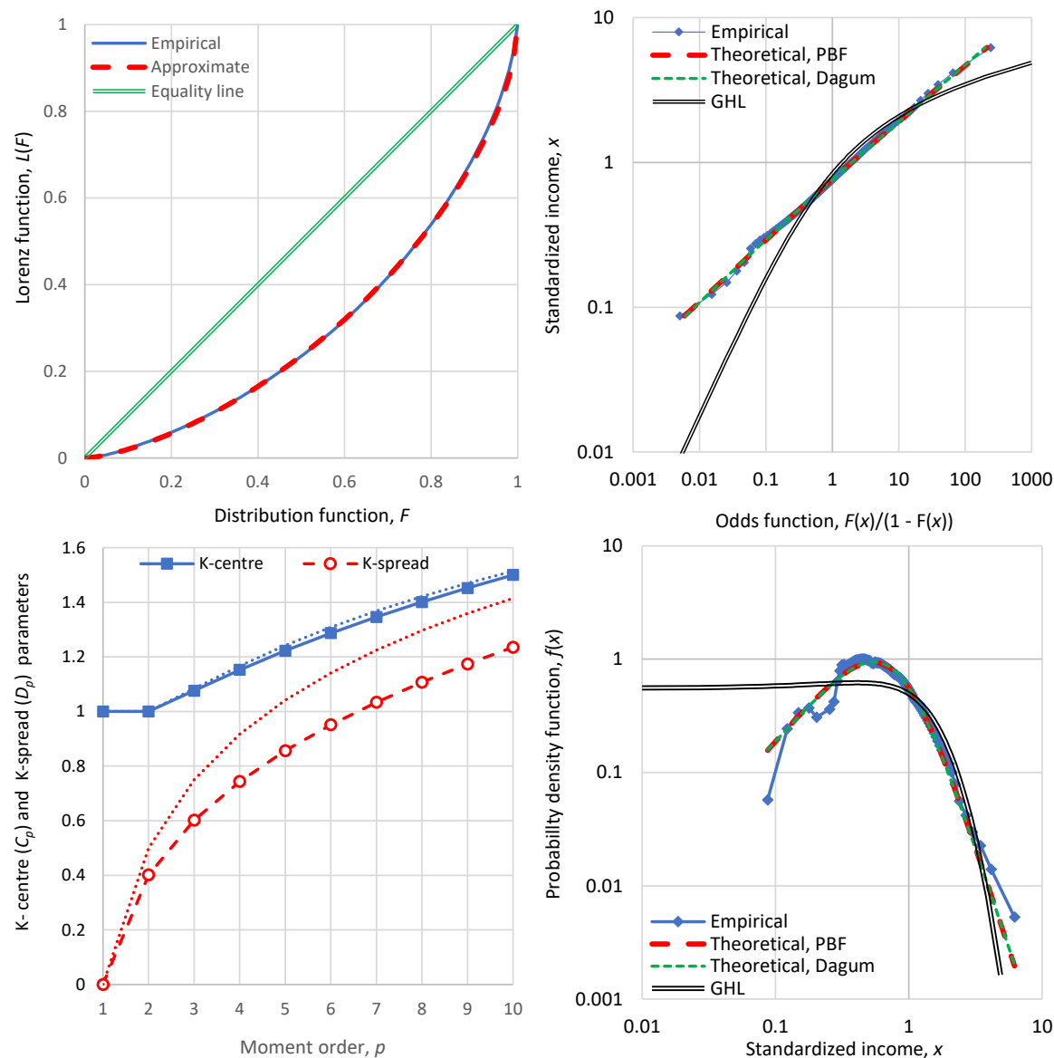
Figure 8. Detailed graphs of economic indicators of USA in 2022 ( clockwise from upper left ): Lorenz curve; odds function; probability density function; and graph of K-centre and K-spread vs. K-moment order, where for reference the theoretical curves of the ME exponential distribution are also plotted in dotted lines.
