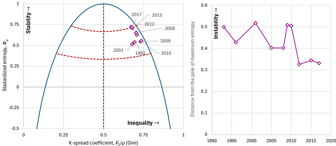
Figure 15 Characteristic graphs for the evolution of major economic indices in South Africa: (left) : standardized entropy vs. K-spread coefficient (Gini index), plotted alongside the maximum entropy vs. K-spread curve; (right) distance from the pole of maximum entropy.
