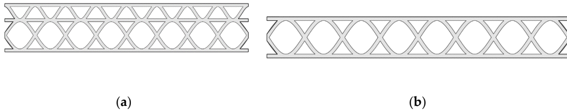
Figure 6. Internal geometry of the walls: (a) Perimeter wall; (b) Internal wall.
