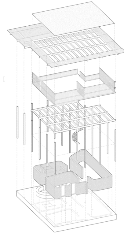
Figure 16. Exploded view of the central block of common spaces.
