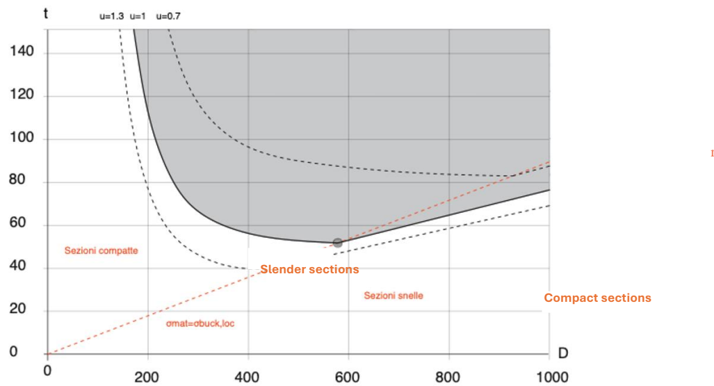
Figure 8. Graph of the resistance domain of the internal wall section.
