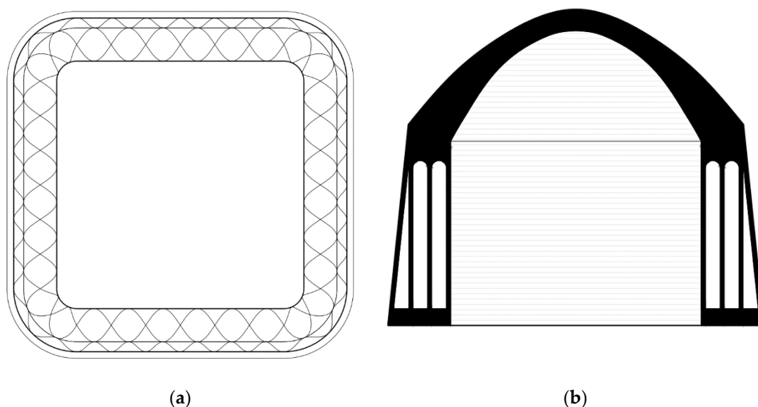
Figure 2. General details of the functional module (for dimensions, see Section 2.2.2): (a) Plan of the module; (b) Section of the module.
