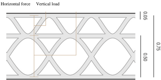
Figure 12. Final infill definition for perimeter wall.
