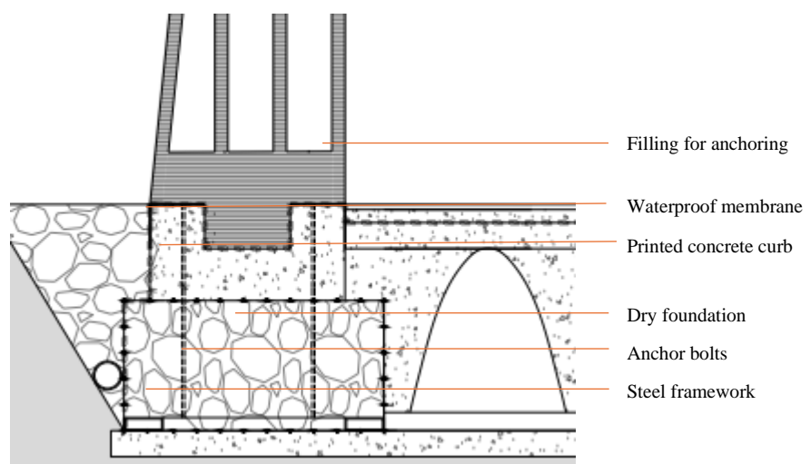
Figure 18. Detail of perimeter wall foundation.
