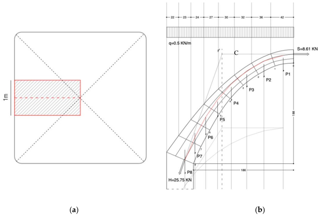
Figure 5. Loads analysis: (a) Study band for the pressure curve; (b) Verification of the pressure curve passing through the middle third of the section.
