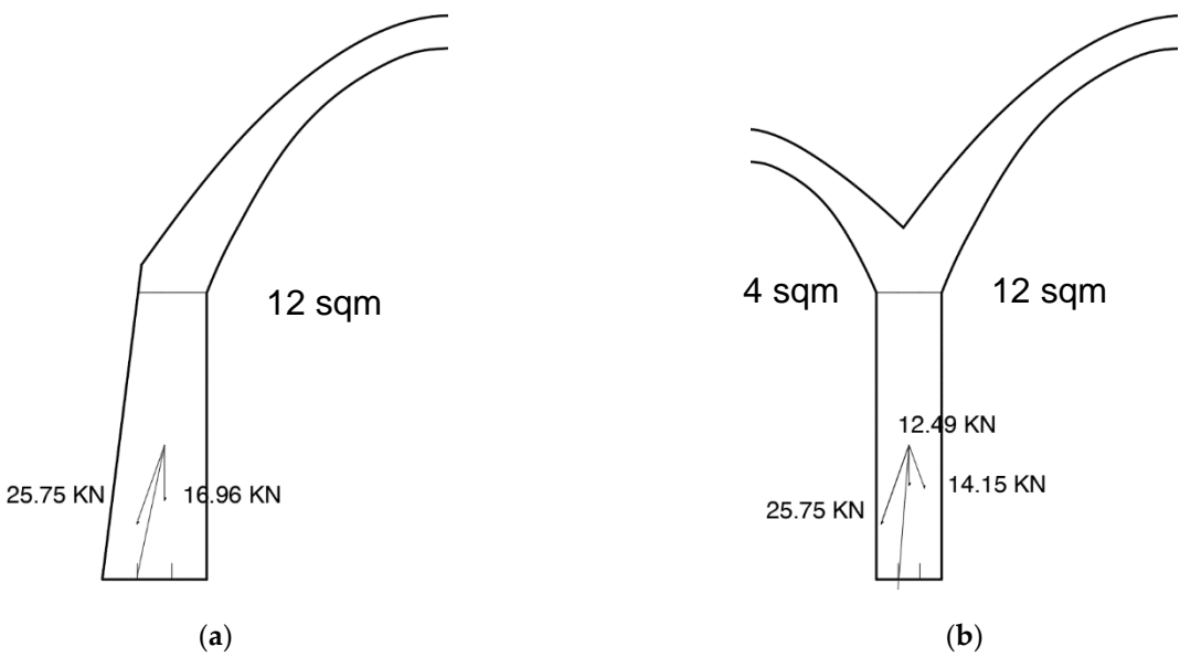
Figure 11. Verification of the force passage within the middle third of the wall base: (a) Perimeter wall; (b) Internal wall.
