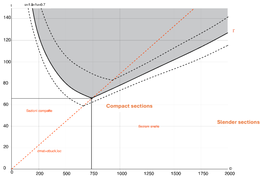
Figure 9. Graph of the resistance domain of the perimeter wall section.
