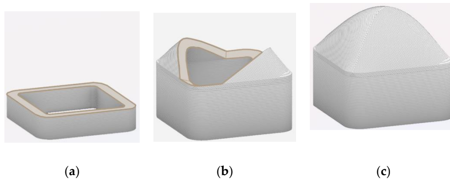
Figure 3. Printing strategies for the walls and roof of the functional module: (a) Printing the walls on horizontal layers; (b) Printing the roofs on 45° inclined layers along the module's diagonal; (c) Completed module.
