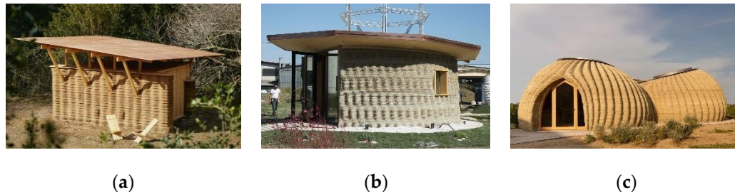
Figure 1. Different support systems for the roofs of 3-D printed houses with earthen materials: (a) The roof resting on the perimeter walls of Tova [18]; (b) The roof resting on internal wooden poles of Gaia [Error! Reference source not found.]; (c) The roof of the global approach of Tecla [20].
