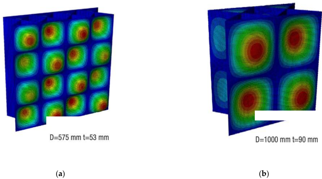
Figure 10. Simulation results in ABAQUS: (a) D=575 mm, t=53 mm; (b) D=1000 mm, t=90 mm.
