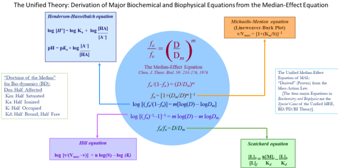
Figure 1. The Median-Effect Equation (MEE) is the unified form of the major biochemical and biophysical specific equations for specific purposes. The MEE is the unified general theory of the Mass-Action Law (MAL) for pharmacodynamics, biodynamics, and bio-informatics (MAL-PD/BD/BI).
