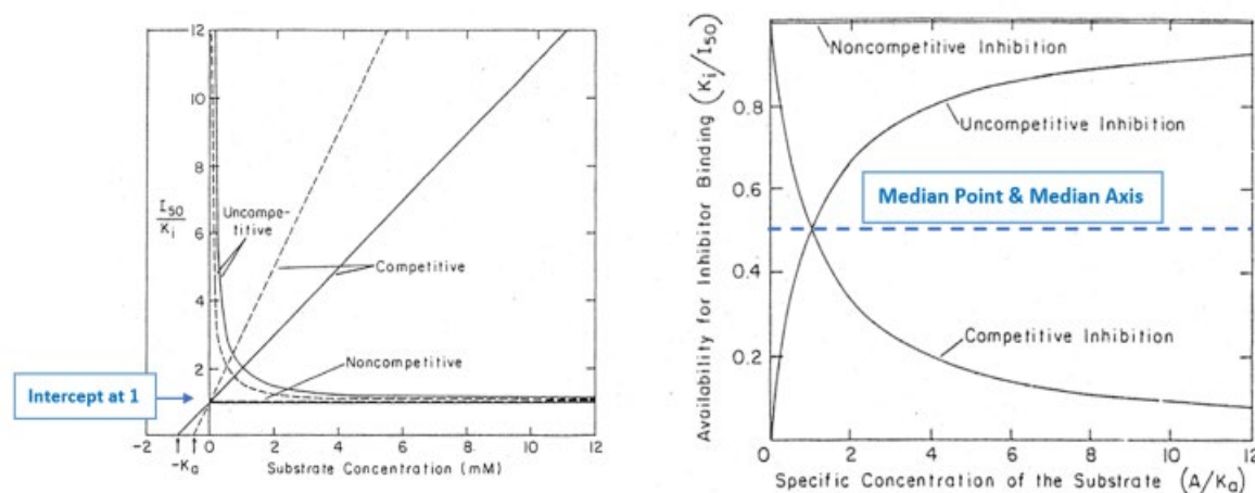
Figure 23. The dose-effect relationship for different mechanisms of action is relevant to the unity theory of one (UTO), median-effect dose, and the median-effect axis.
