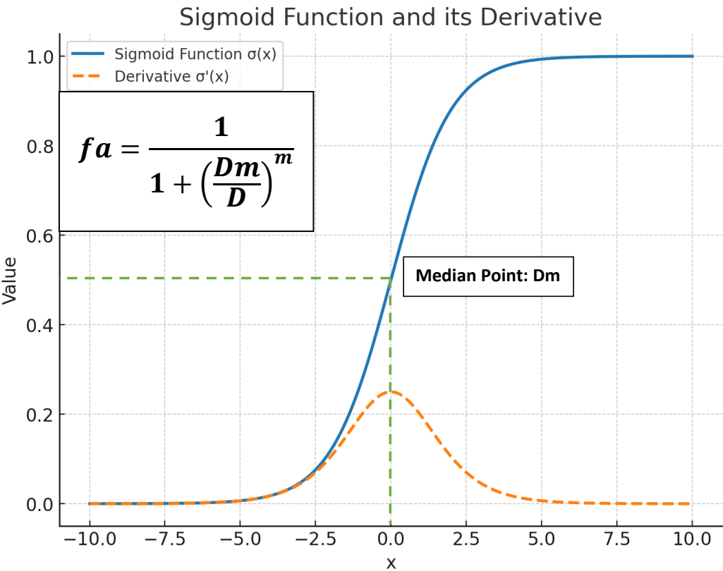
Figure 12. MAL-MEE activation function (fa) indicates a sigmoidal dose-effect curve (DEC) with its derivative showing a symmetrical distribution curve peaks at the Dm, where fa = fu = ½ (The Median point is 0.5), and its intrinsic property of symmetry.
