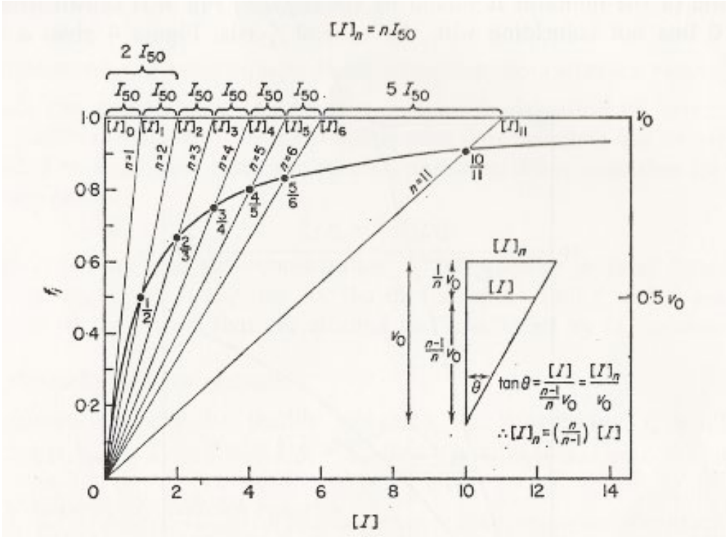
Figure 22. The geometric property of effector dose [I] vs. fractional inhibition (fi) when the dose is in the unit of the median effect dose (I50). The “Dose” can be transformed as the “Median-dose Unit” (normalization) to become a dimensionless ratio due to the ratio-cancellation principle (I/I50 or D/Dm).
