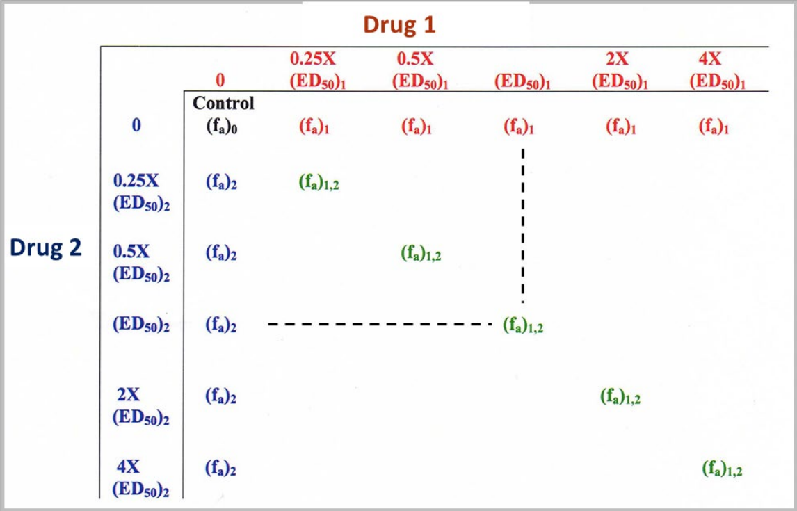
Figure 28A. “Proper Design” is a Prerequisite for Any Efficient MAL-PD Studies. The Simple and Efficient Constant-Ratio Combo Diagonal Design for the Automated Simulations (Recommended). PD-Based Protocol Design (Dose Range, Dose Density, and Dose Ratio) is Critical for Efficient, Cost-Effective Data Analysis in PD-Automated Simulation. The “Non-Constant Ratio Design” can also be used to determine quantitative Synergy. But no automatic computerized simulation is possible. [The Recommended Practical Minimum Number of Data Points for Two Drug Combinations In Vitro, In Animals, and In Clinical Trials need: 16, 10, and 10 Dose-Points, respectively].
