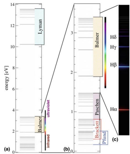
Figure 2. The observed emission line spectrum of atomic hydrogen in chapter 2 atoms [5] (Manini, 2020).
