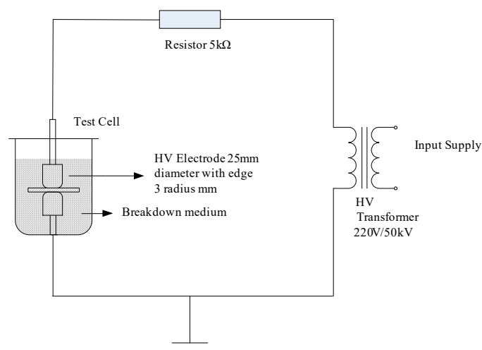
Figure 2. Experimental setup used to perform the breakdown tests.
