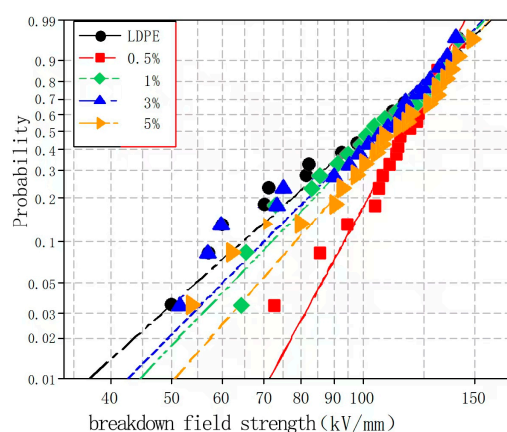
Figure 8. Weibull distributions of the different nano-MgO/LDPE composites during the power frequency breakdown tests.
