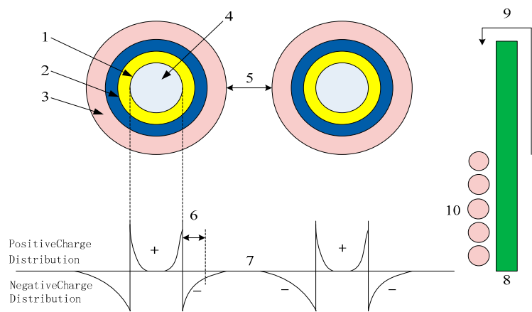
Figure 1. Multi-core model to represent a nanocomposite incorporating spherical inorganic NPs within a polymer matrix. 1) Dense first layer, 2) second layer containing deep traps, 3) third layer containing large amounts of free volume, deep ion traps and shallow electron traps, 4) NP, 5) interparticle distance, 6) Debye shielding distance, 7) NP overlap in the third layer, 8) charge accumulation at the nano filler on the electrode surface, 9) emission of thermoelectrons via the Schottky effect under a high electric field, and 10) changes in charge injection through the neutralizing effect.
