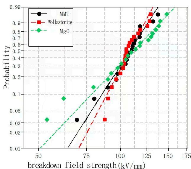
Figure 10. Weibull distributions of the power frequency breakdown characteristics of the different composites.
