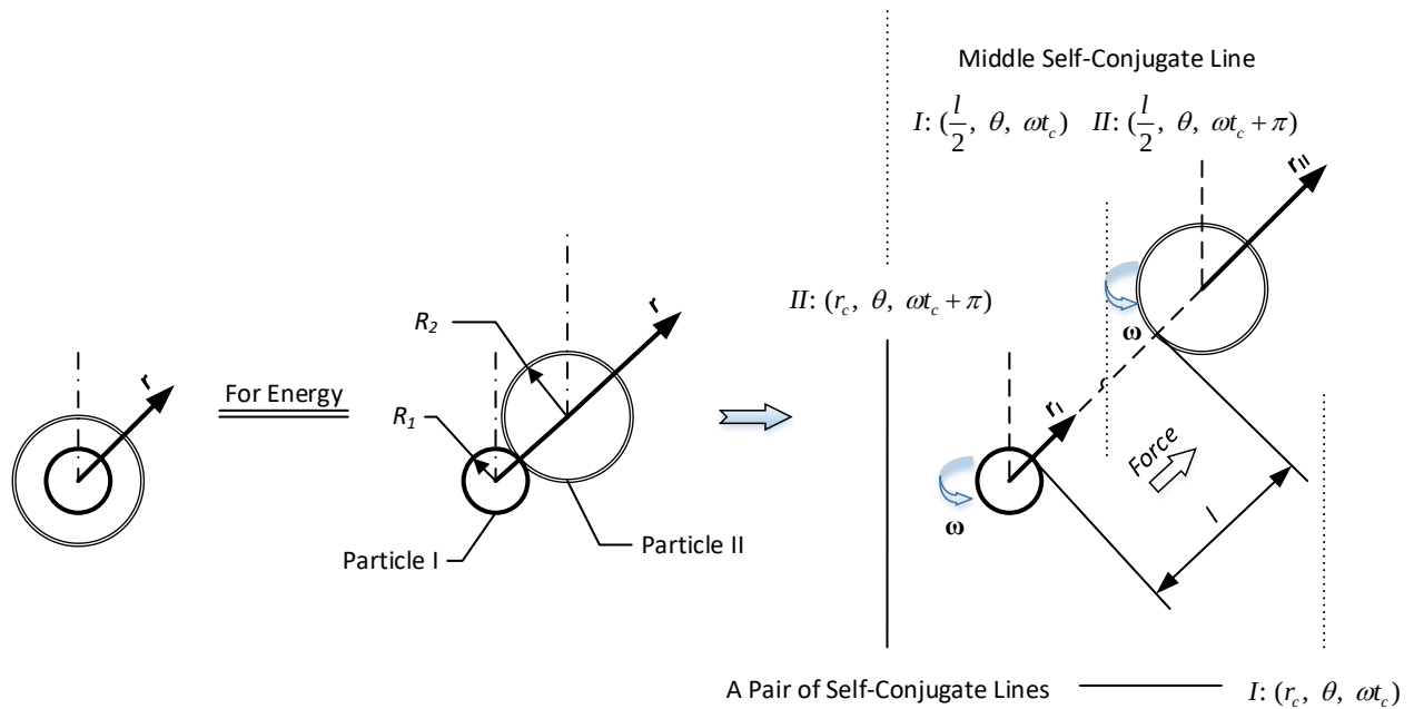
Figure 2. Energy conversion between two primary particles.
