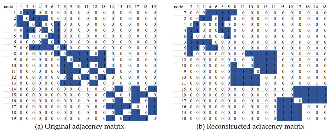
Figure 4. The matrix reconstruction method for ‘network19’
