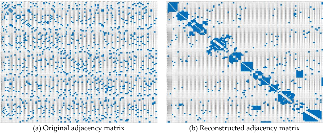
Figure 7. The matrix reconstruction method for ‘football’
