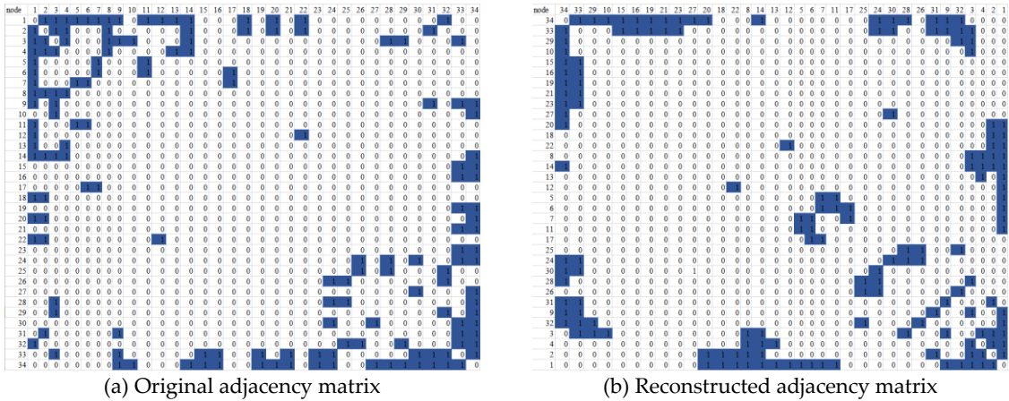
Figure 5. The matrix reconstruction method for ‘karate’
