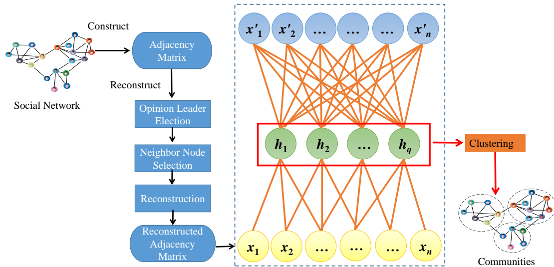
Figure 1. The proposed deep community detection method
