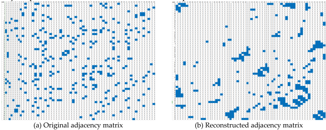
Figure 6. The matrix reconstruction method for ‘dolphins’
