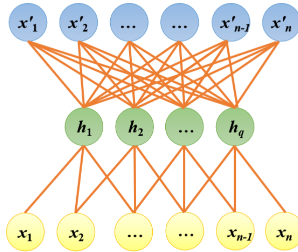
Figure 3. A general case of auto-encoder based on convolutional neural network
