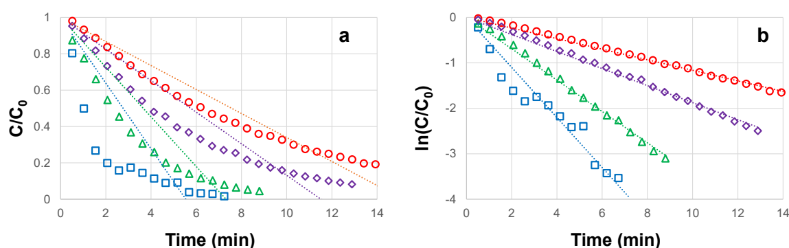
Figure 1. Degradation of 1 (squares), 5 (triangles), 15 (rhombus) and 20 (circles) mg L -1 CBZ with 0.5 mg L -1 TiO 2 , 5 mg L -1 of H 2 O 2 and 8 UVC lamps. Panel (a) and panel (b) show the concentration related to its initial value ( C/C_0 ), and its natural logarithm, respectively. Lines indicate linear regression for each set.
