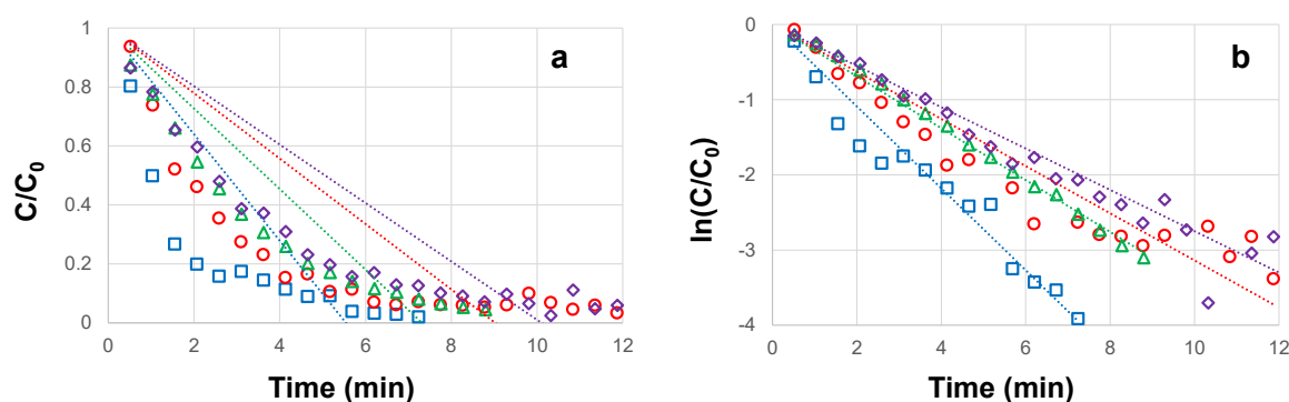
Figure 2. Degradation of 1\text{ mg L}^{-1} CBZ with 0.5\text{ mg L}^{-1} \text{TiO}_2 , 8 UVC lamps and 0.5 (rhombus), 1 (circles), 2 (triangles) or 5\text{ mg L}^{-1} (squares) of \text{H}_2\text{O}_2 . Panel (a) and panel (b) show the concentration related to its initial value ( C/C_0 ), and its natural logarithm, respectively. Lines indicate linear regression for each set.
