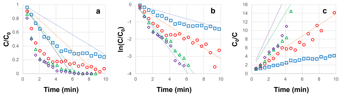
Figure 4. Degradation of 1 mg L -1 CBZ with 5 mg L -1 H 2 O 2 , 0.5 mg L -1 TiO 2 and 2 (squares), 4 (circles), 6 (triangles) or 8 (rhombus) UVC lamps. Panels (a), (b) and (c) show the concentration related to its initial value ( C/C_0 ), its natural logarithm ( \ln(C/C_0) ), and its reciprocal ( C_0/C ), respectively. Lines indicate linear regression for each set.
