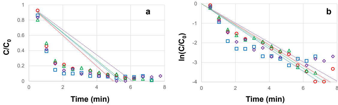
Figure 3. Degradation of 1 mg L -1 CBZ with 5 mg L -1 H 2 O 2 , 8 UVC lamps and 0.02 (squares), 0.05 (rhombus), 0.2 (circles) or 0.5 mg L -1 (triangles) of TiO 2 . Panel (a) and panel (b) show the concentration related to its initial value ( C/C_0 ), and its natural logarithm, respectively. Lines indicate linear regression for each set.
