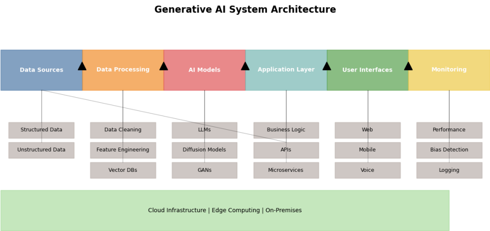
Figure 2. System Architecture Diagram depicting the layered components of a Generative AI solution from data sources to user interfaces.
