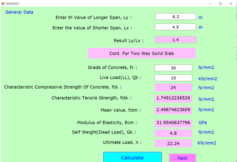
Figure 5. Material Property of Concrete Result
