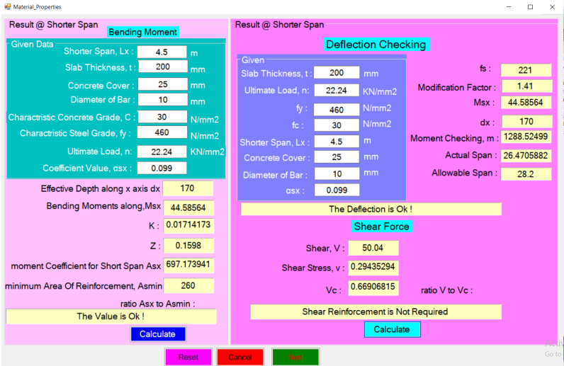
Figure 8. Result for the input data @ Short Span
