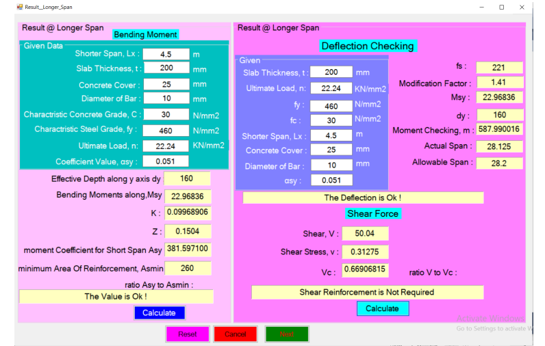
Figure 11. Results @ Long Span
