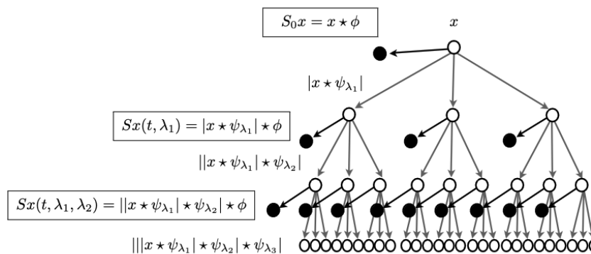
Figure 3. Wavelets traversing CNNs, source: https://www.di.ens.fr/data/publications/papers/1304.6763v1.pdf
