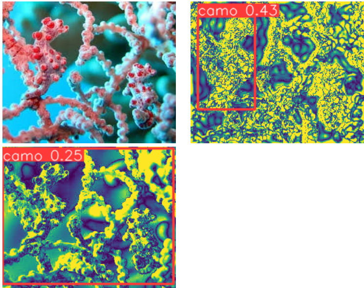
Figure 8. Ensemble Model detecting camouflaged object, Model that did not use fourier transforms failed to detect camouflage object, other two models (Edge enhanced, Shape enhanced) were able to detect. Edge enhanced did best
