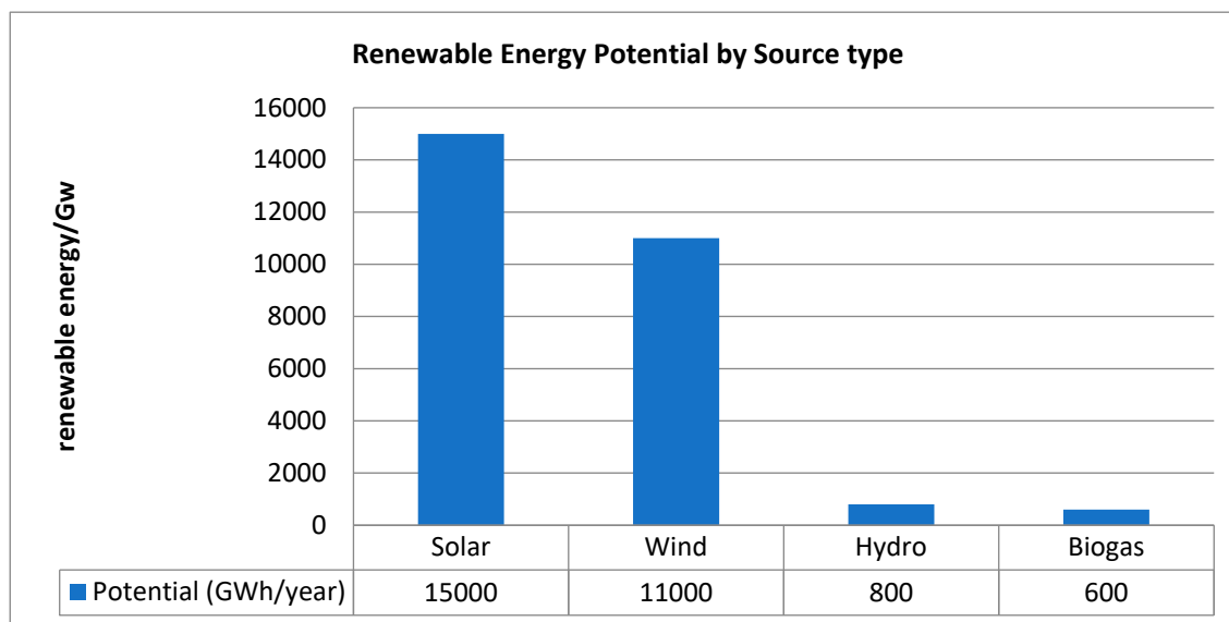
Figure 6. Estimated renewable energy potential by resource type (UNDP & IRENA, 2024).
