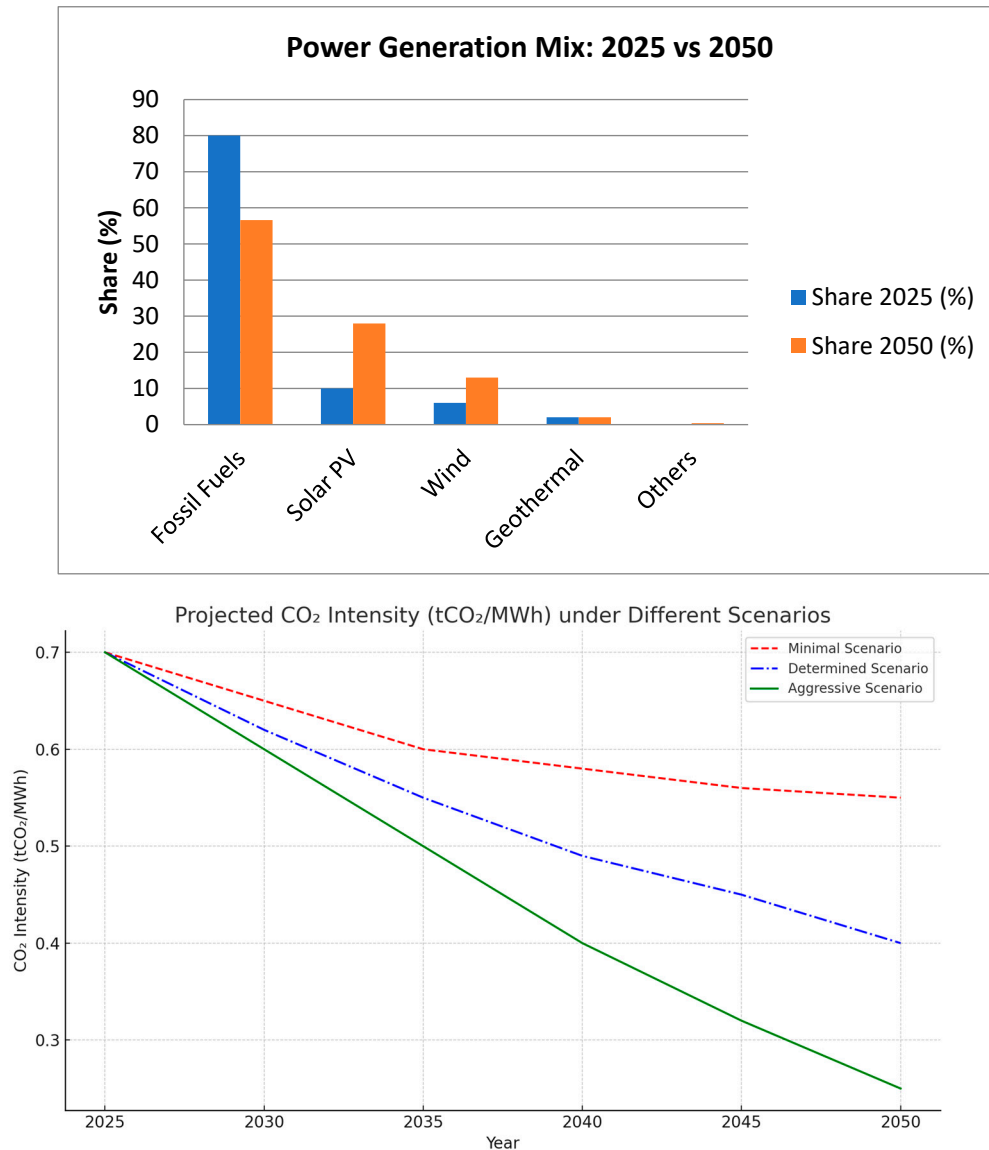
Figure 18. Yemen's projected carbon intensity reduction trend under various scenarios (UNDP Model, 2024).
