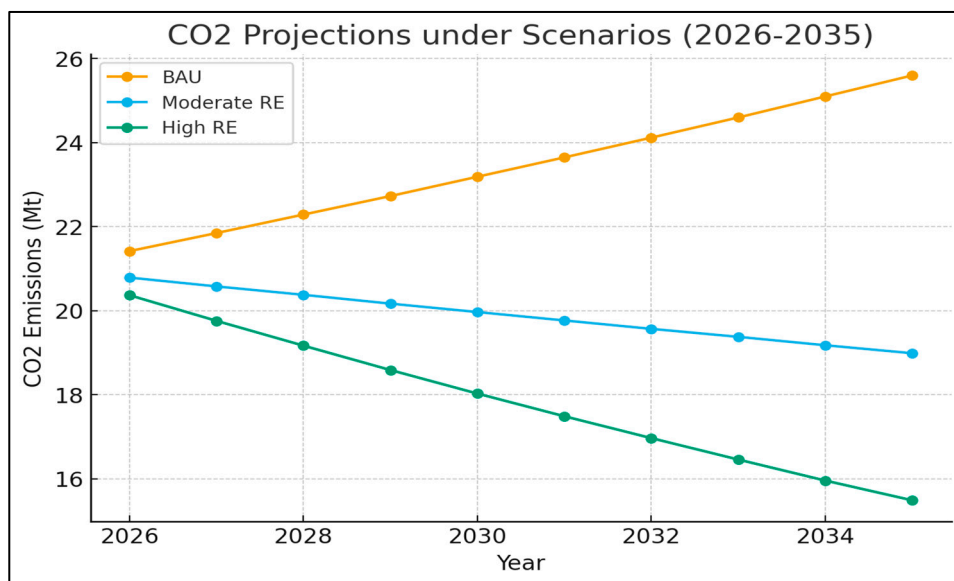
Figure 10. CO 2 projections under BAU, Moderate RE, and High RE (2026–2035).
