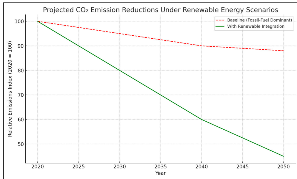
Figure 20. Projected CO 2 emission reductions under renewable integration scenarios (UNDP, 2024).
