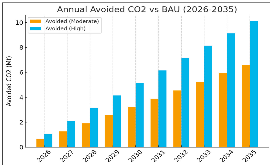
Figure 11. Cumulative CO 2 avoided over 2026–2035 for both scenarios.
