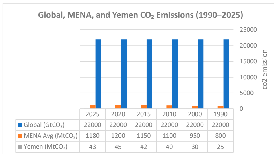
Figure 5. Comparative co2 emission among selected MENA countries (IRENA, 2024).
