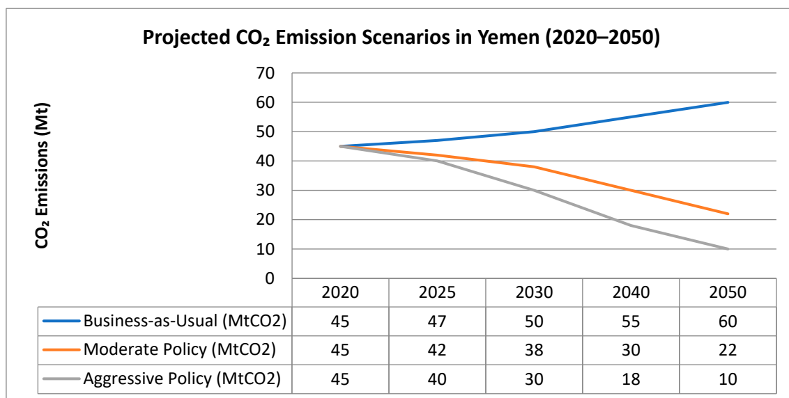
Figure 12. Projected CO 2 Emission Scenarios in Yemen (2020–2050).
