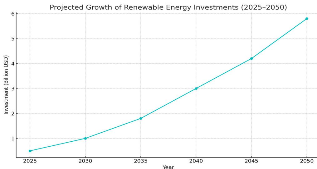
Figure 21. Projected renewable energy investment growth in Yemen through 2050.
