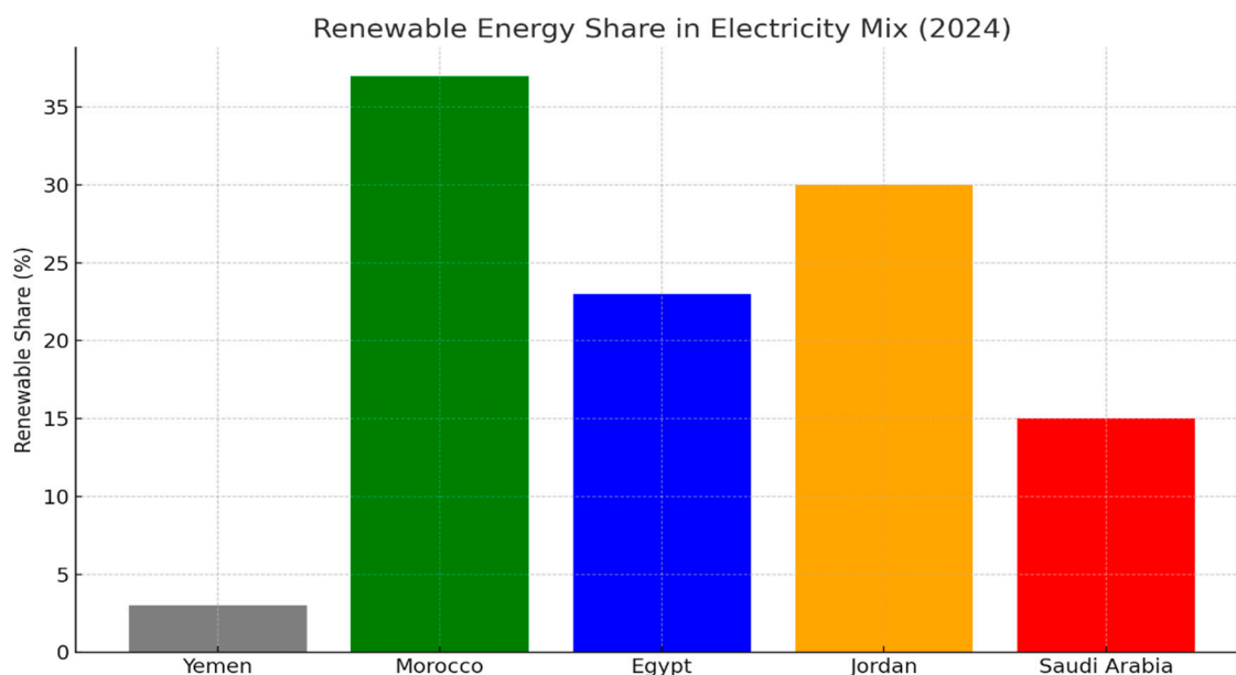
Figure 4. Compares Yemen's renewable progress with selected MENA countries.
