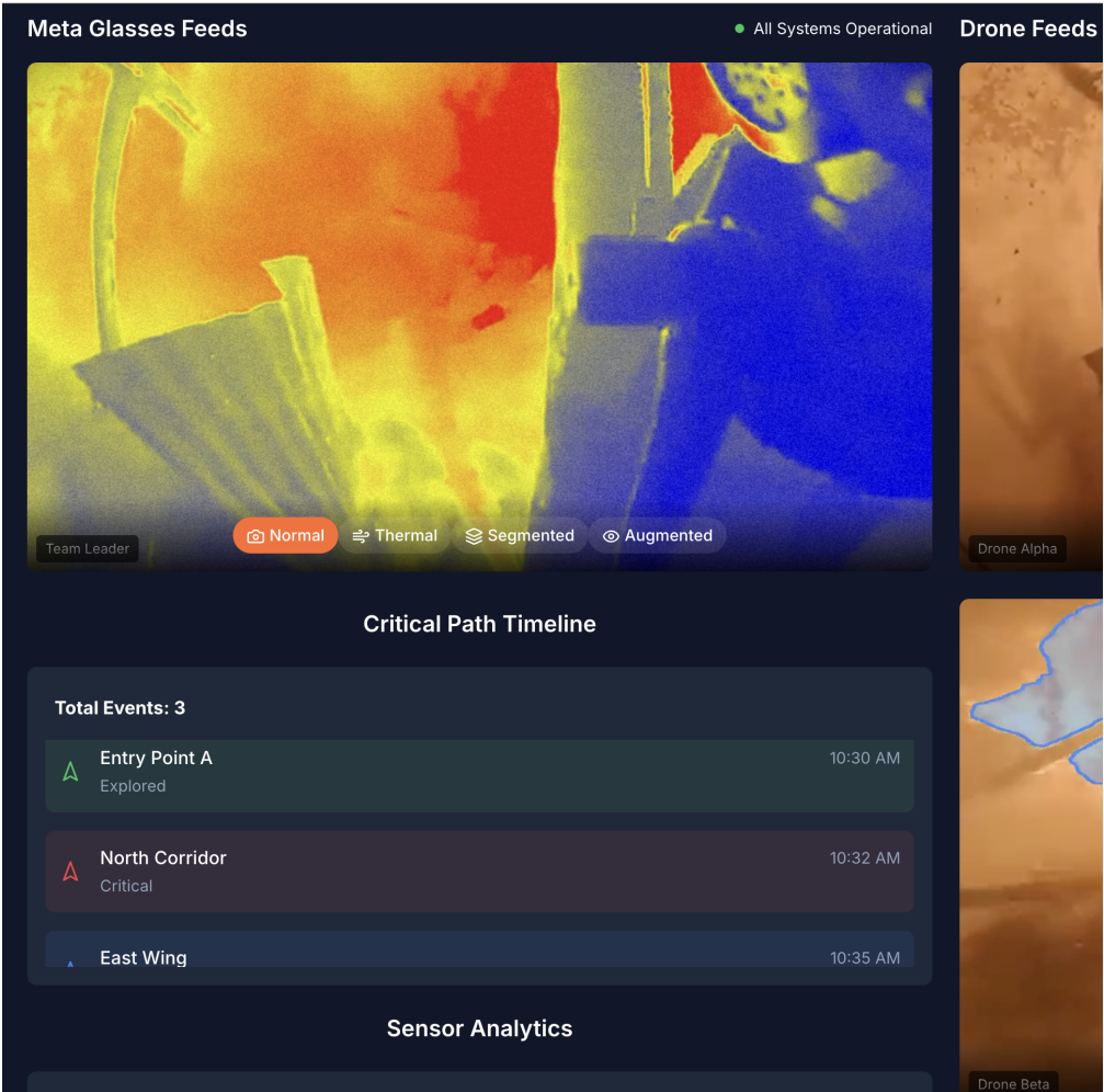
Figure 2. PUSHPA’s integrated UI, which provides live telemetry from drones and Meta Glasses, overlays AI-driven insights, and enables real-time user interaction through a streamlined interface.
