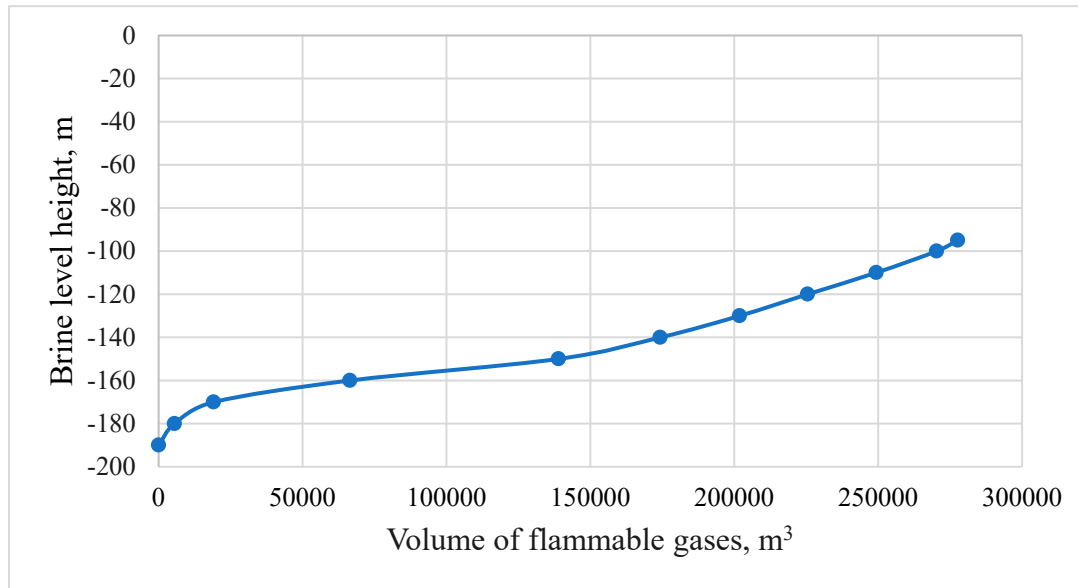
Figure 3. Dependence of the volume of flammable gases released during the dissolution of pillars on the brine level height.
