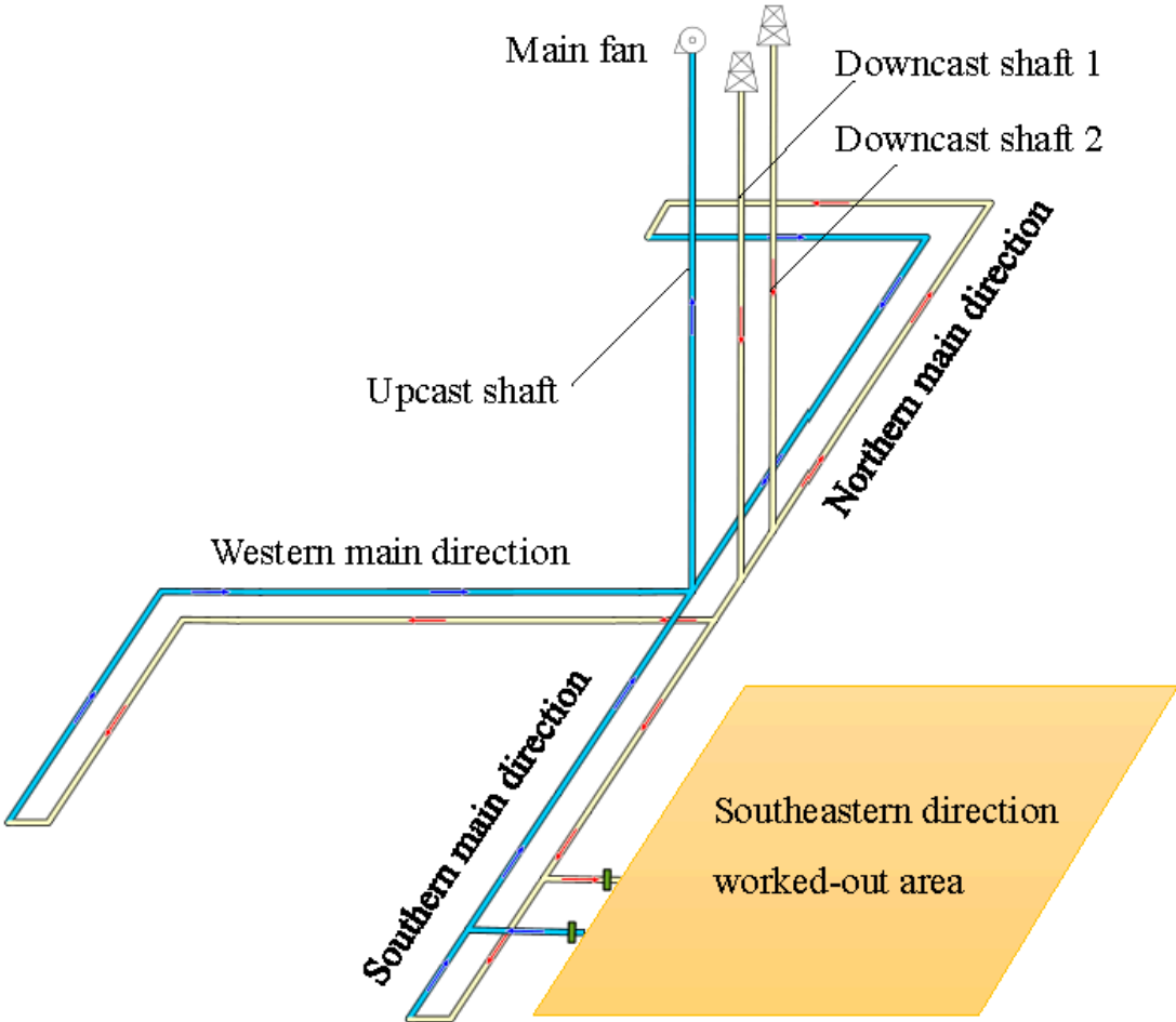
Figure 1. Schematic diagram of the mine ventilation network.
