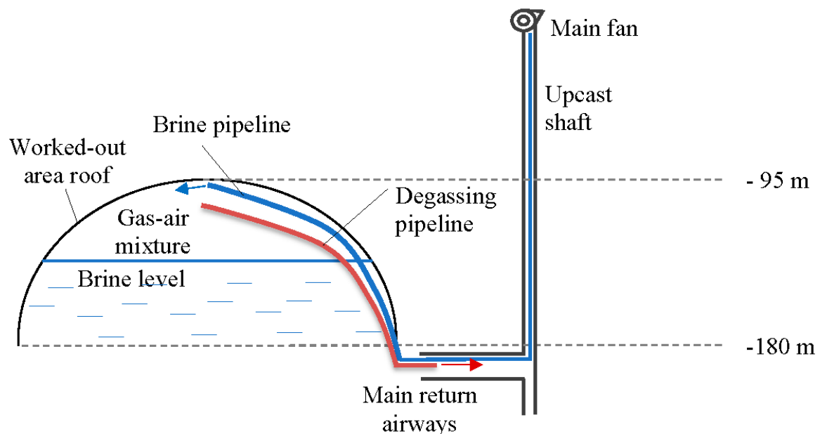
Figure 2. Schematic diagram of the closed section of the mine, brine and degassing pipelines.
