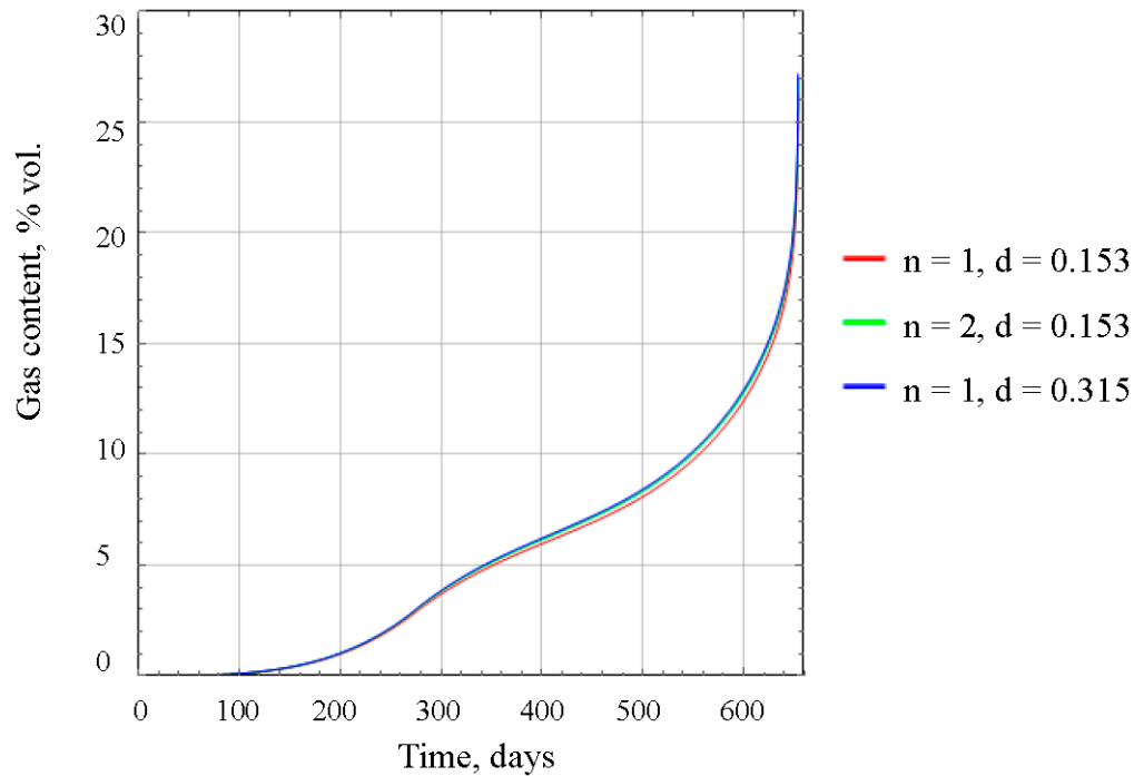
Figure 6. Time dependency of the gas concentration in the gas-air mixture emanating from the pipeline.
