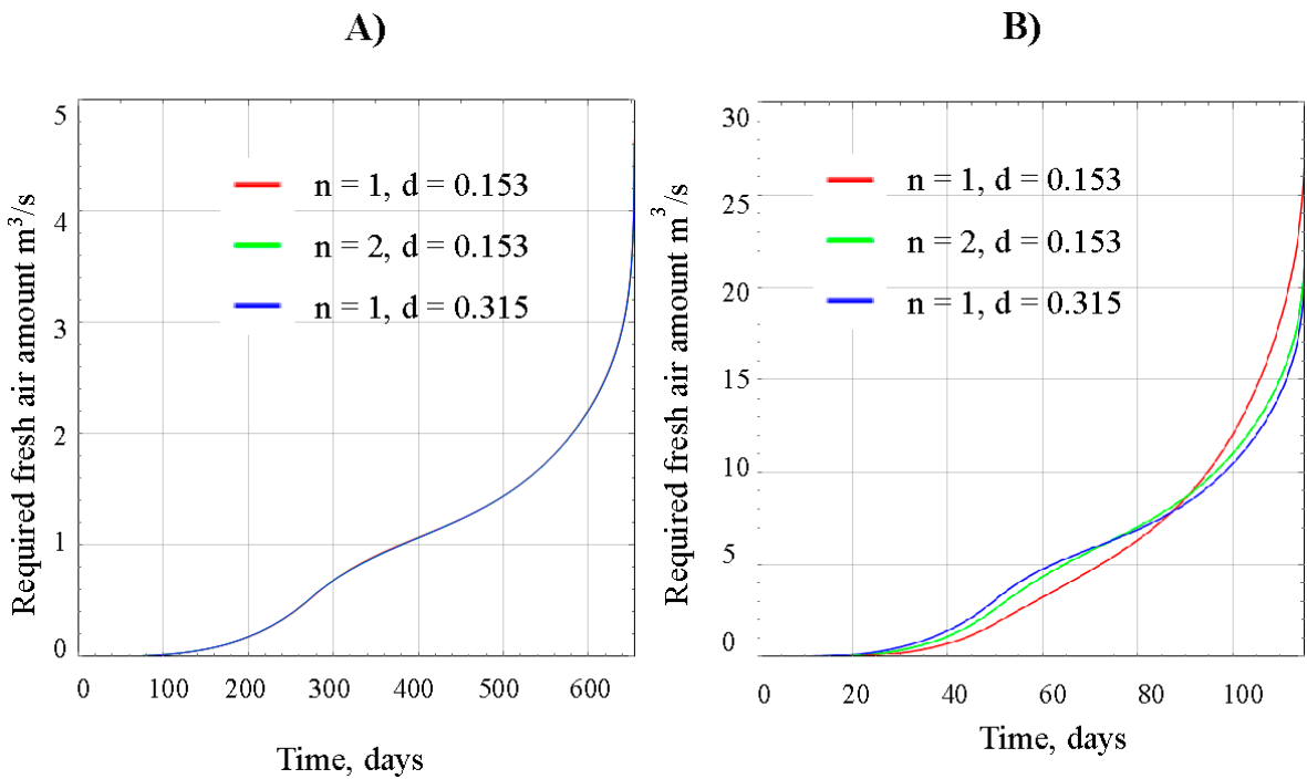
Figure 10. Required fresh air flow in ventilation working to dilute combustible gases to the threshold limit value: A) Scenario 1; B) Scenario 2.
