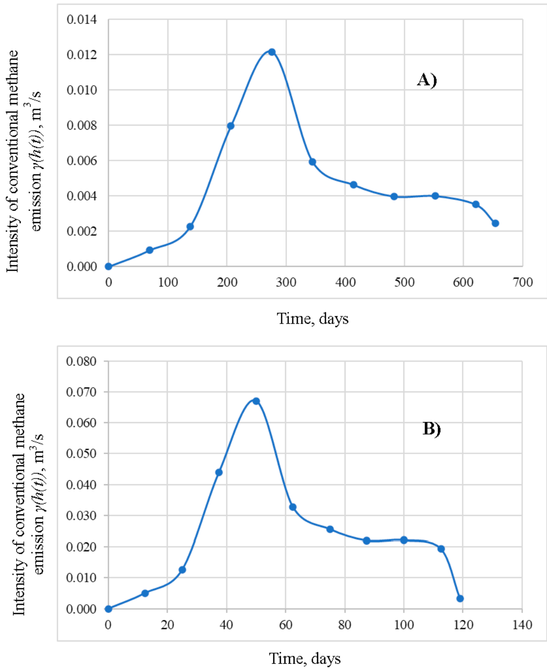
Figure 4. Time dependences of the intensity of flammable gas emissions in terms of conventional methane: A) for scenario 1; B) for scenario 2.
