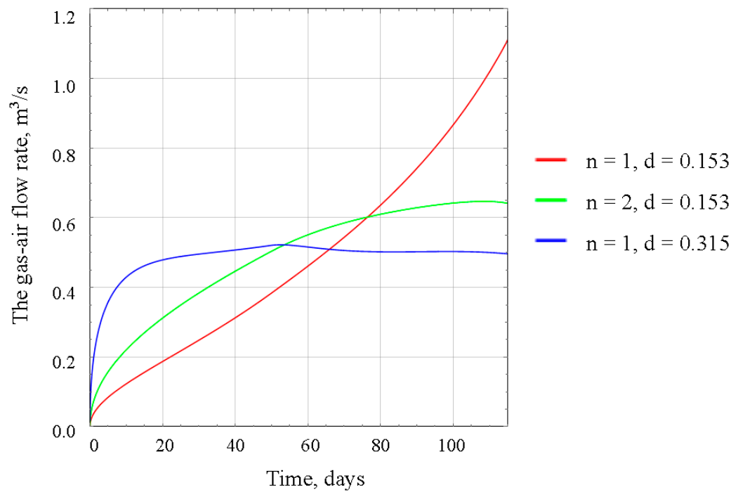
Figure 8. Time dependency of the gas-air flow rate emanating from the pipeline.
