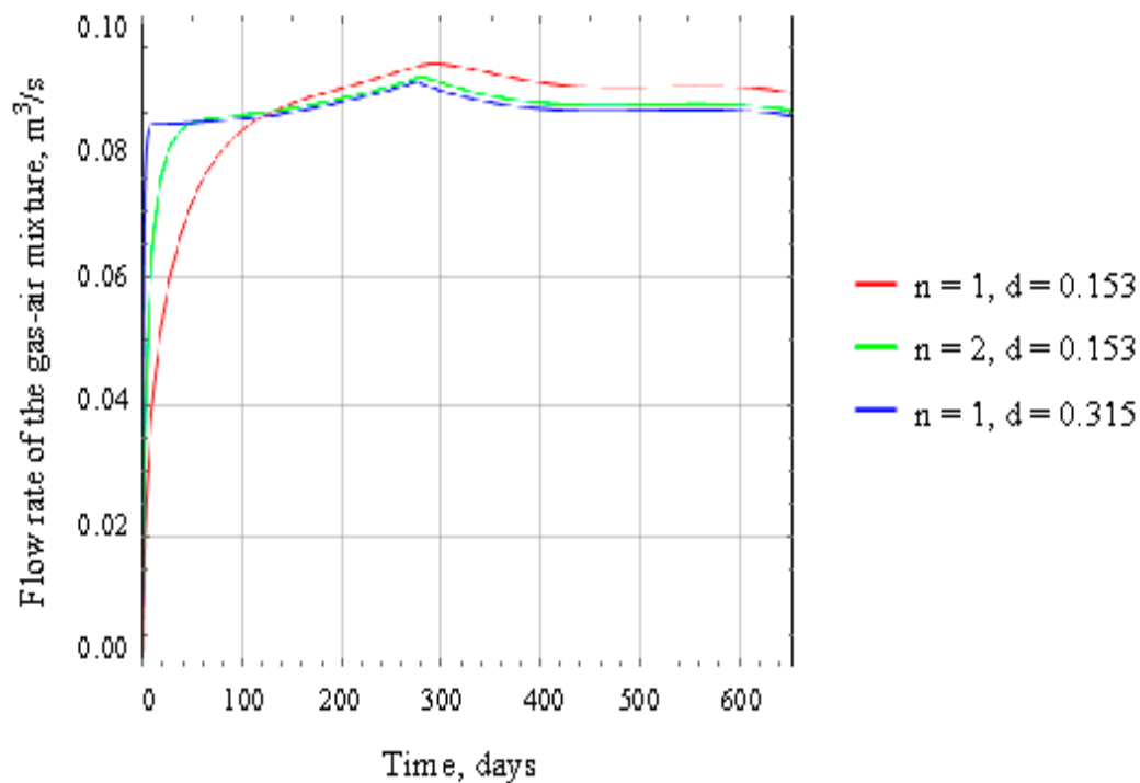
Figure 5. Time dependency of the gas-air mixture flow rate emanating from the pipeline.
