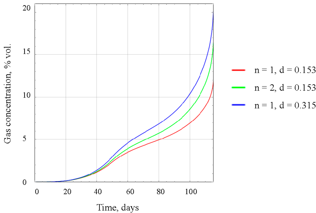
Figure 9. Time dependency of the gas concentration in the gas-air mixture emanating from the pipeline.
