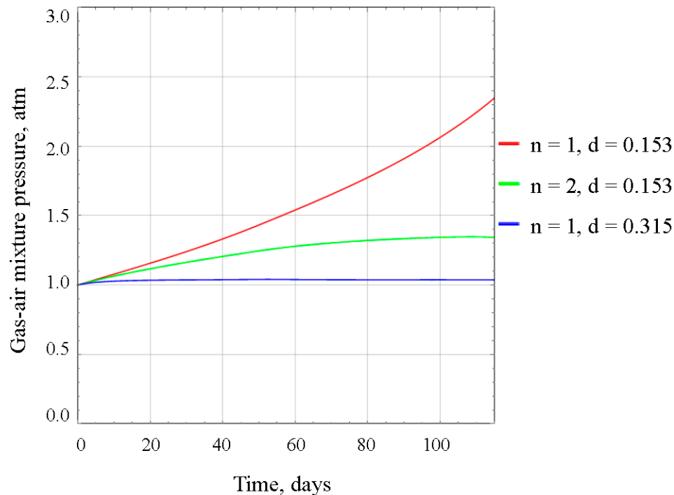
Figure 7. Time dependency of the gas-air mixture pressure in the unflooded section of worked-out area.
