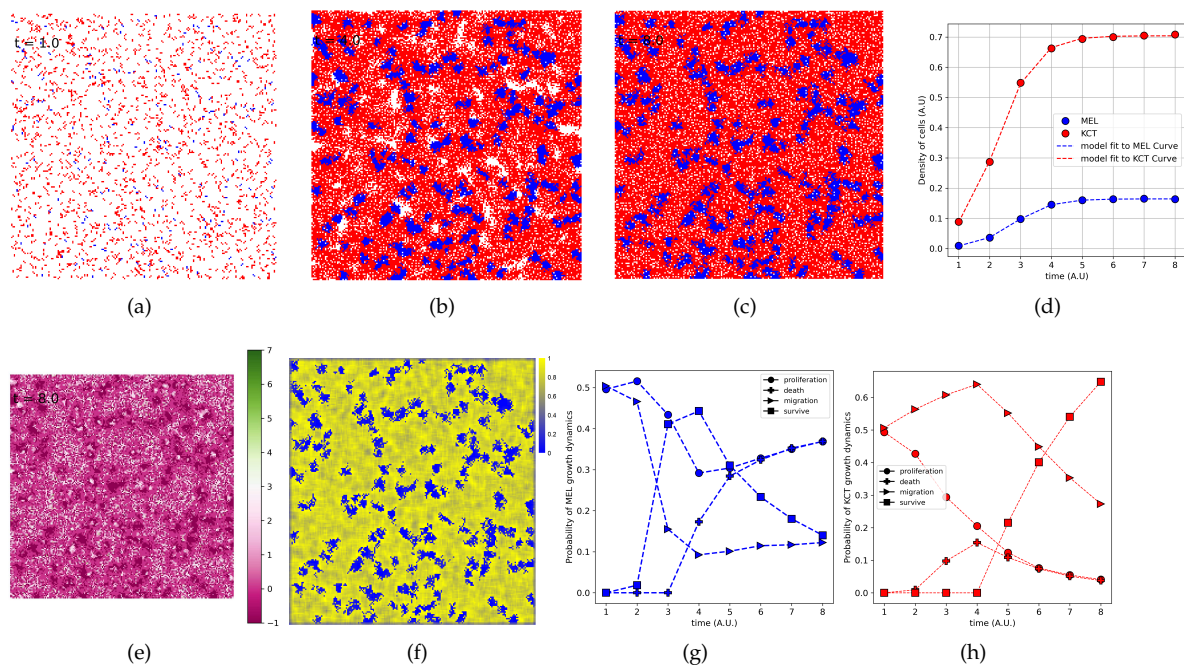
Figure 6. The spatial population and tumor growth dynamics. (A), (B), and (C) frames correspond to days 1, 4, and 8. Blue represents T , and red represents H . (D) Growth curves of T and H . E Spatial distribution of the cells according to the values of \rho_{max} at day 8. In the bar of color at right, the shades of green to pink represent the \rho_{max} values. (F) Heatmap representing H density over all focal cell neighborhoods at day 8. In the bar of color at right, the shades of blue to yellow represent the percentage of occupied vertex by H in all focal cell neighborhoods. (G) Probabilities of T tumor growth dynamics (H) Probabilities of H tumor growth dynamics.
