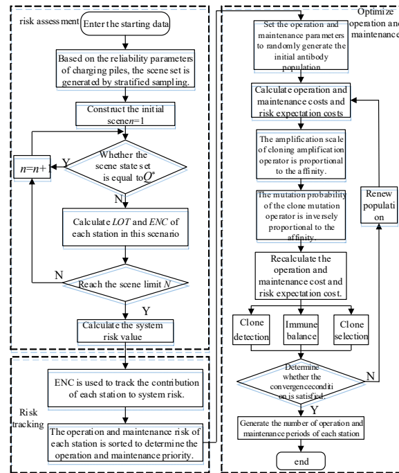
Figure 5. Operation and maintenance strategy optimization process.
