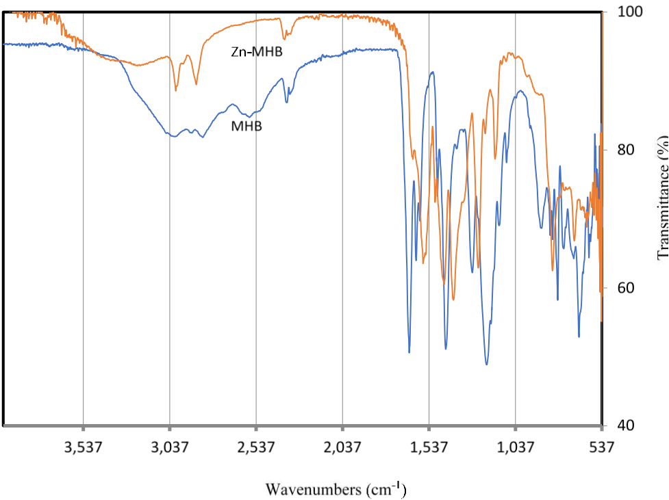
Figure 2. FT-IR spectra of MHB ligand and Zn-MHB complex.
