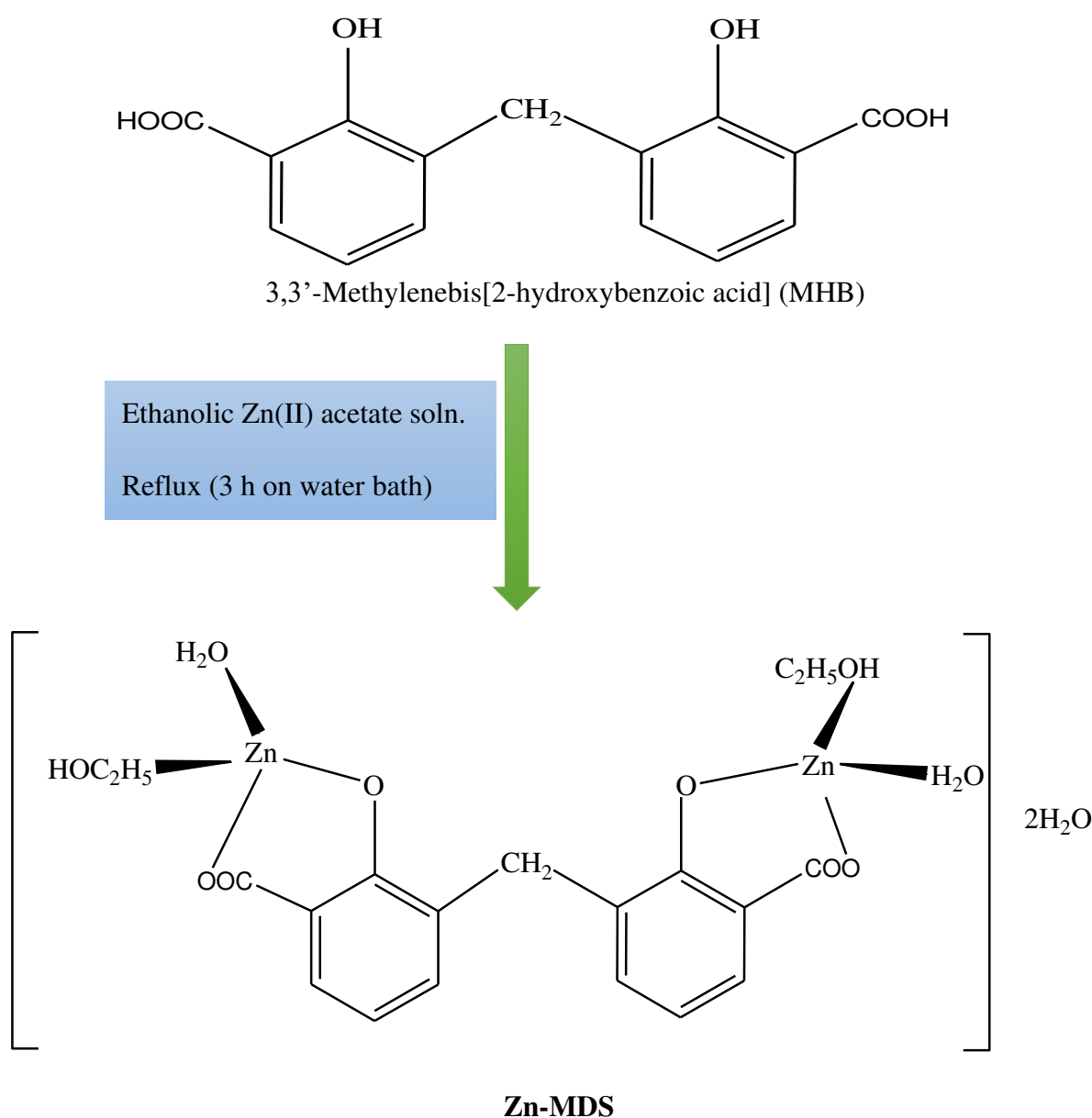
Scheme 1. Schematic diagram of Zn-MHB complex formation.
