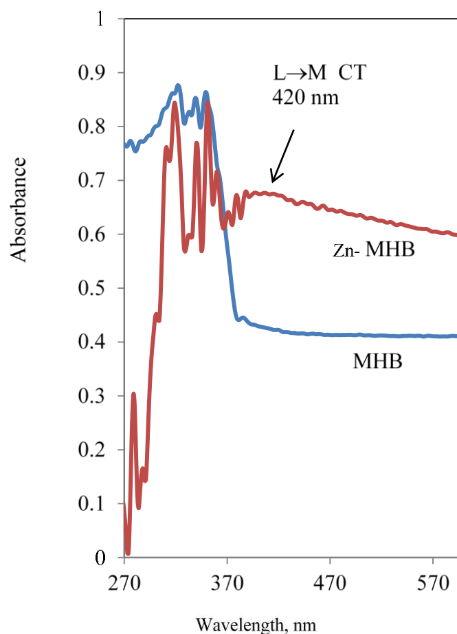
Figure 3. Electronic spectrum of MHB and Zn-MHB.
