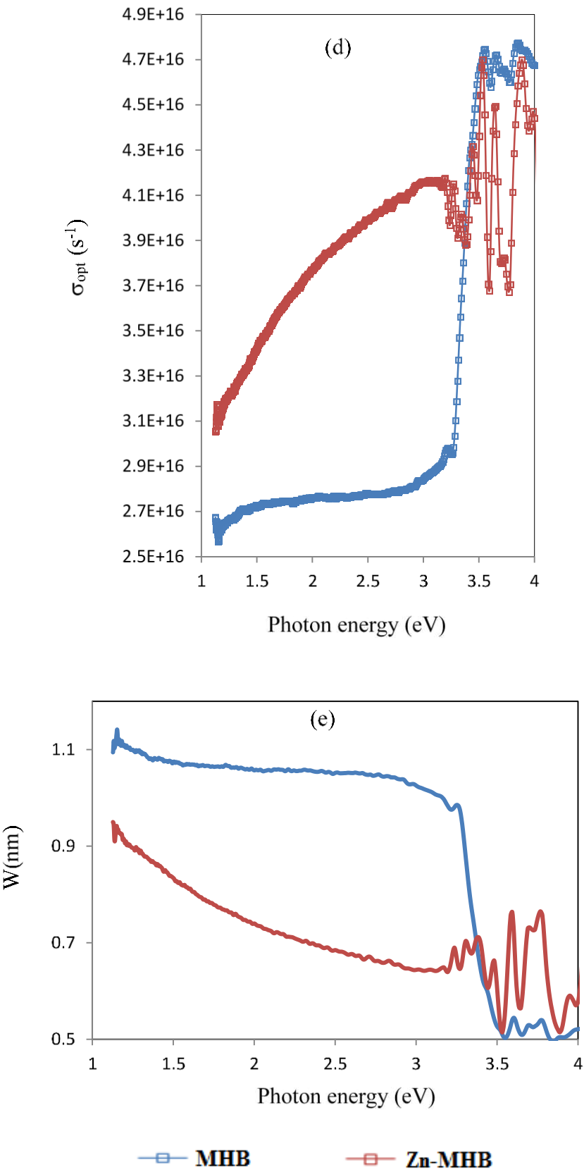
Figure 6. Variation of optical parameters for ligand and complex (a) transmittance, T, (b) band gap energy, E_g , (c) refractive index, n (d) optical conductivity, \sigma_{opt} and (e) penetration depth, W. .
