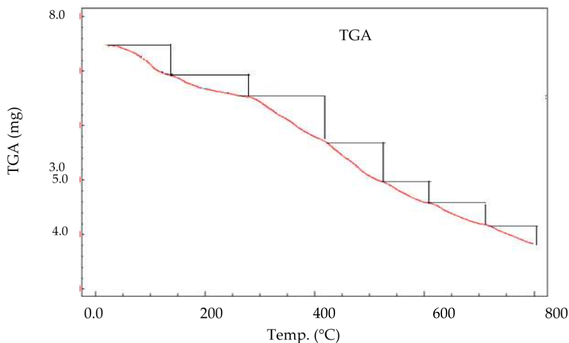
Figure 4. TGA of Zn-MHB.
