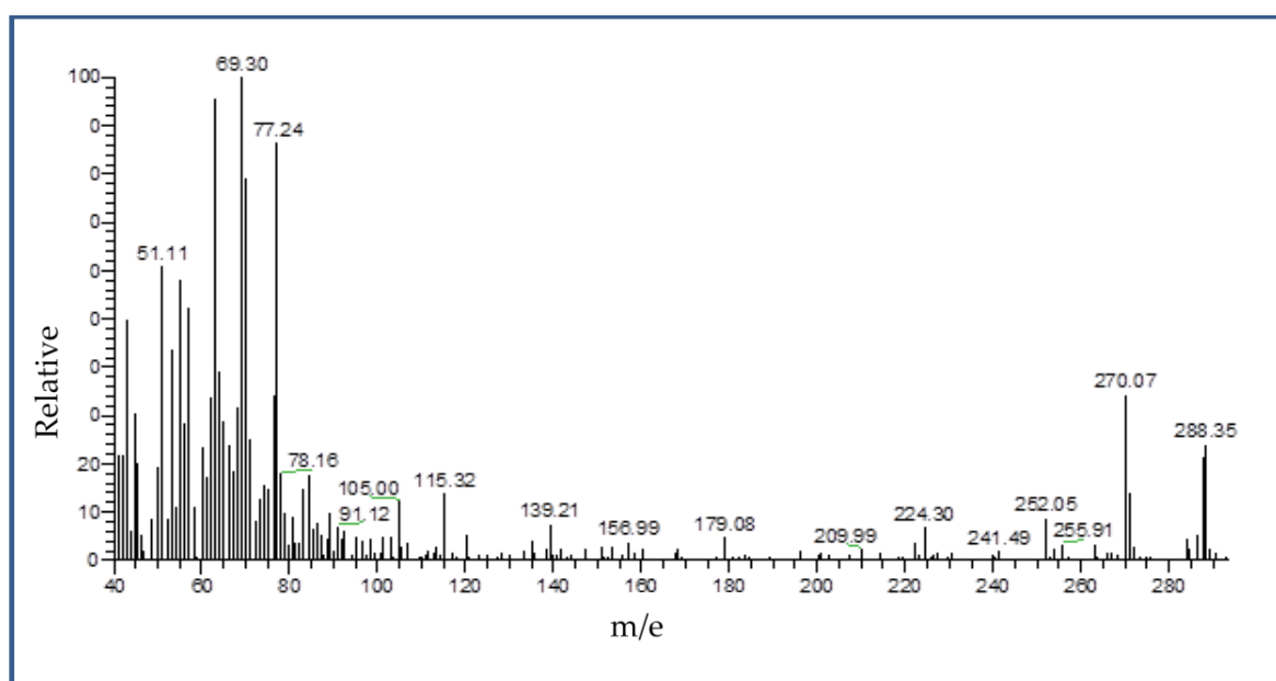
Figure 1. Mass spectrum of MHB.
