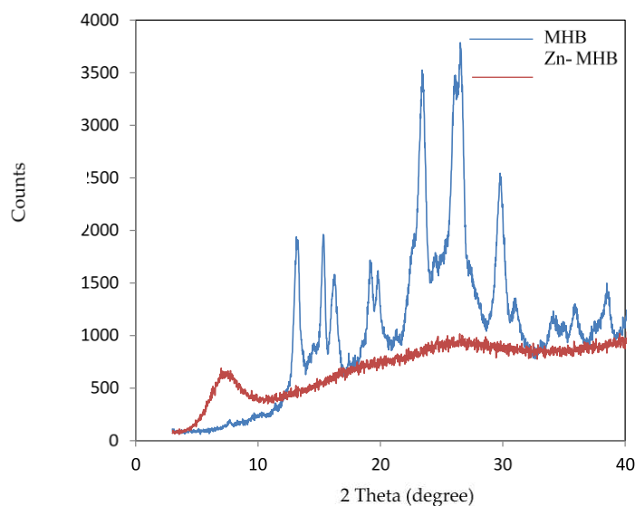
Figure 5. XRD graph of MHB and Zn-MHB.
