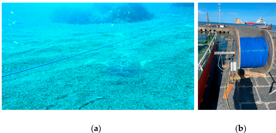
Figure 1. (a) DAS cable deployed on the seafloor of Panarea in the area of natural CO 2 bubbles emission (Calcara). (b) DAS cable reel positioned at the Panarea harbor pier.
