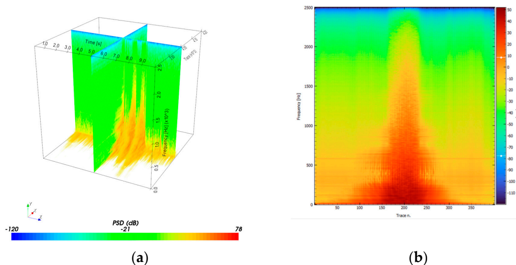
Figure 9. (a) 3D spectrogram of Power Spectral Density (PSD) values of the reference signal from scuba tank, recorded by Carina®. (b) 2D heatmap of the Power Spectral Density (PSD) of a representative record of 10 s during the scuba tank air release test on the DAS cable.
