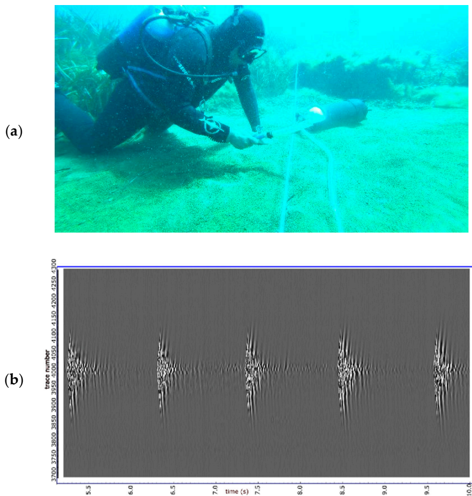
Figure 3. (a) Tap test on the cable performed by scuba diver at selected locations. (b) Tap test signals recorded with the DAS cable shown as a function of time.
