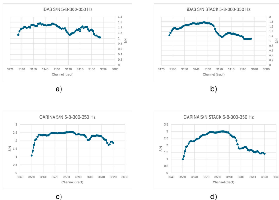
Figure 7. Signal-to-noise ratio (SNR) of (a) the first iDAS record and (c) the first Carina® record computed in a 10 s window. (b,d) show the SNR of the 24 stacked iDAS and Carina® records, respectively.
