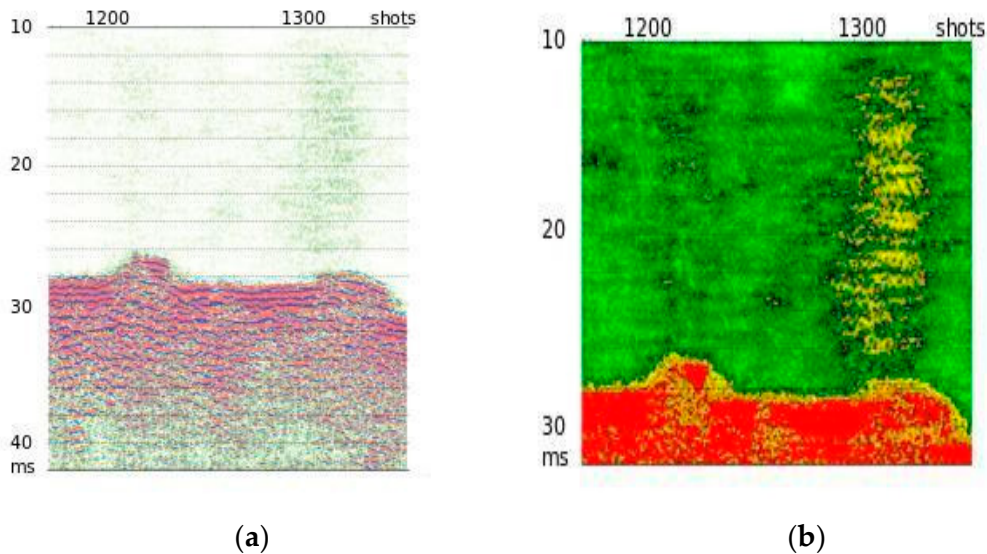
Figure 11. Active seismic results. a) VHRs profile acquired on the locations where natural gas leakage occurs (Calcara 1 and Calcara 2). b) The strength of reflectivity (calculated with Hilbert transform) image of the VHRs profile acquired between Calcara 1 and Calcara 2. Red indicates maximum intensity, green indicates lower intensity.
