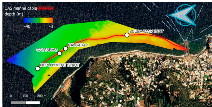
Figure 2. Deployment of the DAS cable laid down by the vessel offshore Panarea (red line). Relevant sites along the cable trajectory are indicated in the map, which includes bathymetric data of the surrounding area.
