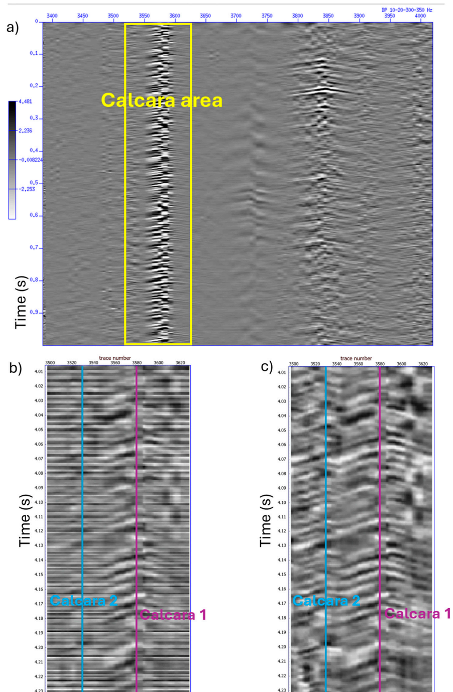
Figure 5. Seismic signal acquired along the deployed DAS cable for a) the total length of the engineered fiber that includes the emission zone of Calcara. Optical noise removal was applied to the data. b) Insight of Calcara area before noise reduction and c) after noise reduction and with the addition of an Ormsby filter 5-8-280-300 Hz. Emission points (centered at 3577 and 3527) correspond to Calcara 1 and 2 and are marked in the figure by a magenta and a blue line, respectively. All data were acquired with Carina ® interrogator.
