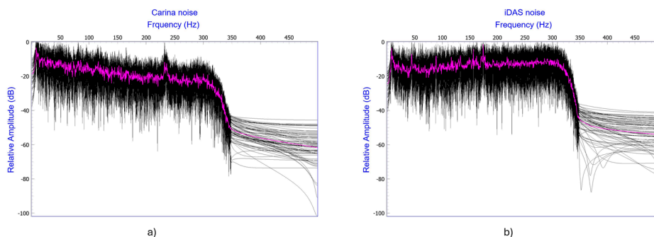
Figure 8. Amplitude spectra of the noise (black lines) of a) Carina® and b) iDAS. The magenta line is the average spectrum of the traces.
