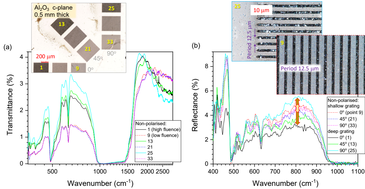
Figure 1. Front-side ablation of Al 2 O 3 . (a) Transmittance T (wavenumber is in log-scale) and (b) reflectance R measured in mid-to-far IR spectral range; insets show optical images of laser ablated Al 2 O 3 ; single-point measurements were carried out on the laser-ablated regions (numbers are indicated on insets); laser: central wavelength \lambda = 1030 nm, pulse duration t_p = 230 fs, repetition rate f_{rep} = 200 kHz, pulse energy E_p = 10 \mu J, numerical aperture NA = 0.45 (focal diameter 1.22\lambda/NA \approx 2.8 \mu m); the grating period was 12.5 \mu m with h = 1 - 10 \mu m depth of the ablated-groove; depth defined by ablation fluence, scan speed and number of repeated passes N_p = 1, 2, 3 (without change of vertical focal spot position). Constant density of pulses 100 \text{mm}^{-1} for shallow gratings and 500 \text{mm}^{-1} for deep gratings was used.
