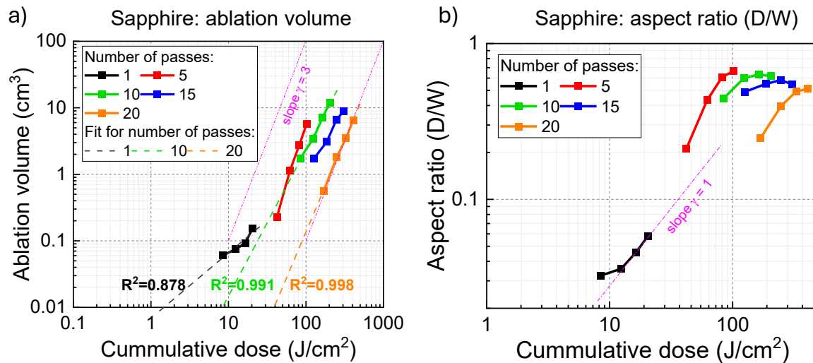
Figure 3. Back-side ablation of \text{Al}_2\text{O}_3 . (a) The effective ablation volume and (b) aspect ratio of ablated grooves on sapphire engraved by 515 nm/230 fs/200 kHz Gaussian beam irradiation. The x-axis is the total dose F_p \times N_p , where N_p is the number of passes. N is the number of pulses per focal spot diameter N = d_p/v_s/f . The pulse-to-pulse separation was \Delta x = 0.5 \mu\text{m} for the constant pulse density mode of 2000 \text{ mm}^{-1} corresponding to N \approx 3 , scan speed v_s = 15 \text{ mm/s} , laser repetition rate f = 200 \text{ kHz} . The pulse fluence F_p = E_p/(\pi[d_p/2]^2) ( E_p pulse energy), the ablation volume (conical pyramid) V = \pi(W/2)^2 D/3 and the aspect ratio \alpha = D/W were calculated with W the width and D the depth of the groove; R^2 is the coefficient of determination for each linear fitting. Focusing with NA = 0.45 objective lens; d_p = 1.22\lambda/NA = 1.4 \mu\text{m} .
