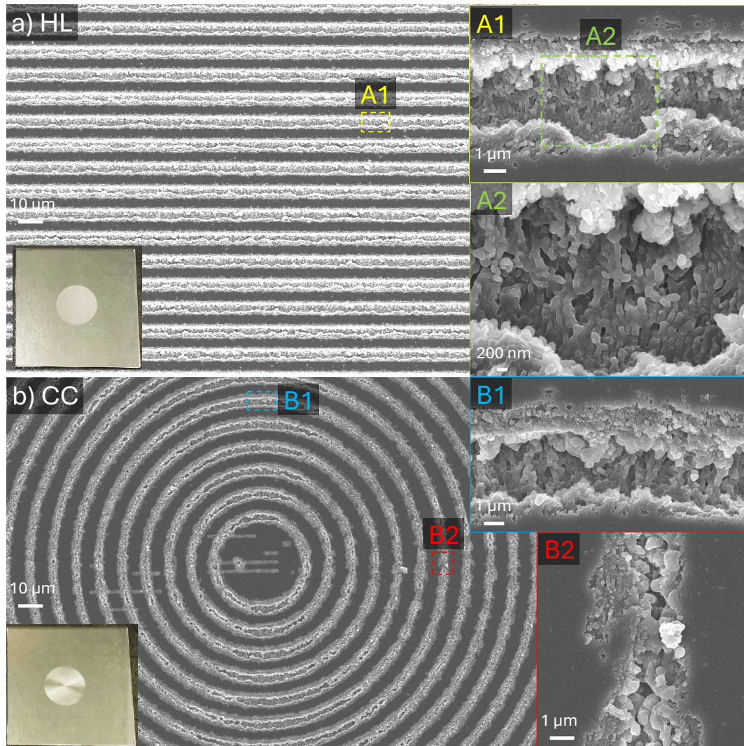
Figure 4. Back-side ablation of \text{Al}_2\text{O}_3 . SEM images of large-area pattern fabrication with a diameter of 0.5 cm on 1.5 \times 1.5 \text{ cm}^2 sapphire chips ablated by 515 nm/230 fs/200 kHz Gaussian beam, pulse fluence F_p = 20.40 \text{ J/cm}^2 (pulse average intensity I_p = F_p/t_p = 88.7 \text{ TW/cm}^2 ), number of passes N_p = 10 . (a) The fabricated area is filled with horizontal hatching (HL). (b) The same fabrication condition for the concentric circle (CC) pattern; both HL and CC patterns have the grating period \Lambda = 10 \mu\text{m} ; the insets (left-bottom) are optical pictures of the fabricated sapphire chips.
