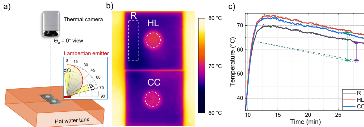
Figure 6. (a) Temperature measurement setup: sapphire samples were placed in the centre of a hot water tank (polypropylene), with a thermal camera (Optris PI 160, Germany) positioned above (azimuth \theta_a = 0^\circ ) the sample to capture temperature data. Inset shows an emissivity angular diagram for the Lambertian source I_0 \cos \theta_a , d\Omega is the solid angle wedge into which the black body source emits (see discussion in the text). (b) Thermal image captured by the camera, showing monitored areas with the horizontal line (HL) and concentric circle (CC) patterns, as well as a non-patterned sapphire surface as a reference (R). (c) Cooling transients: temperature change from the monitored areas.
