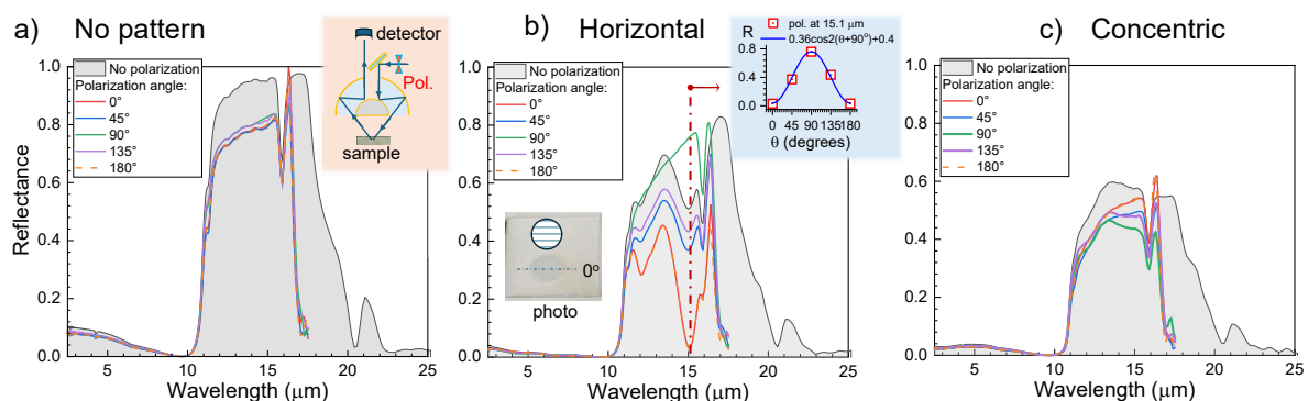
Figure A1. Reflectance FTIR spectra R(\lambda) from c-plane \text{Al}_2\text{O}_3 without laser patterned gratings as well as from 0.5-mm-diameter \Lambda = 10 \mu\text{m} period linear and circular gratings in (a,b,c), respectively, at different polarisation angles \theta ; inset in (a) shows the geometry of measurements. The top-inset in (b) shows the angular dependence of R vs. \theta angle of linearly polarised incident IR radiation from a thermal IR source (Globar TM ) at \lambda = 15.1 \mu\text{m} . Numerical aperture of Cassegranian objective lens NA = 0.5 , which defined focal diameter d_s = 1.22\lambda/NA \approx 45.8 \mu\text{m} at \lambda = 15 \mu\text{m} , i.e., d_s \approx 4\lambda . Note: R spectra are shown only up to a wavelength of 17.5 \mu\text{m} , as the mesh polariser introduces significant noise beyond this range, making the spectrum unreliable due to its inherent design limitations.
