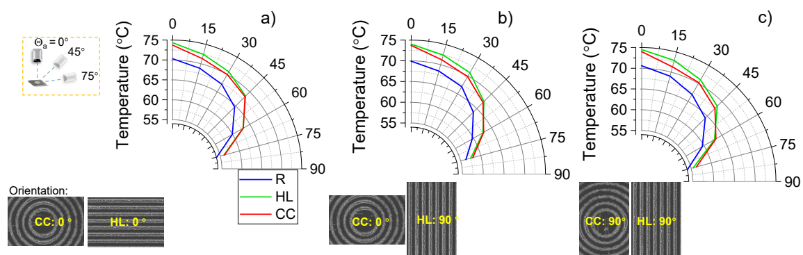
Figure 7. Lambertian-like emitter surfaces. Measurement of temperature of sapphire samples at the azimuthal observation angles from \theta_a = 0^\circ to 75^\circ angle at \phi = 0^\circ and 90^\circ orientations (orientation in the plane of the sample). (a) HL at 0^\circ and CC at 0^\circ orientation. (b) HL at 90^\circ and CC at 0^\circ orientation. (c) HL at 90^\circ and CC at 90^\circ orientation. The setup is the same as Figure 6 to record the temperature at different angles like the insert shown in (a).
