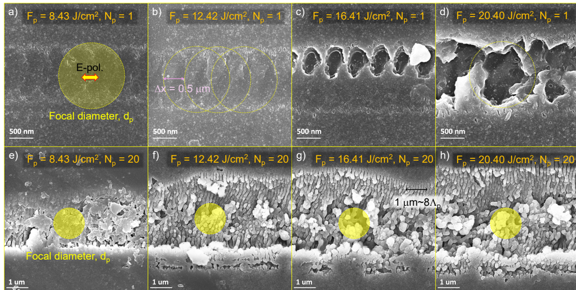
Figure 2. Back-side ablation of \text{Al}_2\text{O}_3 . SEM images of grooves on sapphire ablated by 515 nm/230 fs/200 kHz Gaussian beam with different pulse fluence F_p and number of passes N_p ; F_p increased from the left 8.43 J/cm 2 to the right 20.40 J/cm 2 ; (a), (b), (c) and (d) show single-pass ablation while (e), (f), (g) and (h) show 20-pass ablation. Focusing with NA = 0.45 objective lens; the focal spot d_p \approx 1.22\lambda/NA = 1.4 \mu\text{m} ; number of pulses per focal diameter d_p is N = d_p/\Delta x \approx 3 at constant pulse density 2000 \text{ mm}^{-1} . Linear polarisation of the writing beam was aligned with the scan direction (horizontal).
