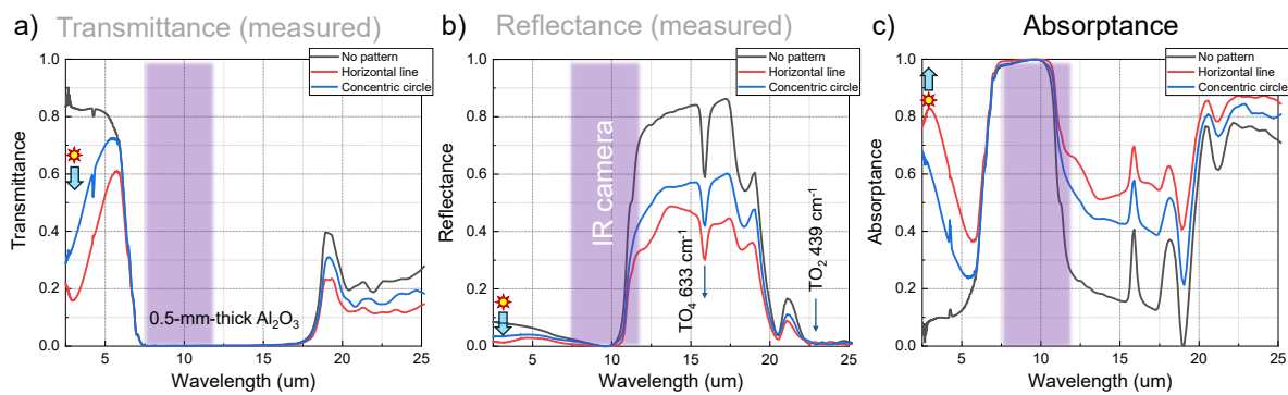
Figure 5. Laboratory-based FTIR spectra of the horizontal line (HL) and concentric circular (CC) grating structures (Figure 4), collected using a Bruker Vertex spectrometer with an internal Global TM IR source (unpolarised). Experimentally measured reflectance R (normalized to Au mirror) and transmittance T . Then the absorbance A is calculated from the energy conservation A + R + T = 1 . Changes of R , T (measured), and A (calculated) at 7.5\text{--}13 \mu\text{m} caused emittance changes when imaged by IR camera (Figure 6); highlighted by a rectangular block. A star marker with an arrow shows a tendency of increased A at \sim 4.3 \mu\text{m} as compared with unstructures Al_2O_3 .
