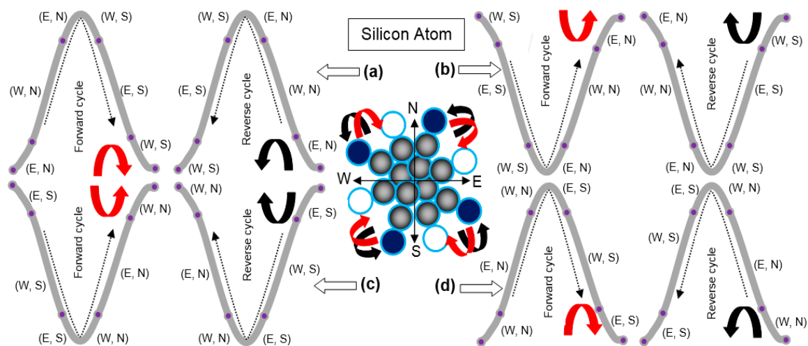
Figure 5. Electrons of four quadrants denoted by (a), (b), (c), and (d) deal with the east (E), west (W), north (N), and south (S) forces along the relevant poles while executing confined inter-state dynamics in forward (red-colored round arrows) and reverse (black colored round arrows) cycles.
