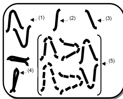
Figure 1. (1) Unit photons shape like Gaussian distribution having turned ends, (2) division of unit photon in shape like integral symbol and (3) division of unit photon in shape like opposite integral symbol, (4) merged energy of unit photons and (5) broken pieces of unit photons.
