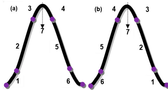
Figure 4. Sections of the unit photon generated by electron dynamics of silicon atom in (a) forwarding and (b) reverse cycles; (7) maximum limit point connecting left and right half-cycles.
