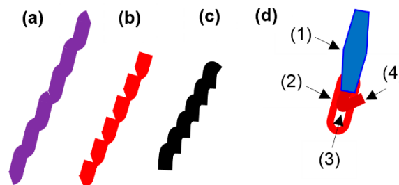
Figure 6. Overt photon of connected (a) integral symbols, (b) tick symbols, (c) L -like symbols, and (d) shaping force and energy along the trajectory; (1) electron dynamics, (2) shaping energy, (3) shaping force, (4) the removed red-colored energy region showing the force in white color.
