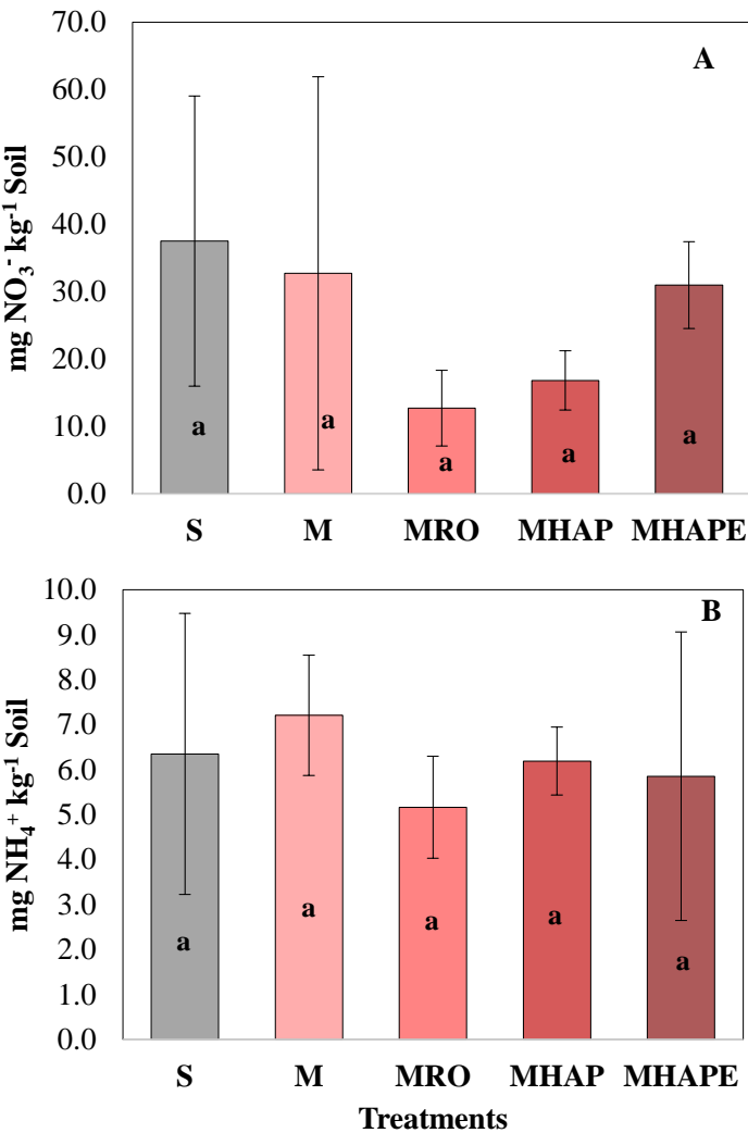
Figure 5. The effect of treatments on soybean soil nitrate-N (A) and ammonium-N (B) concentrations. The mean was calculated for n=4 ; the vertical bar represents the standard deviation of the mean. Here, S = soil control; M = manure control; MRO = manure+red oak biochar; MHAP = manure+highly alkaline porous biochar; MHAPE = manure+corn feedstock autothermal porous Fe-engineered biochar. The means were not statistically different at p<0.05 level.
