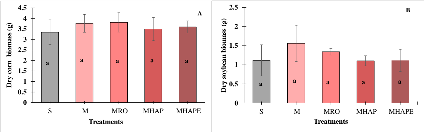
Figure 7. The effect of treatments on the biomass yield for corn (A) and soybean (B) biomass. Each bar represents an average of 4 replications \pm standard deviation. S = soil control; M = manure control; MRO = manure + red oak biochar; MHAP = manure + highly alkaline porous biochar; MHAPE = manure + corn feedstock autothermal porous Fe- engineered biochar. Different letters show the treatments that are statistically different at p < 0.05 level.
