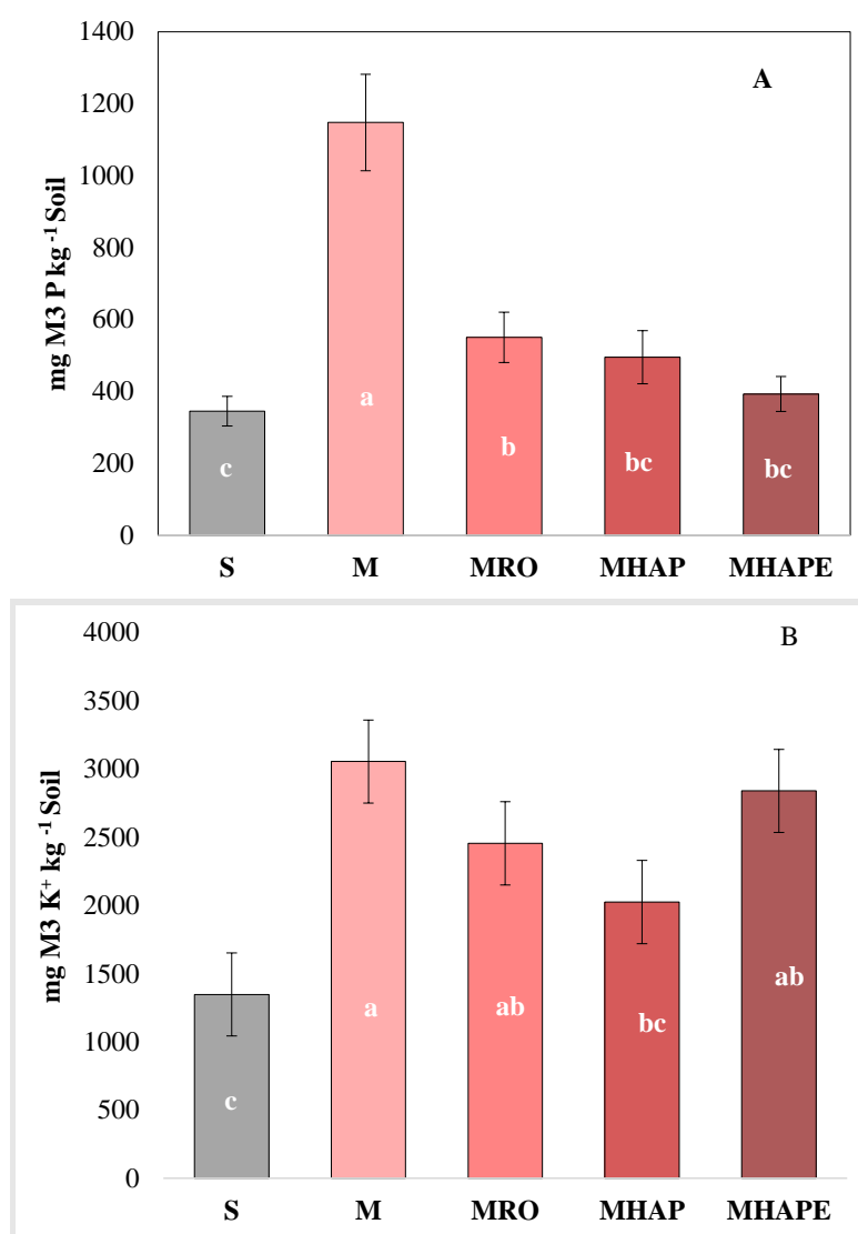
Figure 4. The effect of treatments on Mehlich3 (M3) extractable corn soil P (A) and K (B) concentrations. The mean was calculated for n=4 ; the vertical bar represents the standard deviation of the mean. Here, S = soil control; M = manure control; MRO = manure+red oak biochar; MHAP = manure+corn feedstock autothermal porous Fe-engineered biochar; MHAPE = manure+corn feedstock autothermal porous Fe-engineered biochar. Different letters show the treatments that are statistically different at p<0.05 level.
