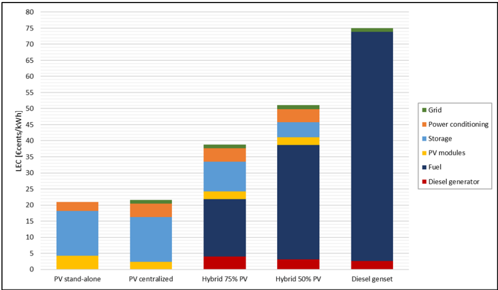
Figure 21. LEC comparison of different types of power plant and contribution of each subsystem cost considering the ideal case and total centralization.
