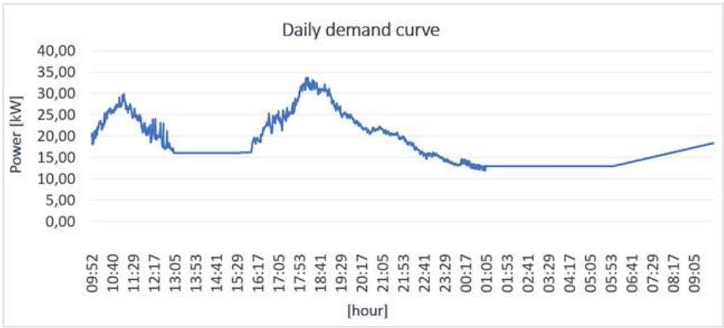
Figure 6. Daily demand curve of Guasasa obtained from network analysis [79].
