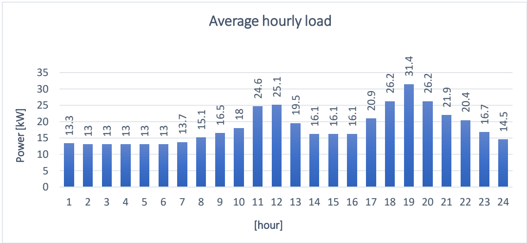
Figure 7. Average hourly energy load for the community of Guasasa [73].
