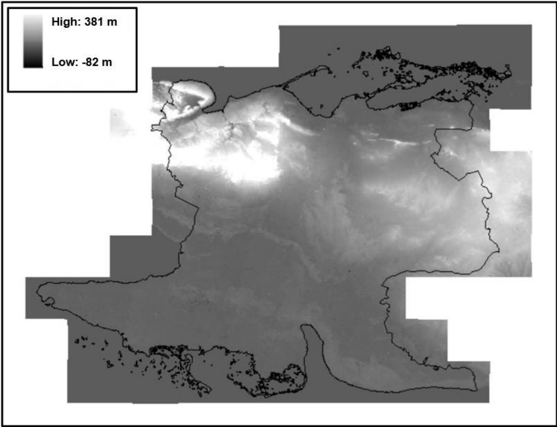
Figure 10. DEM including the province of Matanzas. (Source: JAXA [84]).
