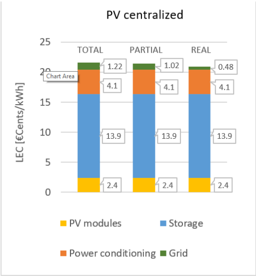
Figure 14. Cost contribution of each subsystem to the total LEC of a PV centralized system for the three cases tested.
