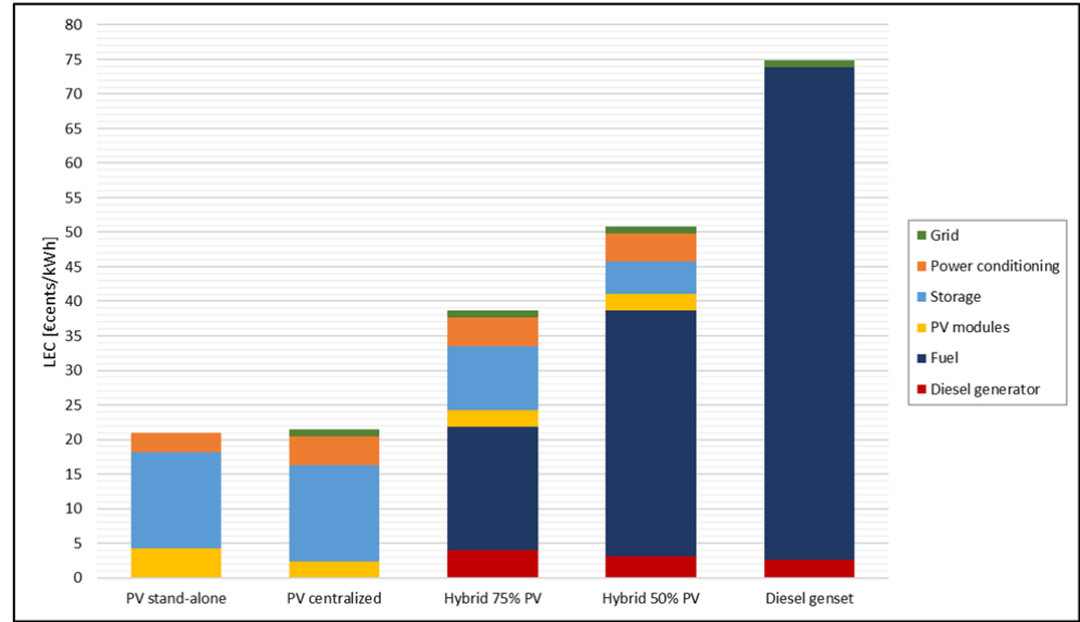
Figure 22. LEC comparison of different types of power plant and contribution of each subsystem cost considering the ideal case and partial centralization.
