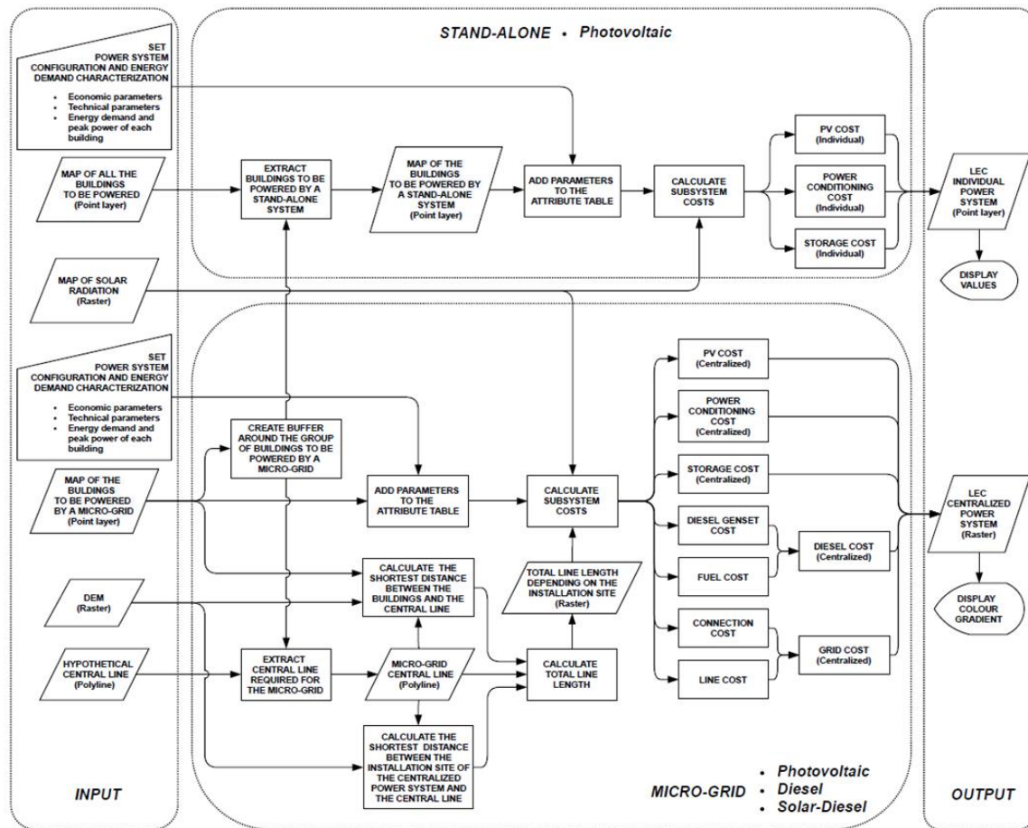
Figure 1. IntiGIS-local flowchart.
