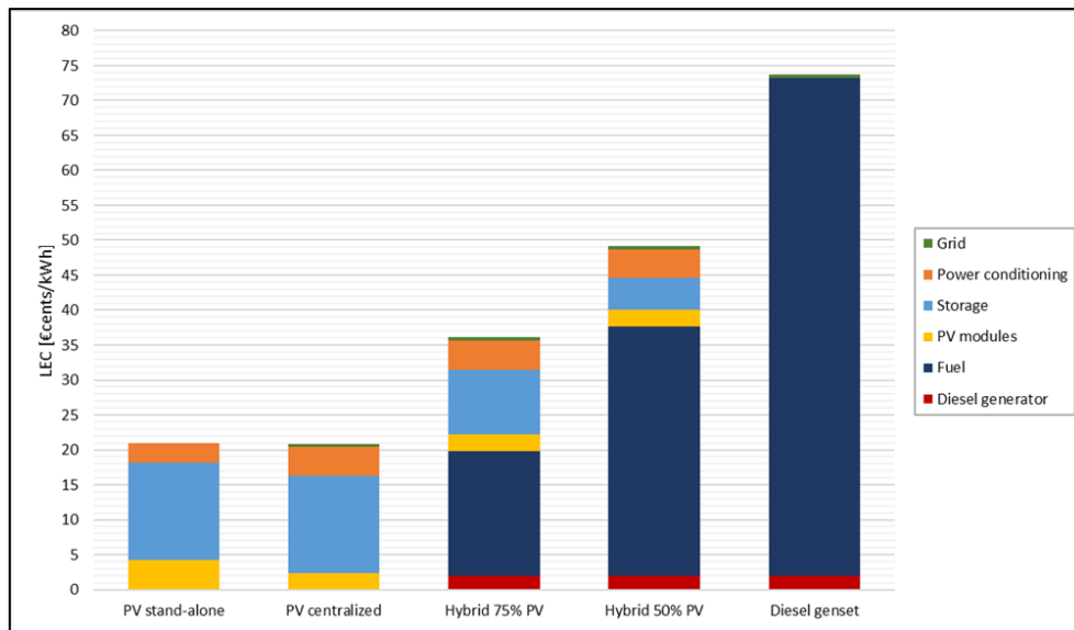
Figure 23. LEC comparison of different types of power plant and contribution of each subsystem cost considering the real case.
