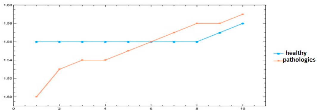
Figure 8. Dimension fractal average of the retinas of patient healthy of patient healthy reported by Santiago - Cortes and collaborators (25) and patient with pathologies reported in this work.
