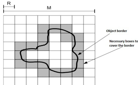
Figure 4. Method BC. In this case they are necessary 20 boxes to cover the whole border of the object.
