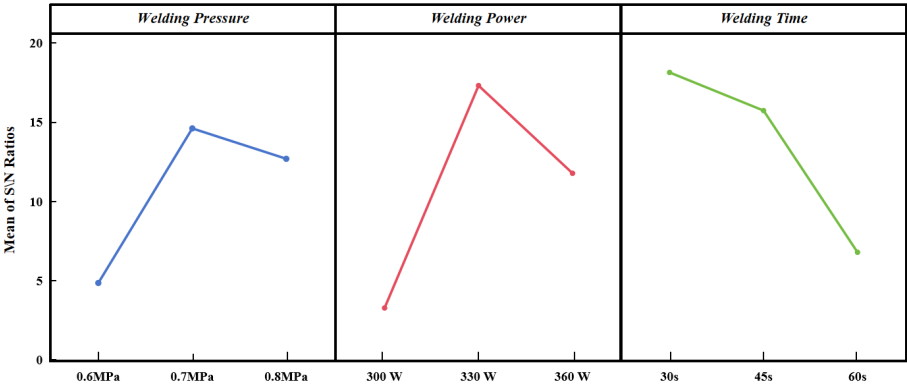
Figure 3. Main effect diagram of single lap shear strength of CF/EP welded joints.
