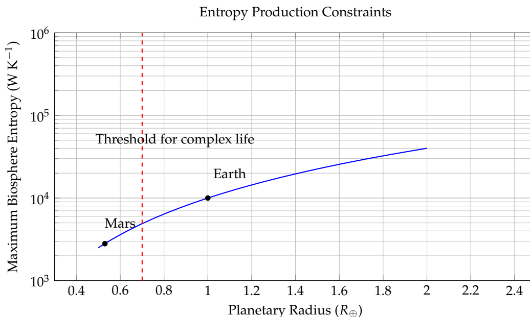
Figure 2. Entropy constraints on complex biospheres. The curve shows the maximum biospheric entropy production S_{\max} \sim R^2 , as a function of planetary radius. A vertical red dashed line marks the critical radius threshold R_{\min} = 0.7 R_{\oplus} , below which a planet cannot generate sufficient entropy to sustain complex life. Earth lies well above this threshold, while Mars falls below it.
