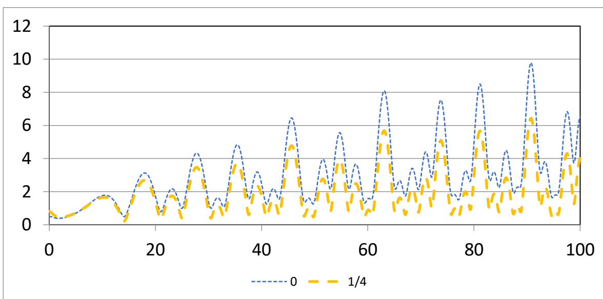
Figure 4. Plots of |\zeta(\sigma + it)| with \sigma = \{0, \frac{1}{4}\} and 0 \leq t \leq 100 .
