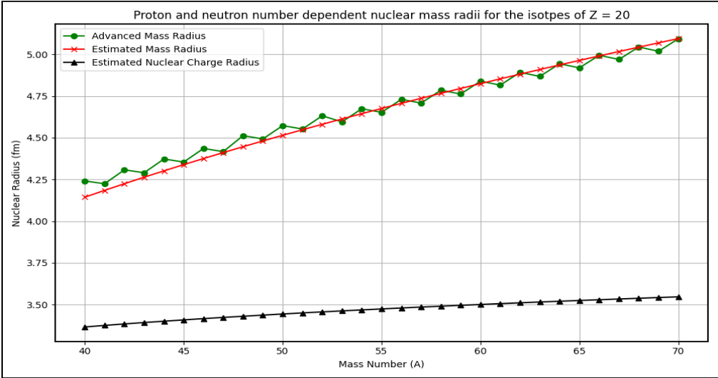
Figure 4. Estimated mass radii of isotopes of Z=20 based on cubic root of proton and neutron numbers.
