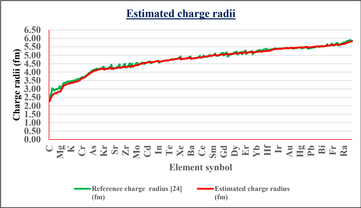
Figure 9. Estimated charge radii of Z= (6 to 96) based on cubic root of proton and neutron numbers.
