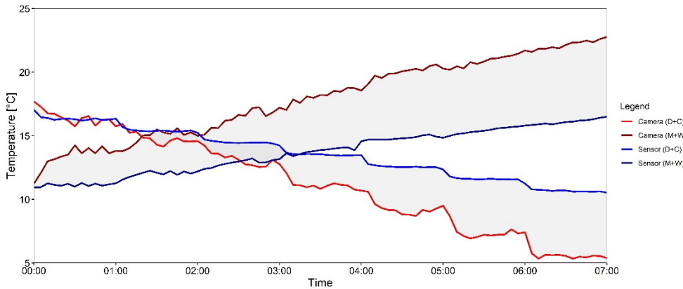
Figure 4. Temperature measurements on the calibration plate by the thermal camera (red) and the surface temperature sensors (blue) for two of the five experiemental conditions (Dry + Cooling and Moist + Warming).
