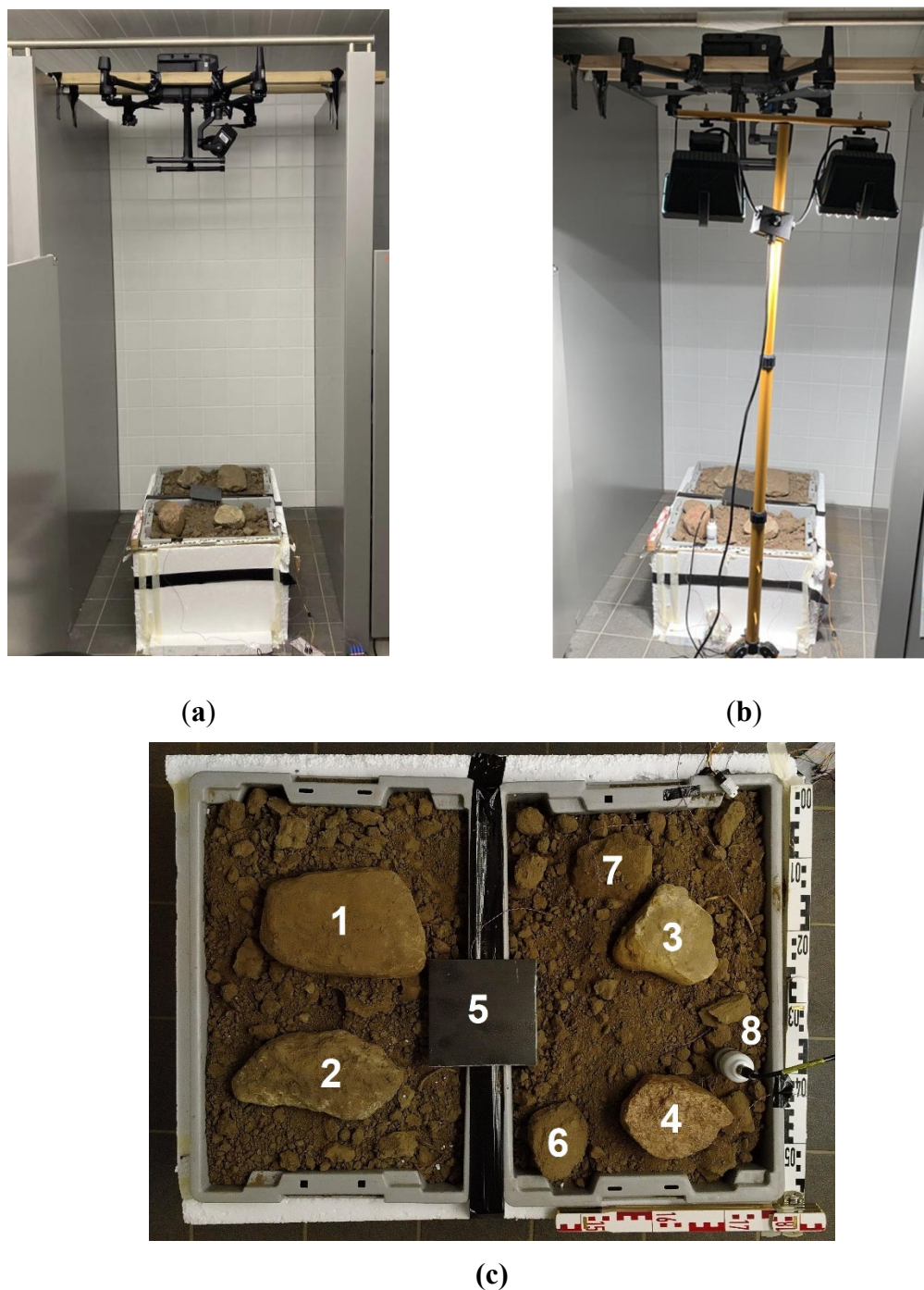
Figure 1. Experimental setup in the climate chamber under controlled conditions. (a) Setup without artificial light; (b) setup with artificial light, (c) the soil containers with numbers 1 to 4 indicating stones, number 5 referring to the calibration plate, numbers 6 to 7 pointing at a soil clods, and number 8 marking the soil moisture sensor.
