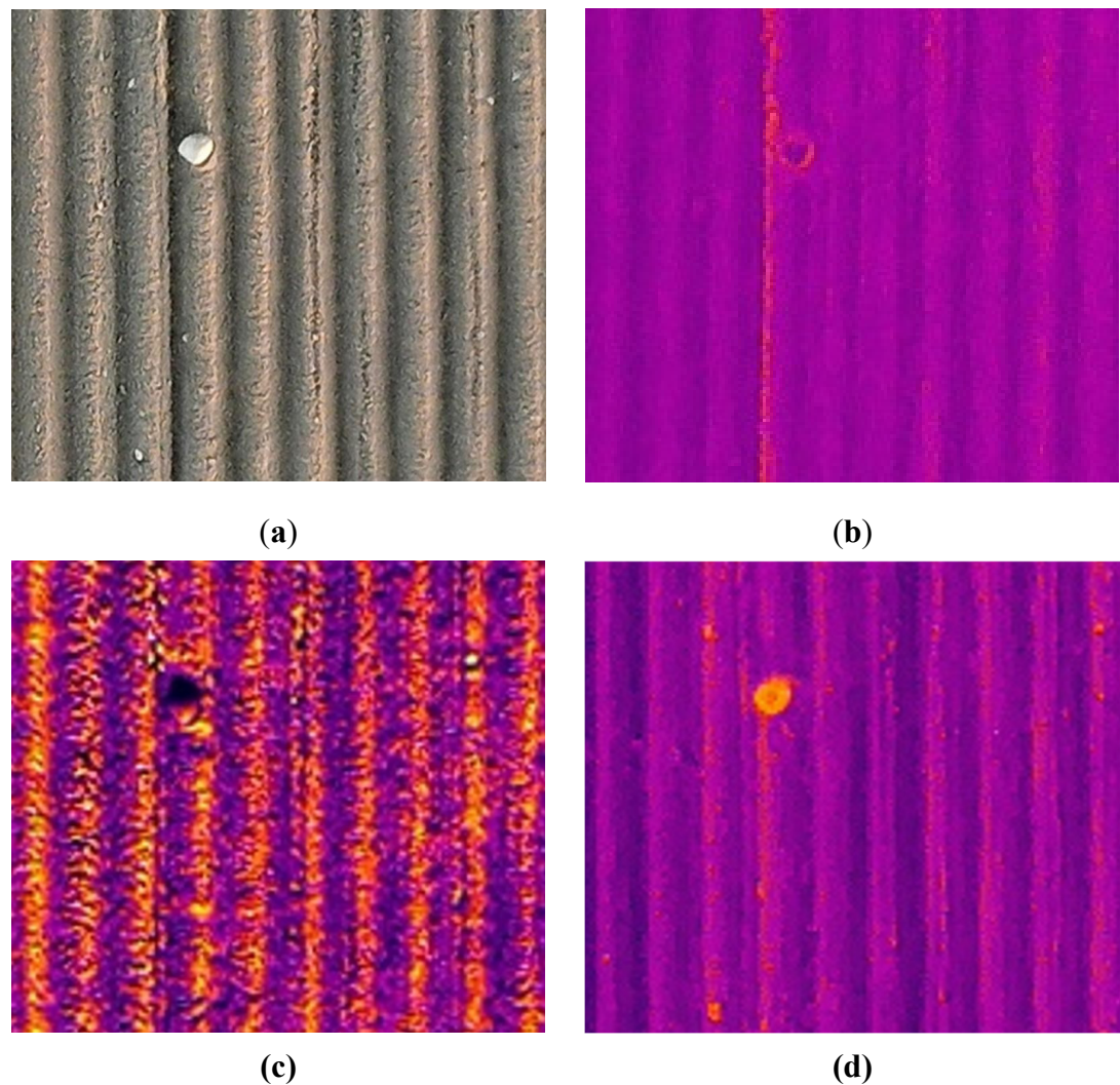
Figure 3. a) RGB image, b) thermal image in the morning at 7:06 a.m., c) thermal image around midday at 11:12 a.m. and d) thermal image in the evening at 20:28 p.m. of a stone in the field. Temperature scales are not displayed, as the thermal range varies between images and the focus lies on the relative differences between the stone and the surrounding soil.
