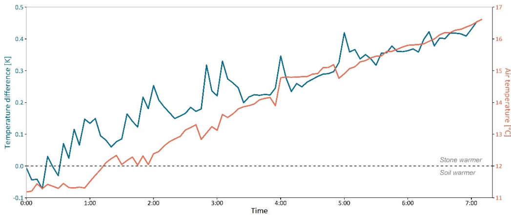
Figure 6. Temperature difference between the stones and the soil for moist soil conditions (blue solid) measured by the thermal camera and surrounding air temperature (red) during the moist and warming (M+W) experimental conditions.
