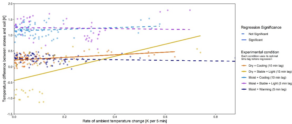
Figure 9. Relationship between the absolute rate of ambient temperature change and the temperature difference between stones and soil across five experimental conditions. Each condition is analyzed using the time lag that produced the most pronounced effect in the regression, as specified in the legend. Solid lines represent statistically significant regressions ( p < 0.05 ), while dashed lines indicate non-significant relationships.
