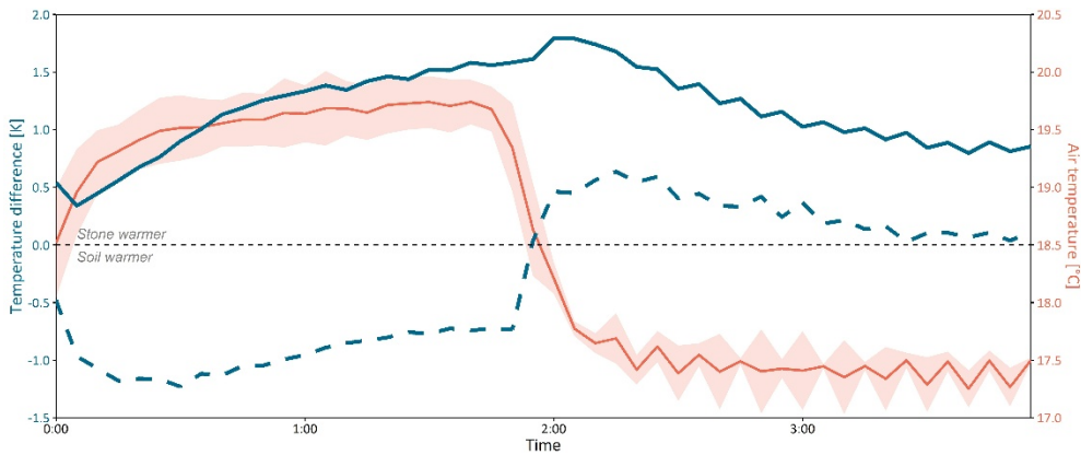
Figure 7. Temperature difference between the stones and the soil for moist soil conditions (blue solid) and dry soil conditions (blue dashed) measured by the thermal camera and mean surrounding air temperature (red) during the M+S+L and D+S+L experimental conditions.
