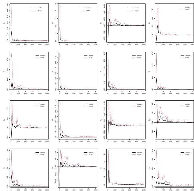
Figure A2. Potential scale reduction factor (PSRF) against iterations for all coefficients under the deviation coding strategy. Note: The black line denotes the PSRF and the red dotted line indicates the upper limit of the 95% confidence interval for the PSRF.
