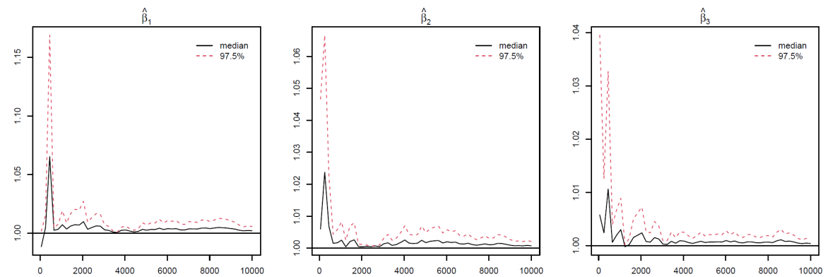
Figure 3. Potential scale reduction factor (PSRF) against iterations for the three coefficients associated with Race under dummy coding. The black line shows the PSRF, and the red dotted line marks the upper limit of the 95% confidence interval.
