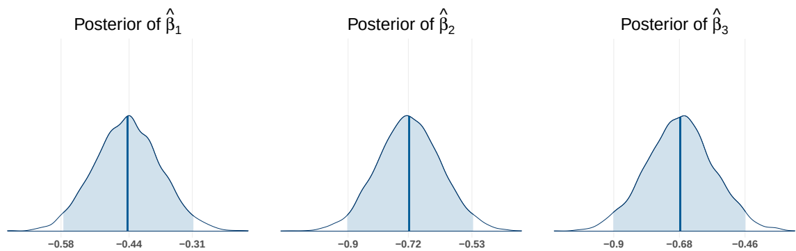
Figure 2. Posterior distributions of the regression coefficients associated with Race under dummy coding. The grey dashed lines denote the lower and upper bounds of the 95% credible interval, and the blue solid line represents the median.
