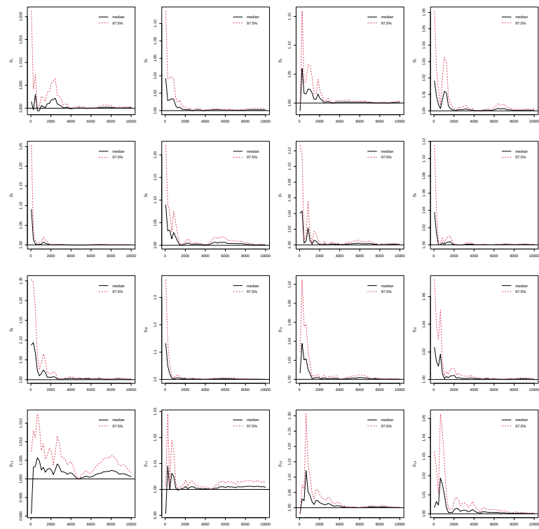
Figure A3. Potential scale reduction factor (PSRF) against iterations for all coefficients under the sequential coding strategy. Note: The black line denotes the PSRF and the red dotted line indicates the upper limit of the 95% confidence interval for the PSRF.
