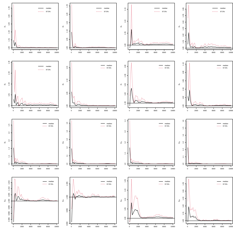
Figure A1. Potential scale reduction factor (PSRF) against iterations for all coefficients under the dummy coding strategy. Note: The black line denotes the PSRF and the red dotted line indicates the upper limit of the 95% confidence interval for the PSRF.
