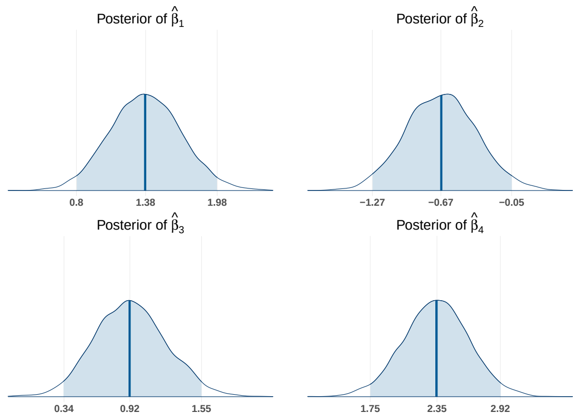
Figure 1. Posterior distributions of \beta_1 to \beta_4 for the simulated data. The grey dashed lines denote the lower and upper bounds of the 95% credible interval, and the blue solid line represents the median.
