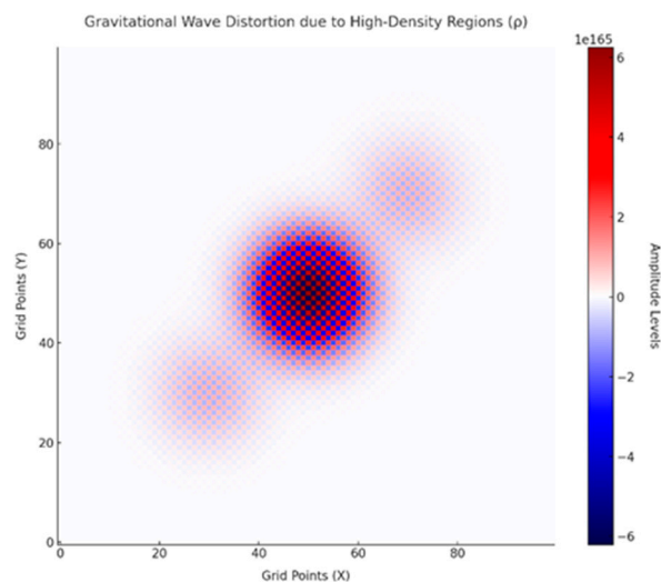
Figure A.1.1.3. Visualization of gravitational wave distortions caused by high-density quantum informational regions ( \rho > \rho_{\text{critical}} ). The wave amplitude is represented using a seismic colormap, with red and blue indicating positive and negative wave amplitude.
