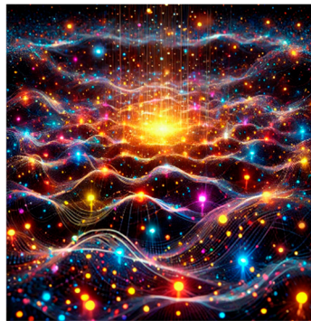
Figure 2. Multicolored Dots—A visualization of quantile distributions and their dynamic interactions within the PIF. The multicolored flows represent the emergence of forces (e.g., electromagnetic, gravitational) and spacetime curvature from quantum informational density ( \rho ).
