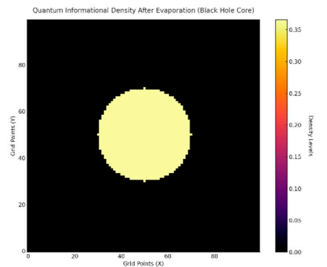
Figure B.1.3.1. Visualization of quantum informational density ( \rho ) in the black hole core after 100 timesteps.
