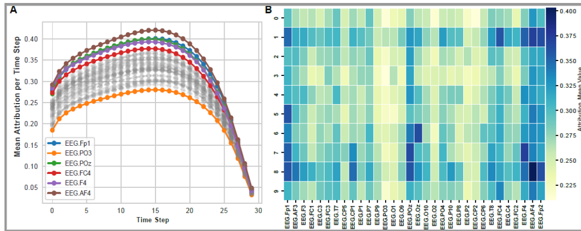
Figure 2. Visualization of attribution scores. A) Line plot showing average attribution scores across time steps in EEG data. B) Heatmap showing average attribution of for each EEG channel and each stimuli type (images of handwritten numbers from 0 to 9).
