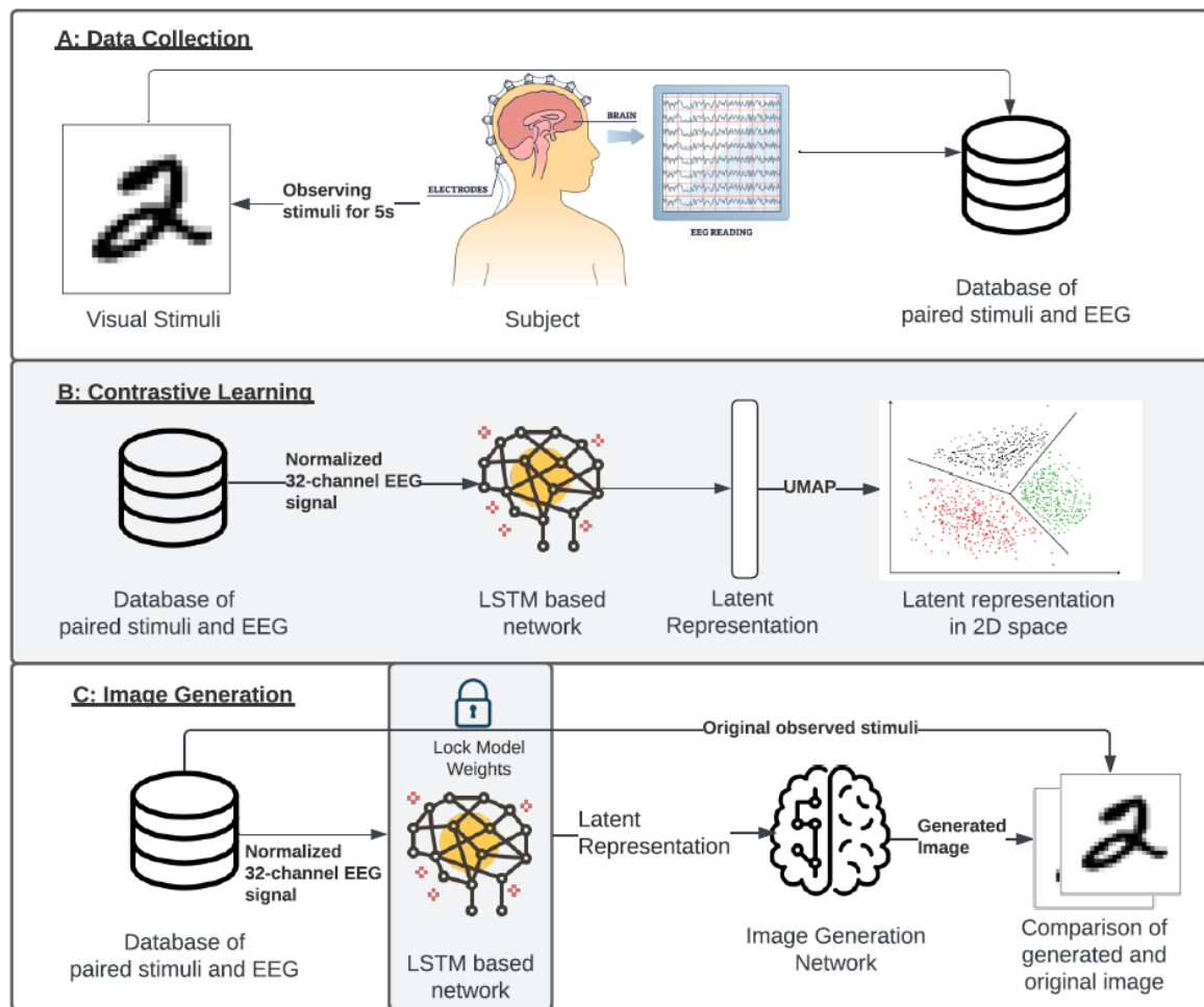
Figure 1. Study overview. Figure showing the study overview. A) Data Collection: EEG Data was collected while subjects observed the stimuli (image). Paired stimuli (image) and EEG data for each subject were stored in a database for further analysis. B) Each sample contained 32 channels, which were normalized based on the subjects' baseline measurements (closed eyes). The data was then fed into an LSTM-based network while employing contrastive loss. This resulted in a latent representation of the EEG signal. C) Extracted latent representations served as input for an image generator, generating images for comparison against the original stimuli (ground truth image).
