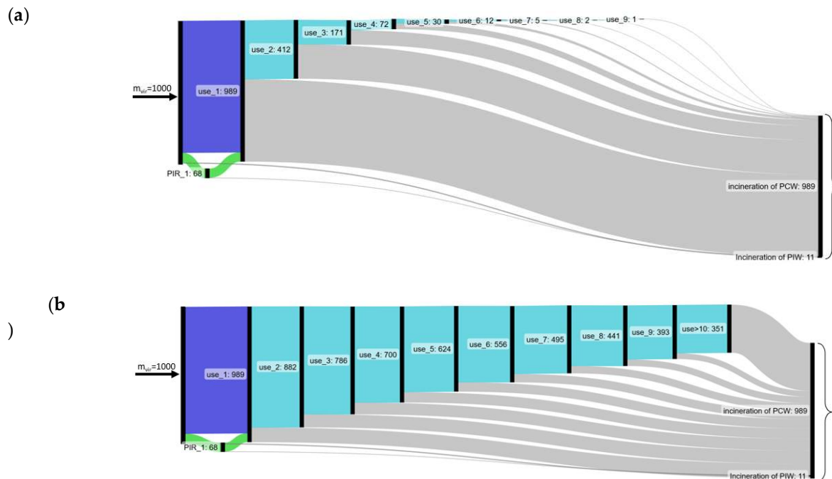
Figure 5. Sankey diagram of 1 kg of virgin PP input up to 10 th use of a material including contributions from virgin (dark blue), PIR (green) and PCR (light blue): (a) Realistic scenario; (b) Ideal scenario.
