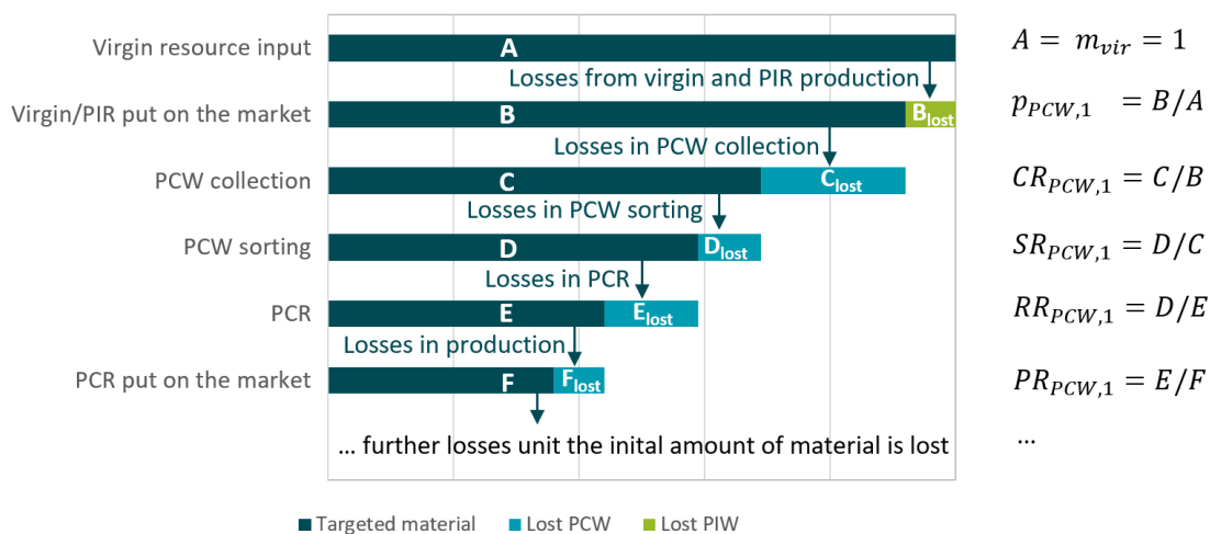
Figure 1. Simplified collection, sorting and recycling scheme of targeted PCW material to be recycled.
