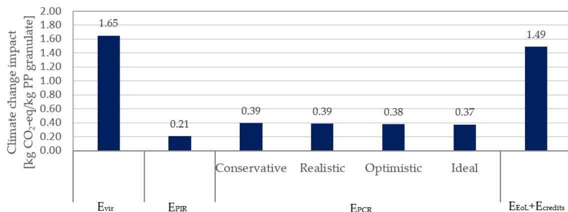
Figure 7. CC impact per kg of PP from virgin granulate provision ( E_{vir} ), PIR ( E_{PIR} ), PCR ( E_{PCR} ) as well as the aggregated burdens and benefits of incineration and energy recovery of 1 kg PP ( E_{EoL}+E_{credits} ).
