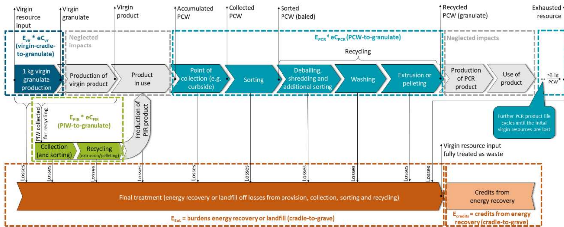
Figure 2. Entire path of 1 kg of virgin resource input used in multiple product systems until the material is lost including the environmental impacts associated with the material.
