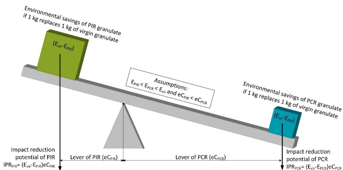
Figure 3. Schematic example of the IRP of PIR and PCR if PIR granulate causes lower environmental impacts than PCR granulate ( E_{PIR} < E_{PCR} ) and both have lower impacts than virgin granulate provision ( E_{vir} ).
