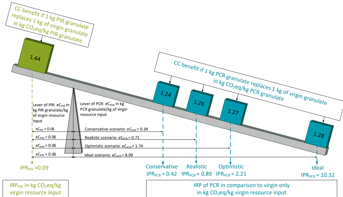
Figure 8. The IRP of PP PIR compared to PP PCR.
