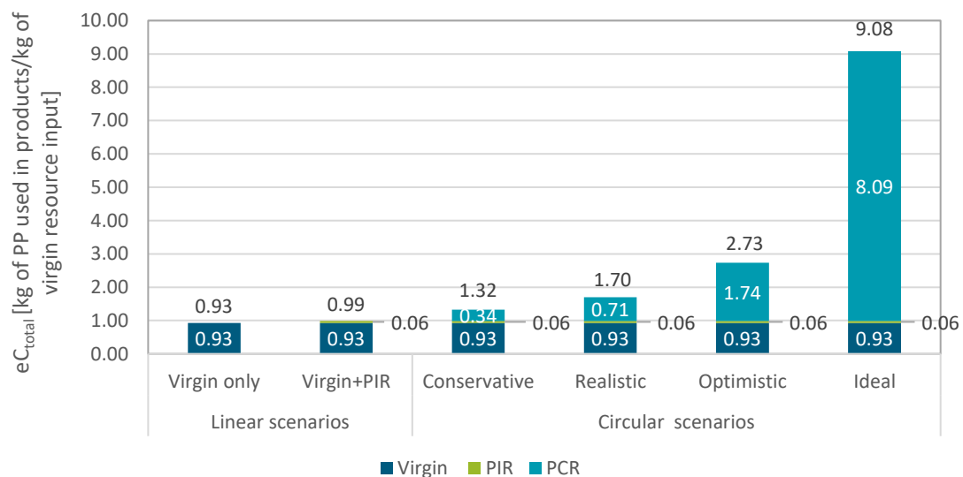
Figure 4. The eC of PP for the linear and circular scenarios.
