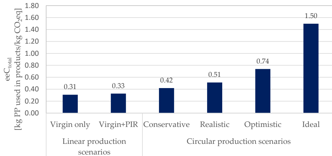
Figure 6. The eeC calculated for the linear and circular scenarios per CC impact.
