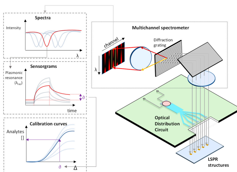
Figure 7. The optical reader concept, based on an optical distribution circuit and a multi-channel spectrometer.
