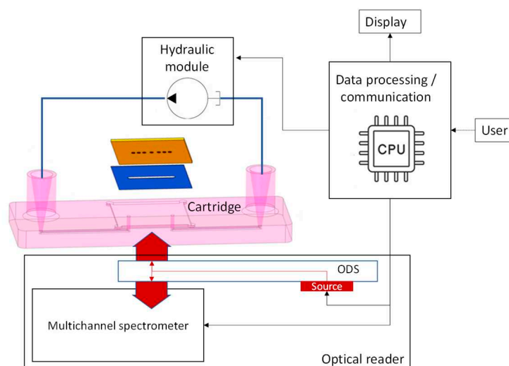
Figure 6. Reader instrument scheme, showing optical readout sub-system, hydraulic module and embedded processing and connectivity.
