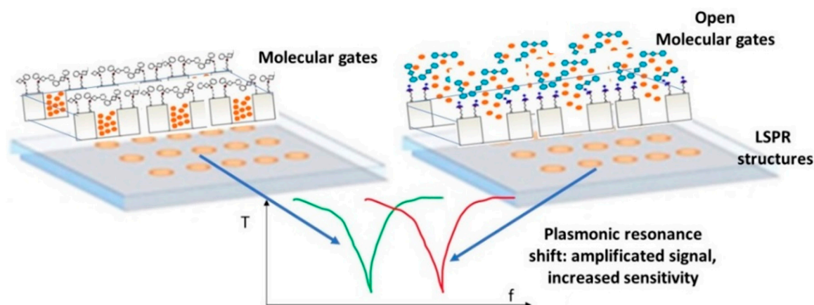
Figure 4. PHOTONGATE transduction based on LSPR structures.
