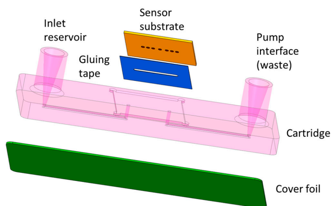
Figure 5. Schematics of the proposed PHOTONGATE cartridge.
