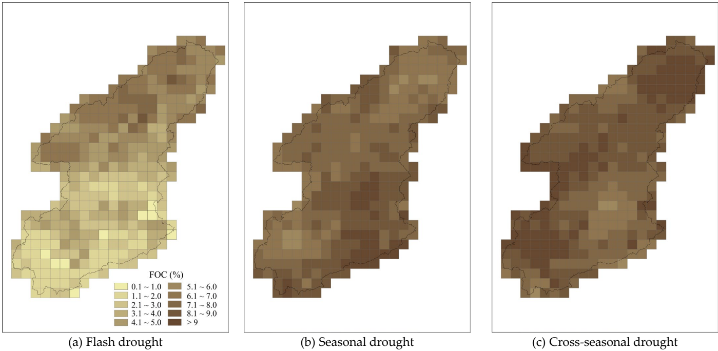
Figure 4. Spatial distribution of drought occurrence frequency in the Dongjiang River Basin.
