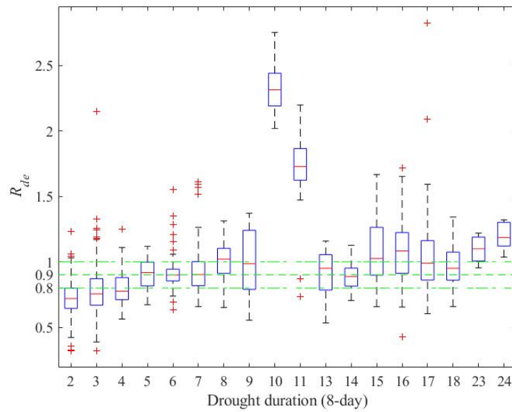
Figure 8. Relationship between flash drought duration and R_{de} in the Dongjiang River Basin.
