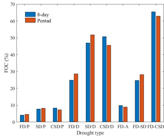
Figure 10. Comparison of the occurrence frequency of different types of droughts identified using the 8-day scale and the pentad scale. /P denotes the proportion of a specific drought type relative to all time units, and /D represents the proportion of a specific drought type relative to the total number of drought events.
