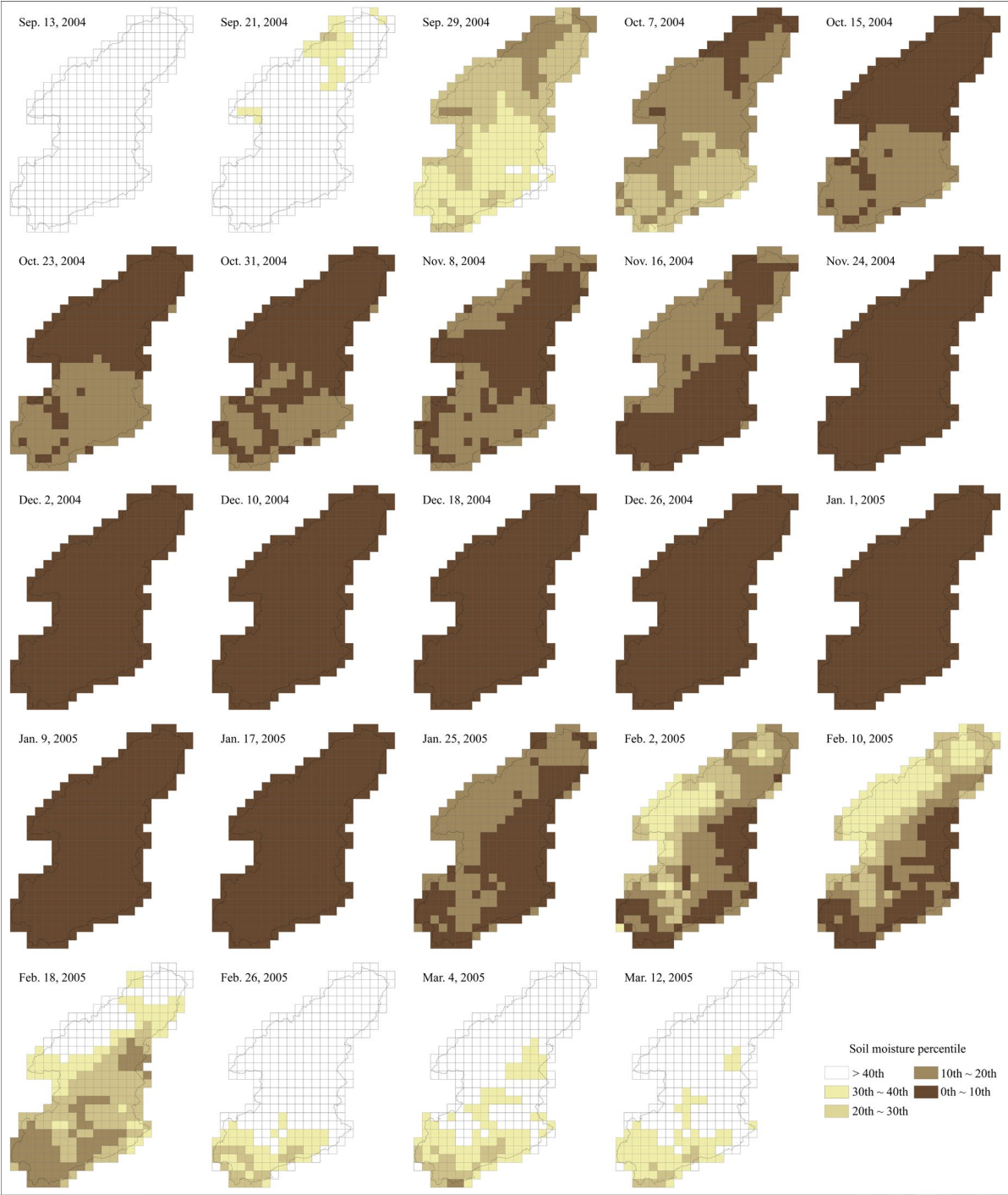
Figure 7. Spatial evolution of the 2004 drought event in the Dongjiang River Basin.
