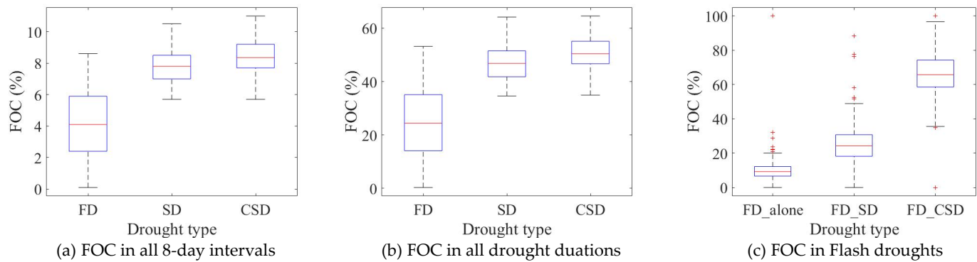
Figure 3. Statistical box plot of drought occurrence frequency in the Dongjiang River Basin.
