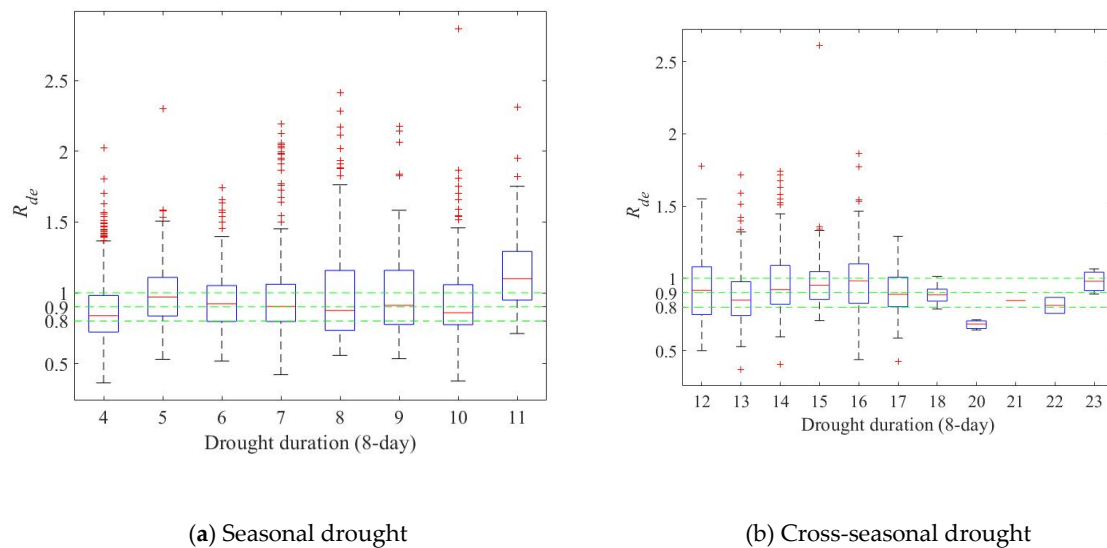
Figure 9. Relationship between drought duration and R_{de} for (a) seasonal drought and (b) cross-seasonal drought (evolved from non-flash drought) in the Dongjiang River Basin.
