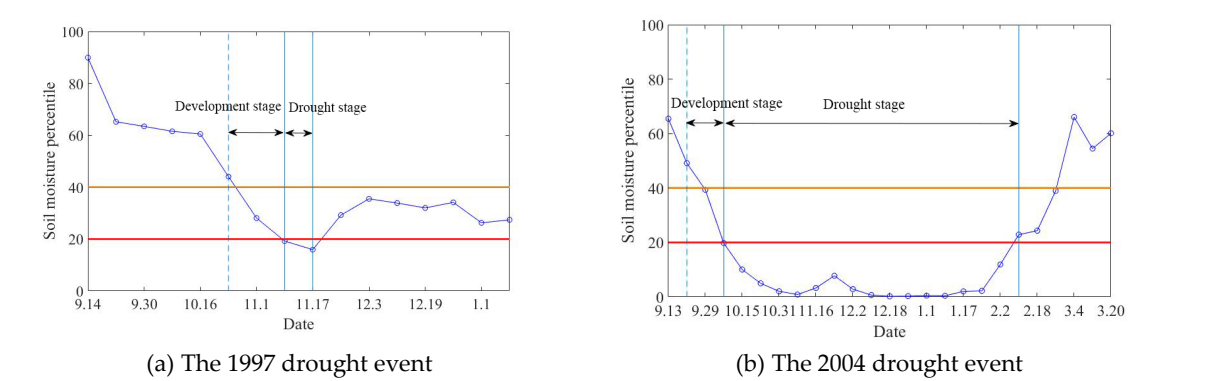
Figure 5. Temporal evolution of the two drought events in the Dongjiang River Basin in 1997 and 2004.
