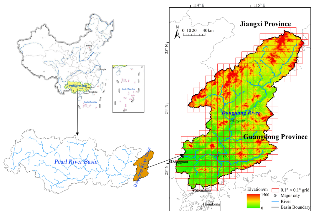
Figure 1. The location of Dongjiang River Basin.
