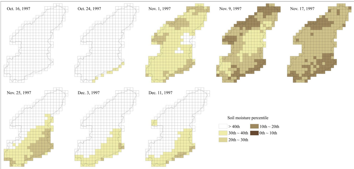
Figure 6. Spatial evolution of the 1997 drought event in the Dongjiang River Basin.
