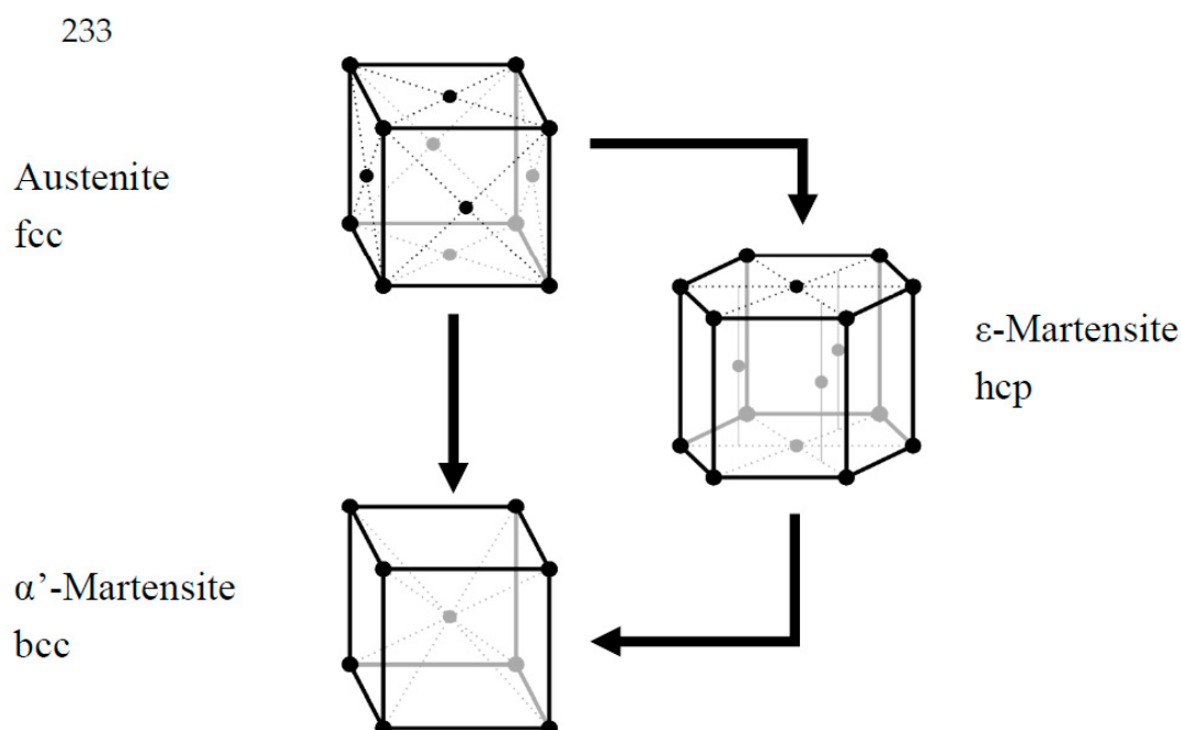
Figure 1. Hardening of metastable austenitic materials according to /Lin00/.
