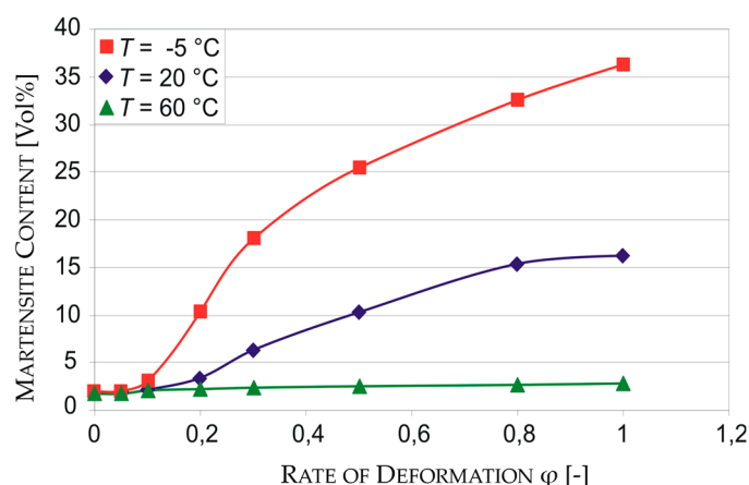
Figure 2. Martensite content in compression specimens (1.4301) as a function of forming temperature and degree of deformation (strain rate = 0.1 1/s).
