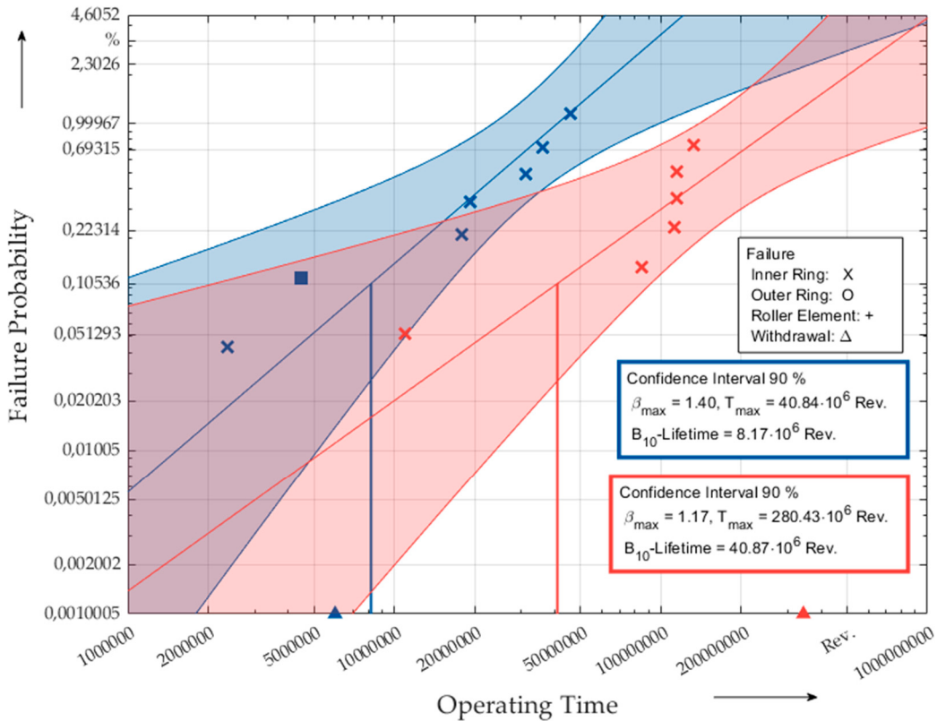
Figure 11. Weibull plot for industrial stainless-steel bearings in comparison to bearings with induced martensitic phase.
