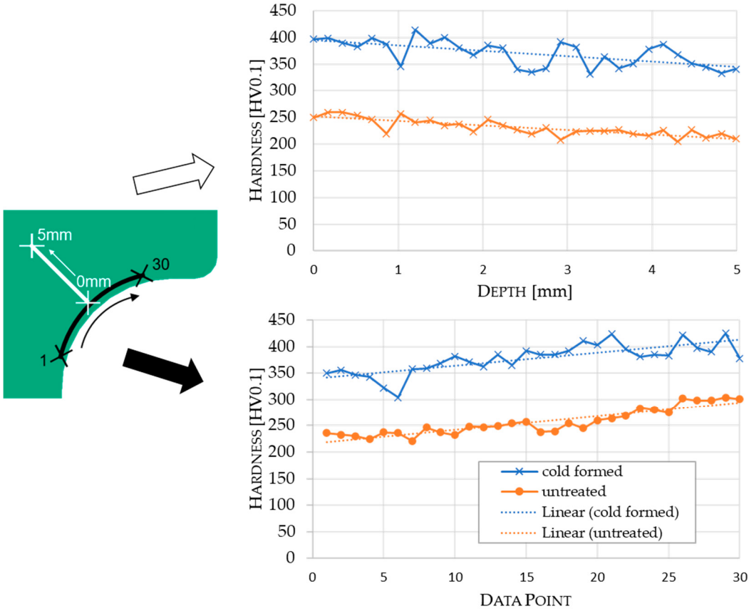
Figure 6. Hardness comparison between a cold formed (at -15°C) and a machined inner ring made from 1.4301.
