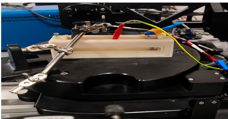
Figure 7. \text{TiO}_2 - \text{MoO}_3 -during-electrochromic-experiments by SE.
