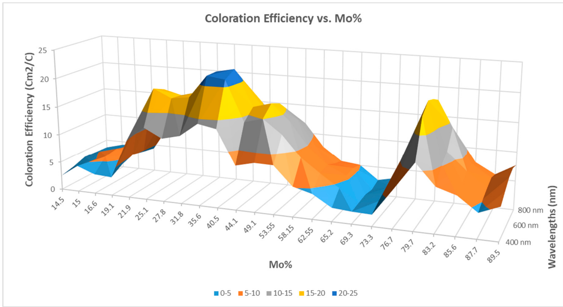
Figure 2. diagram of the Coloration Efficiency data of TiO 2 -MoO 3 . vs. Mo % for wavelengths from (400-800) nm visible spectral range.
