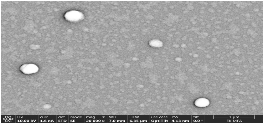
Figure 3. SEM micrograph from the TiO 2 -MoO 3 surface Ti-rich side.
