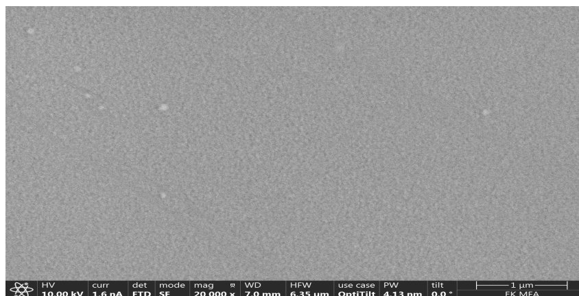
Figure 4. SEM micrograph from the \text{TiO}_2\text{-MoO}_3 surface Mo-rich side.
