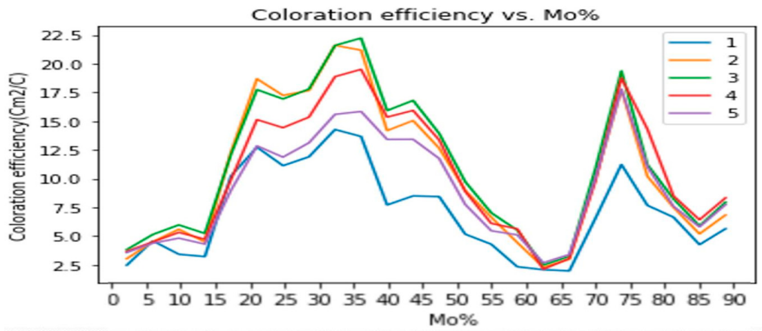
Figure 1. Coloration Efficiency of TiO 2 -MoO 3 . vs. Mo % for wavelengths from (400-800) nm by home-made software version 1.0 coded in Python version 3.11 language. (Individual color-coded curves represent different wavelengths: 1 – 400 nm, 2 – 500 nm, 3 – 600 nm, 4 – 700 nm, 5 – 800 nm).
