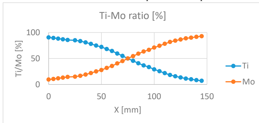
Figure 5. Ti/Mo ratio measured on the Si-probes by SEM-EDS.
