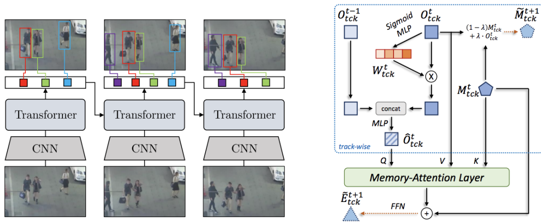
Figure 5. (Left) TrackFormer [49] introduces autoregressive queries to model detection and identity jointly. (Right) The Temporal Interaction Module in MeMOTR [50], which uses memory-based attention and gated updates for long-term identity propagation.
