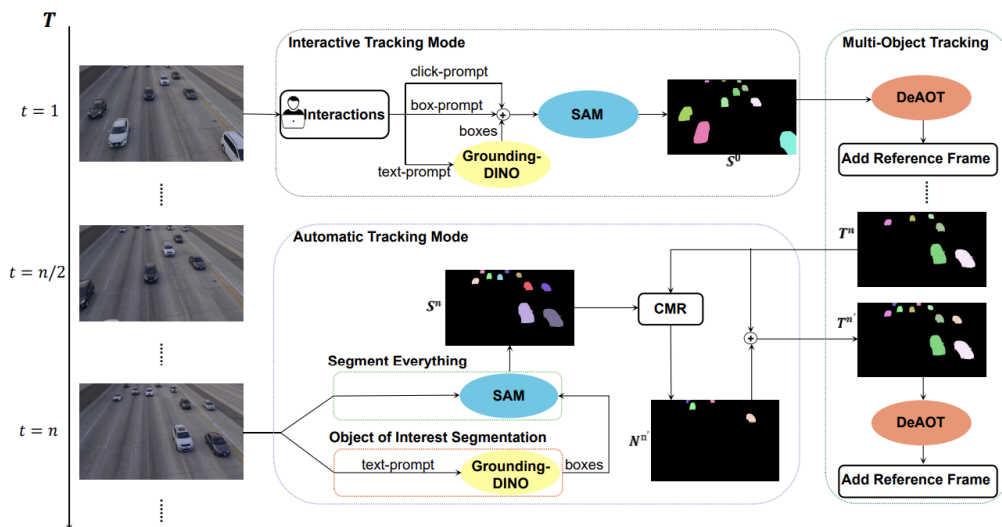
Figure 7. Overview of a SAM-based multi-object tracking framework [89]. The system supports both interactive and automatic tracking modes. In the interactive mode, object prompts (e.g., clicks, boxes, or text) are passed to Grounding-DINO and SAM to generate instance masks, which are tracked via DeAOT. In automatic mode, frames are processed by SAM with "segment everything" or object-specific prompts, and merged using context-aware reasoning (CMR). The resulting object masks are tracked using DeAOT with reference frame updates.
