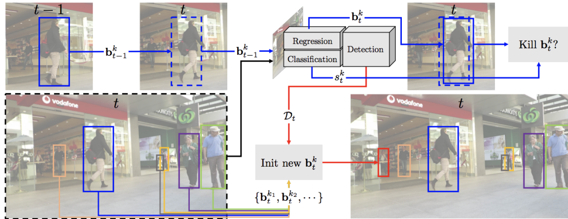
Figure 4. Overview of the Tracktor pipeline for multi-object tracking [35]. Regression aligns bounding boxes from frame t-1 to t , while classification scores determine termination. New detections are introduced when overlaps are low.
