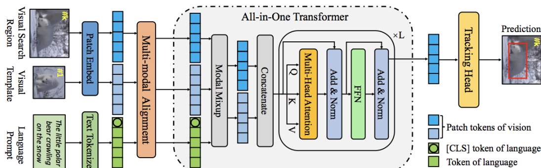
Figure 8. Overview of the All-in-One vision-language tracker [99]. The model unifies visual search region, visual template, and language prompts through multi-modal alignment. Features are embedded using separate vision and language encoders, followed by modal mixup and joint processing via a multi-head self-attention Transformer. The All-in-One Transformer encodes both modalities for tracking, and a shared tracking head predicts object locations in the target frame.
