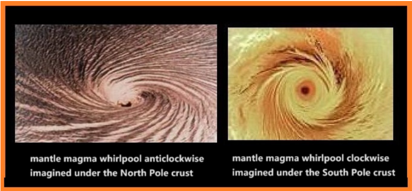
Figure 12. the mantle magma whirlpool imagined under the crust of North and South Pole.
