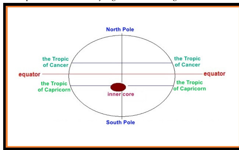
Figure 3. reasonable locating of the inner core of the planet Earth.
