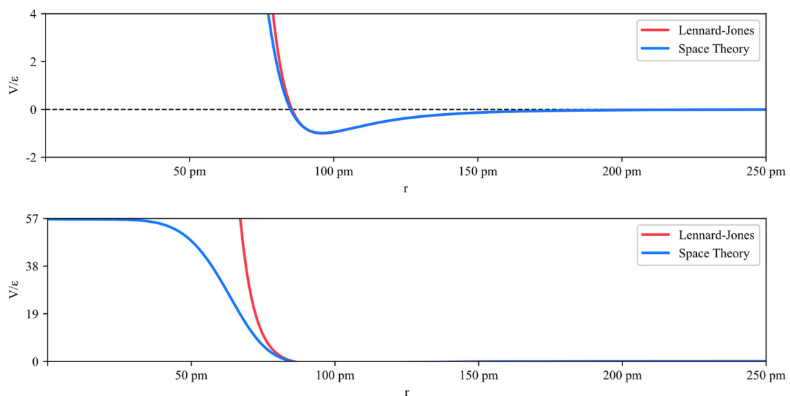
Figure 14. Lennard-Jones potential of a hydrogen bond.
