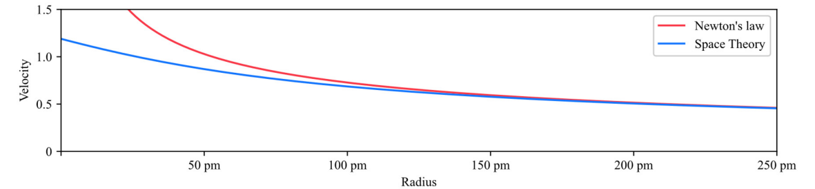
Figure 12. The orbital velocity of a Hydrogen atom.
