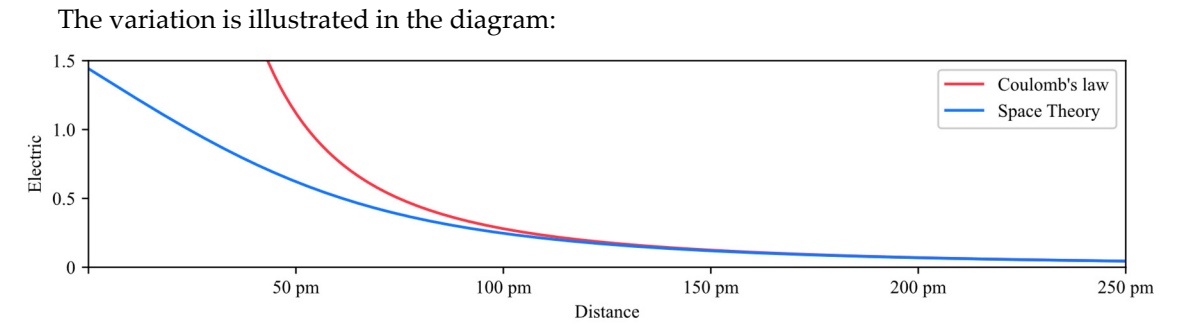
Figure 11. The electric field of a Hydrogen atom.
