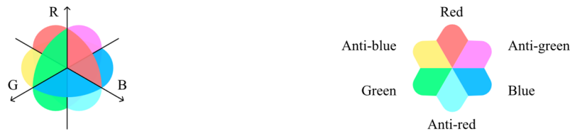
Figure 6. Quark color.
