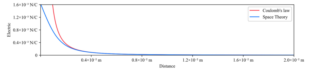
Figure 10. The electric field of an electron.
